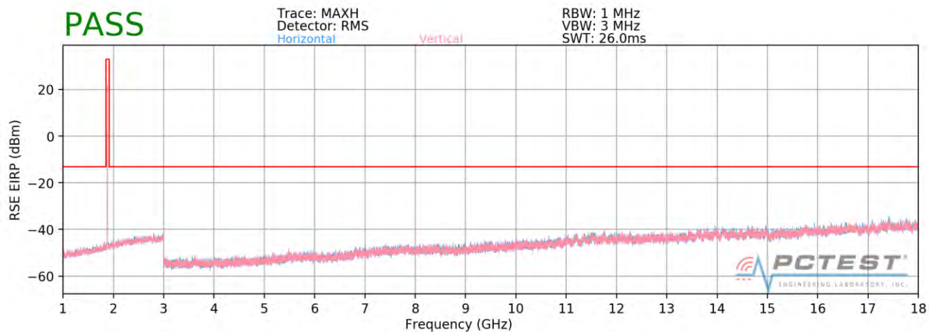
Plot 7-106. Radiated Spurious Plot above 1GHz (PCS CDMA)
