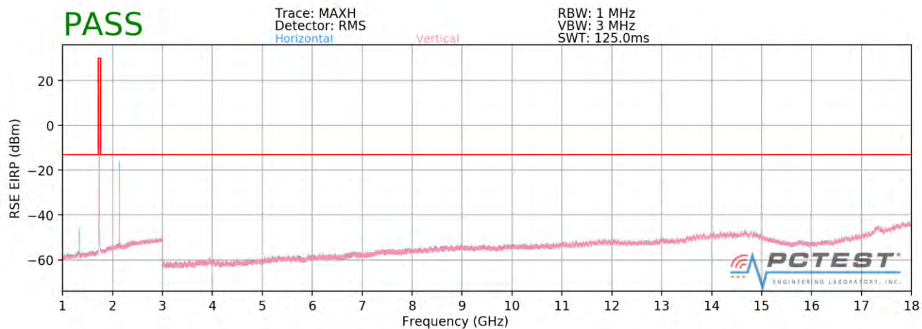
Plot 7-104. Radiated Spurious Plot above 1GHz (AWS WCDMA)
