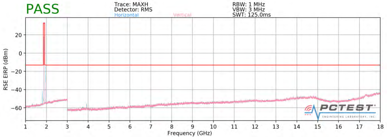
Plot 7-107. Radiated Spurious Plot above 1GHz (PCS WCDMA)
