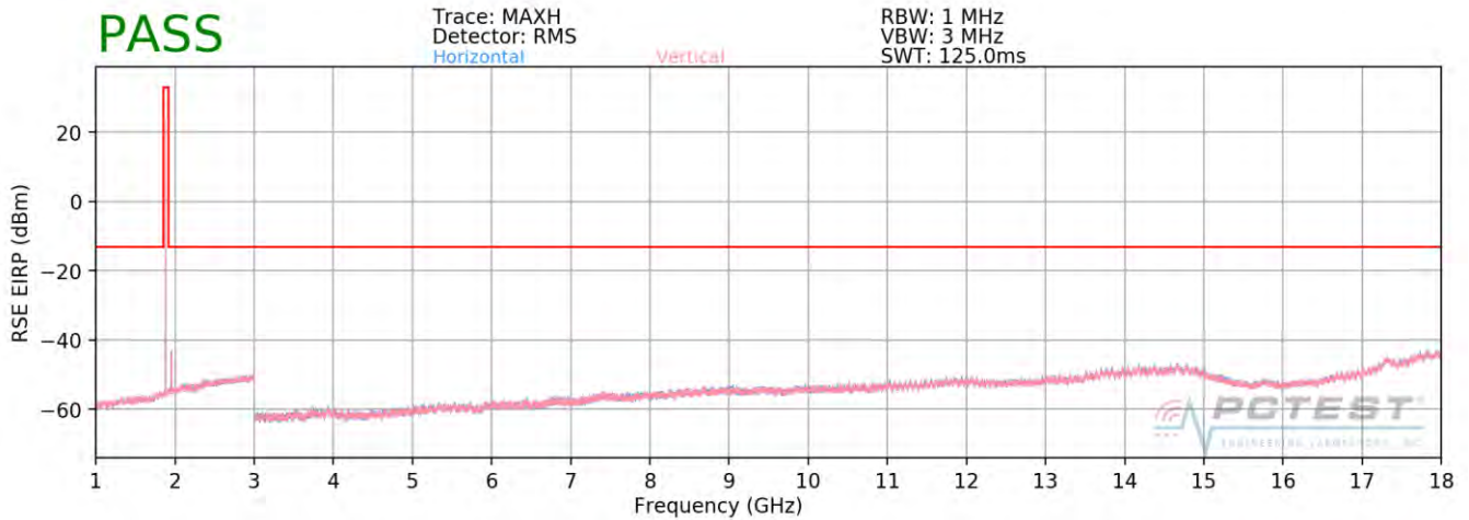
Plot 7-105. Radiated Spurious Plot above 1GHz (PCS GPRS)
