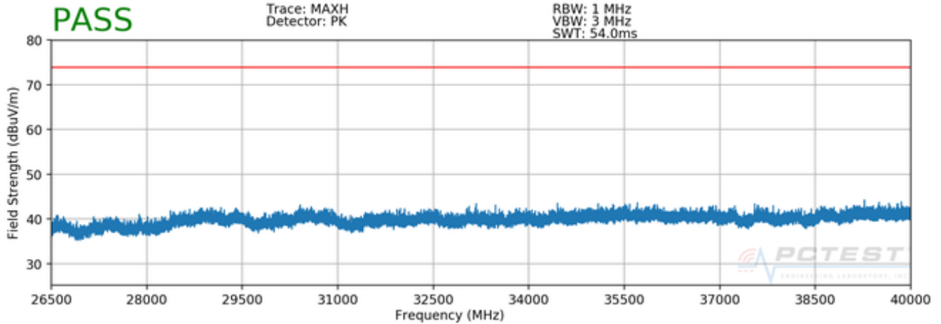
Plot 7-84. Radiated Spurious Plot 26.5GHz - 40GHz (802.11a)
