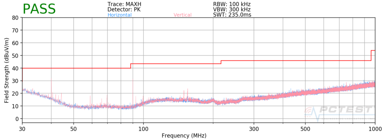
Plot 7-43. Radiated Spurious Plot below 1GHz
