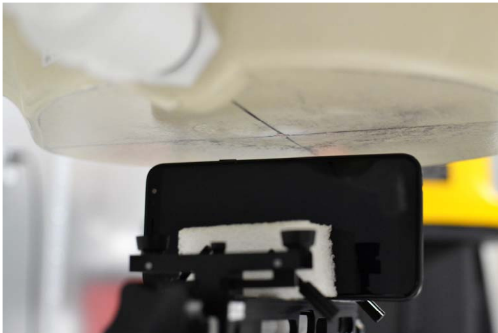
SAR Test Setup Photo 11: Right at 1.0 cm
