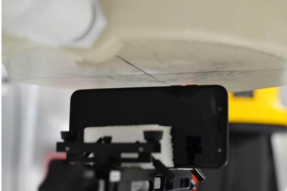
SAR Test Setup Photo 12: Left at 1.0 cm
