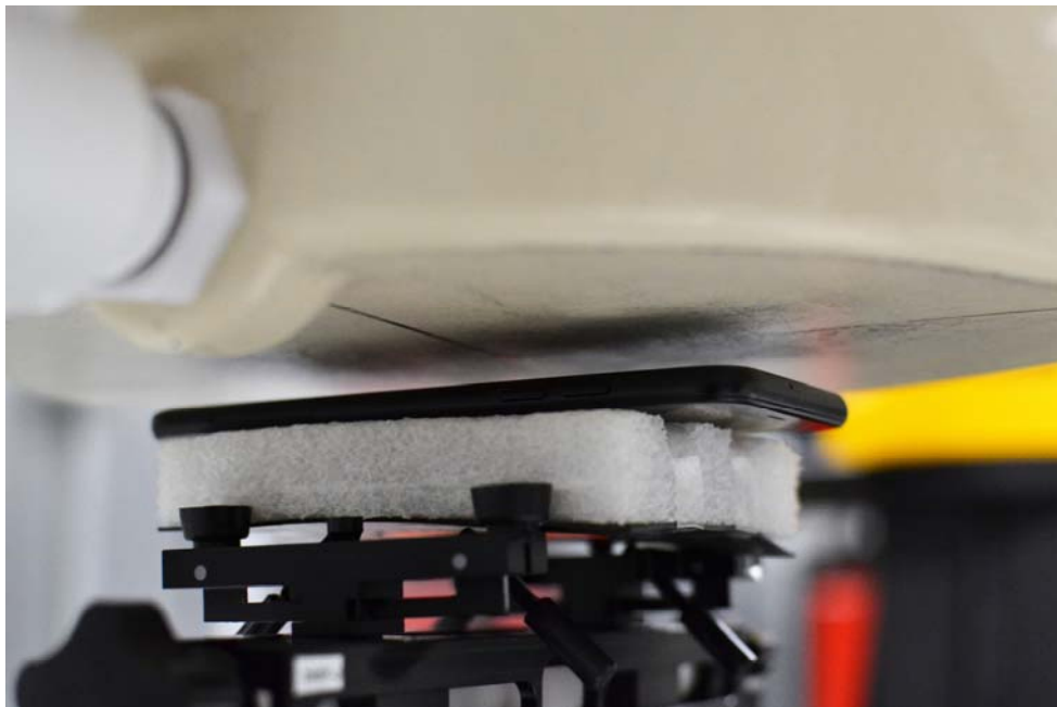
SAR Test Setup Photo 7: Back at 1.0 cm
