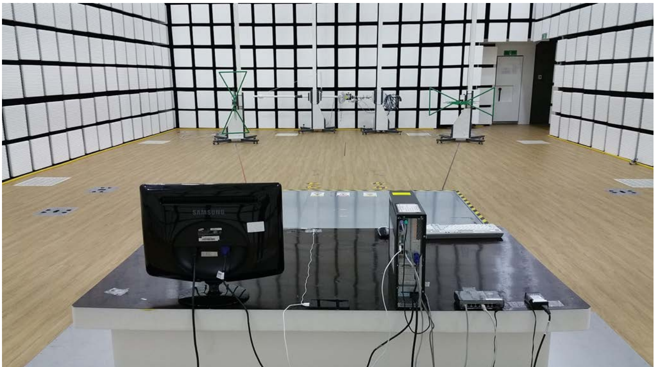
[ Radiated Disturbance for Below 1 GHz – Rear ]
