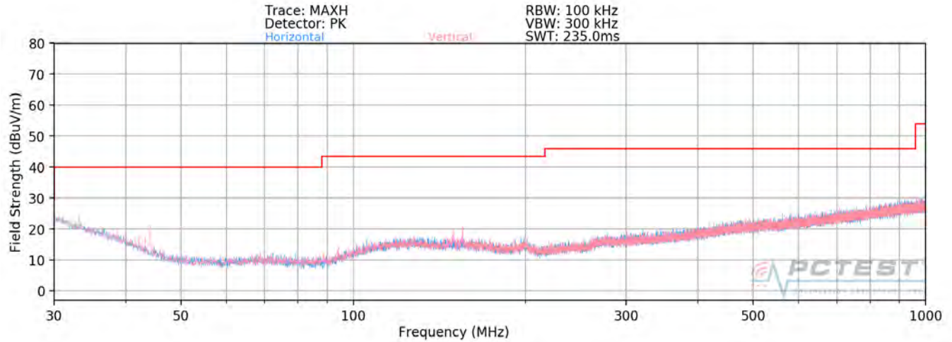
Plot 7-105. Radiated Spurious Plot below 1GHz (802.11a – U3 Ch. 157)
