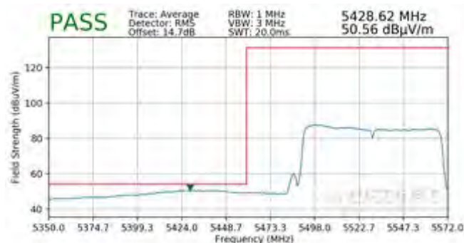
Plot 7-102. Radiated Lower Band Edge Plot (Average – UNII Band 2C)
