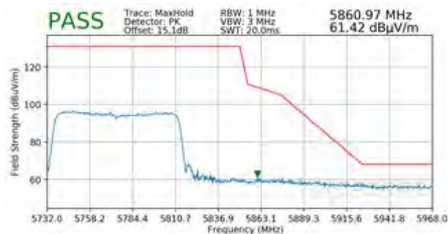
Plot 7-104. Radiated Upper Band Edge Plot (Peak – UNII Band 3)
