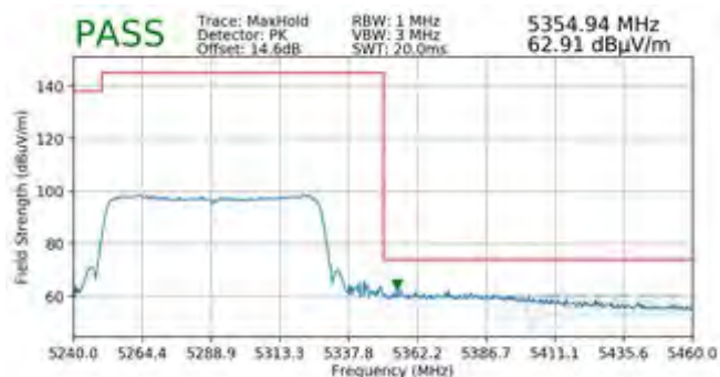
Plot 7-101. Radiated Upper Band Edge Plot (Peak – UNII Band 2A)
