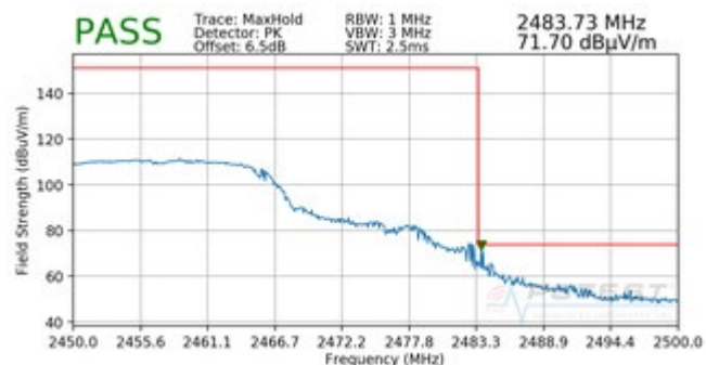
Plot 7-40. Radiated Restricted Upper Band Edge Measurement (Peak)
