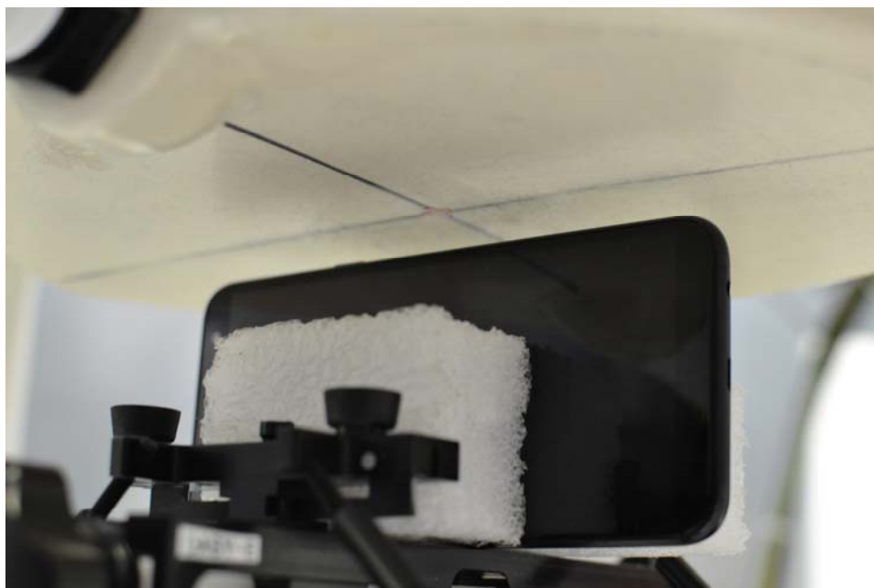
SAR Test Setup Photo 11 - Right Side at 10 mm
