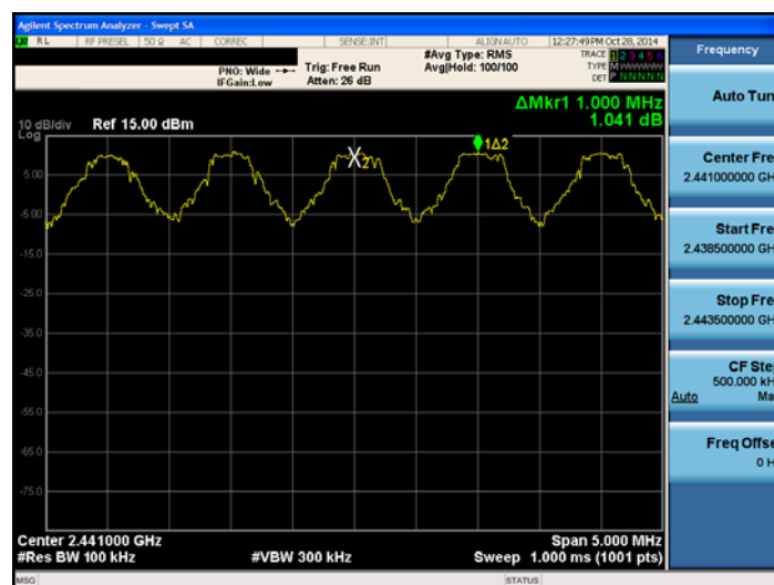
Plot 6-32. Channel Spacing Plot (Bluetooth)
