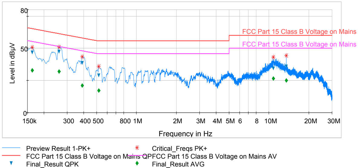
Plot 6-43. Line-Conducted Test Plot (L1)
