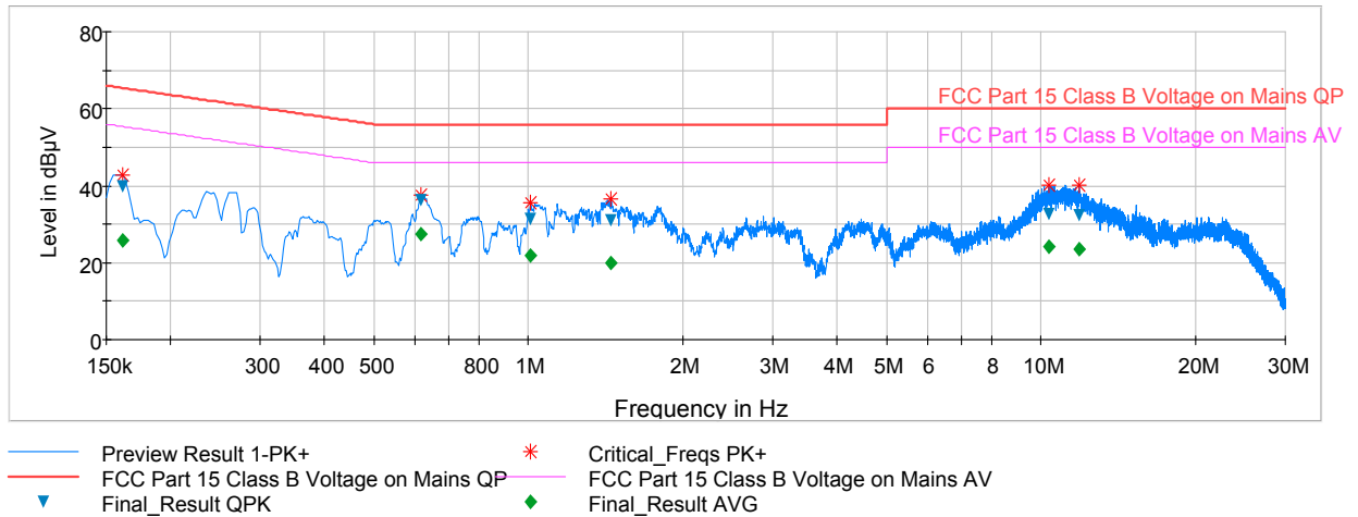
Plot 6-44. Line-Conducted Test Plot (N)
