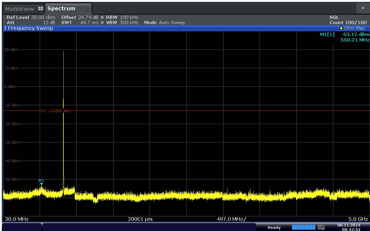
Plot 6-13. Conducted Spurious Plot (Band 5–1.4MHz–QPSK–RB Size 3–RB Offset 3– Ch.20643)
