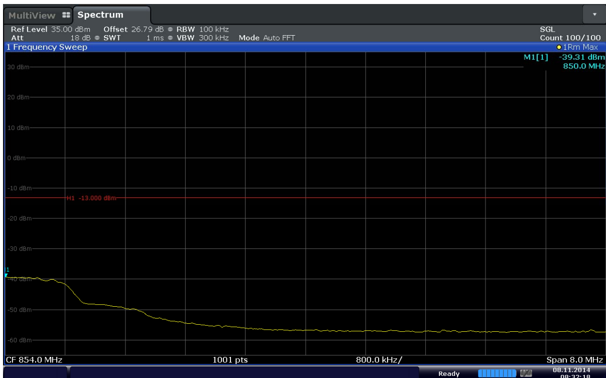
Plot 6-36. Upper Extended Band Edge Plot (Band 5 – 1.4MHz – QPSK – RB Size 6)
