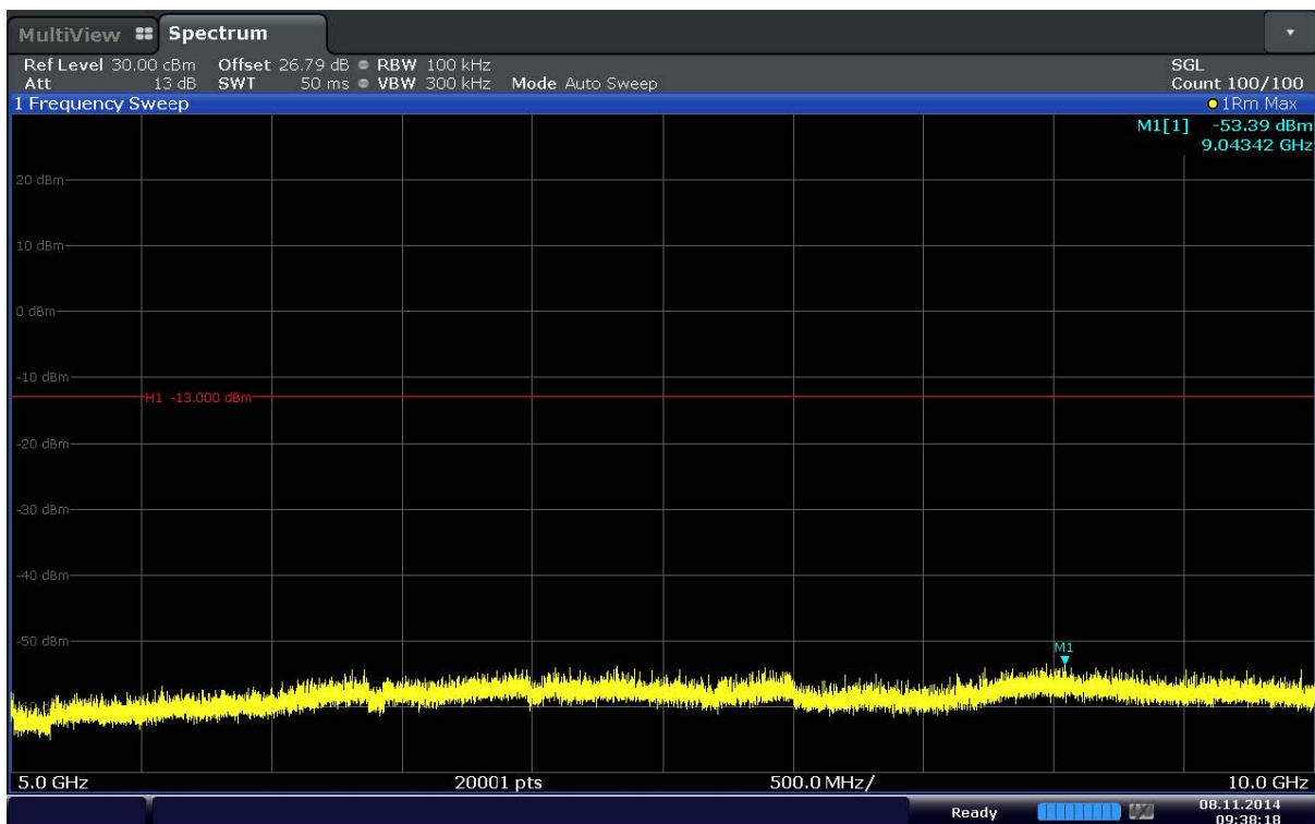
Plot 6-31. Conducted Spurious Plot (Band 5–10.0MHz–QPSK–RB Size 1–RB Offset 49– Ch.20600)
