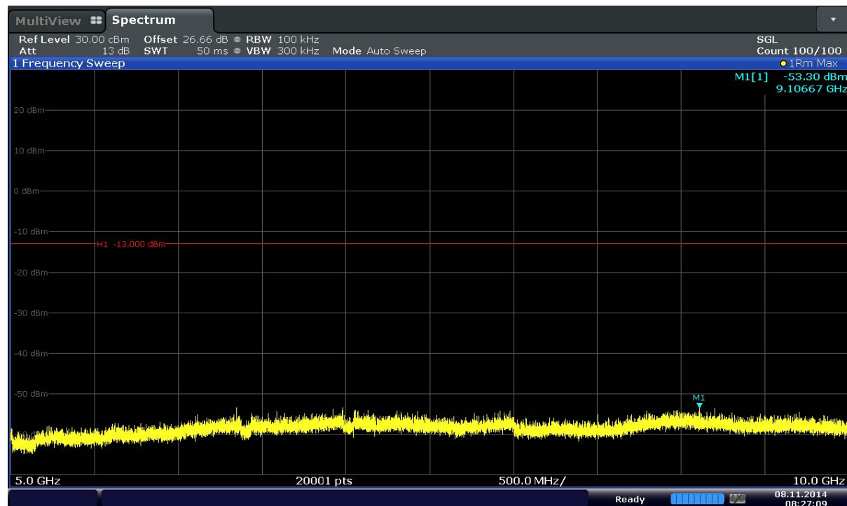
Plot 6-10. Conducted Spurious Plot (Band 5–1.4MHz–QPSK–RB Size 3–RB Offset 0– Ch.20407)
