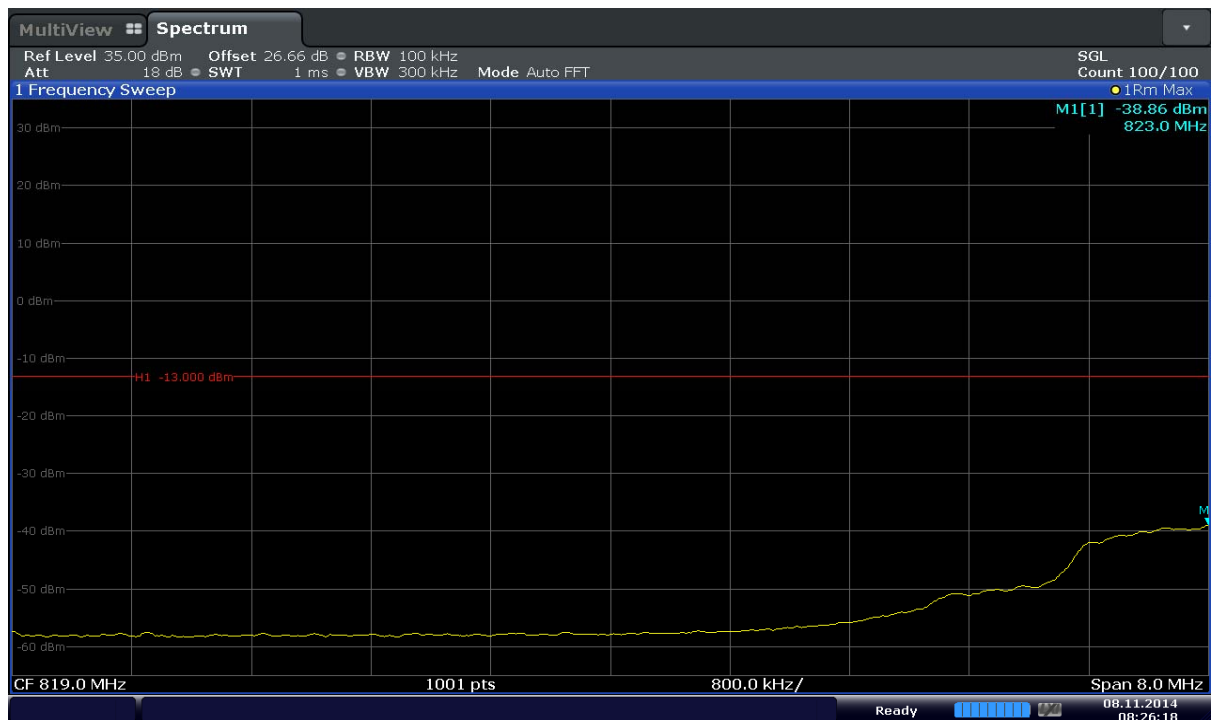
Plot 6-34. Lower Extended Band Edge Plot (Band5 – 1.4MHz – QPSK – RB Size 6)
