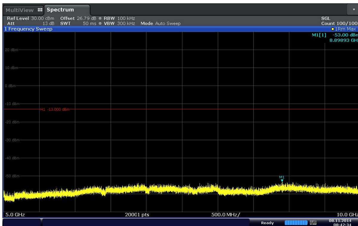
Plot 6-19. Conducted Spurious Plot (Band 5–3.0MHz–QPSK–RB Size 1–RB Offset 7– Ch.20635)
