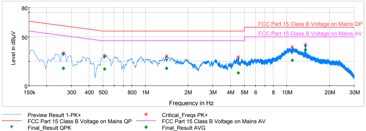
Plot 8-1. Line-Conducted Test Plot (L1)
