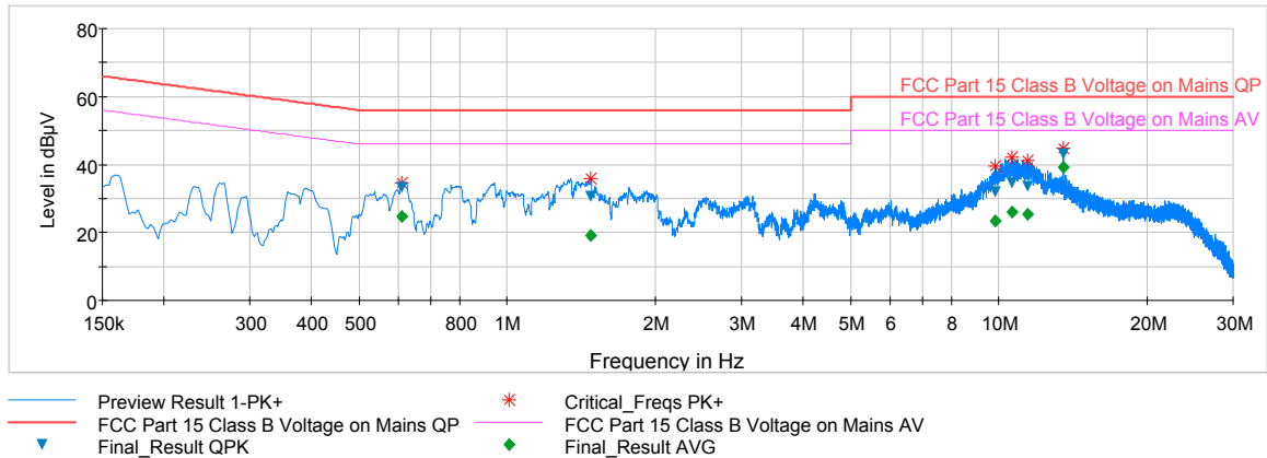
Plot 8-2. Line-Conducted Test Plot (N)
