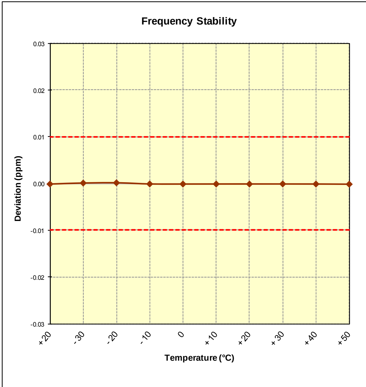
Figure 8-3. Frequency Stability Plot
