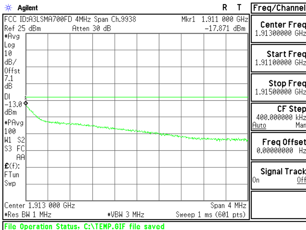
Plot 6-46. 4MHz Span Plot (PCS WCDMA Mode - Ch.9538(DL9938))
