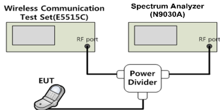
Figure 6-2. Test Instruments & Measurement Setup
