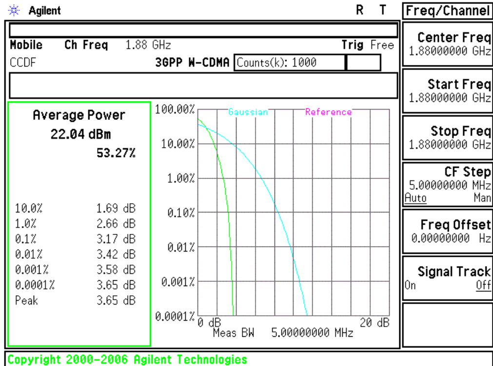
Plot 6-49. Peak-Average Ratio Plot (PCS WCDMA Mode - Ch.9400(DL9800))
