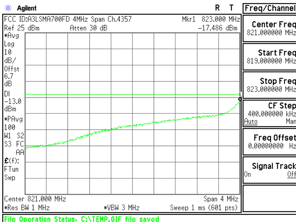
Plot 6-40. 4MHz Span Plot (Cellular WCDMA Mode - Ch.4132(DL4357))
