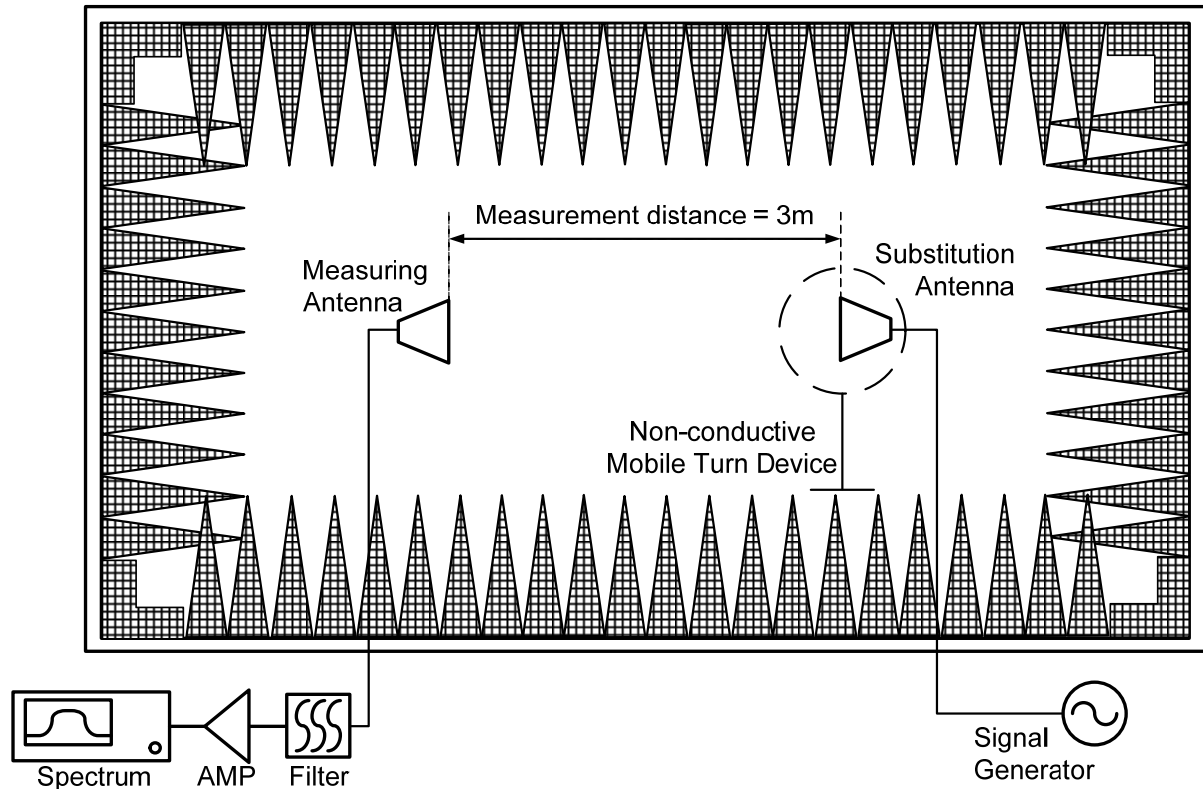
Figure 6-8. Test Instruments & Measurement Setup
