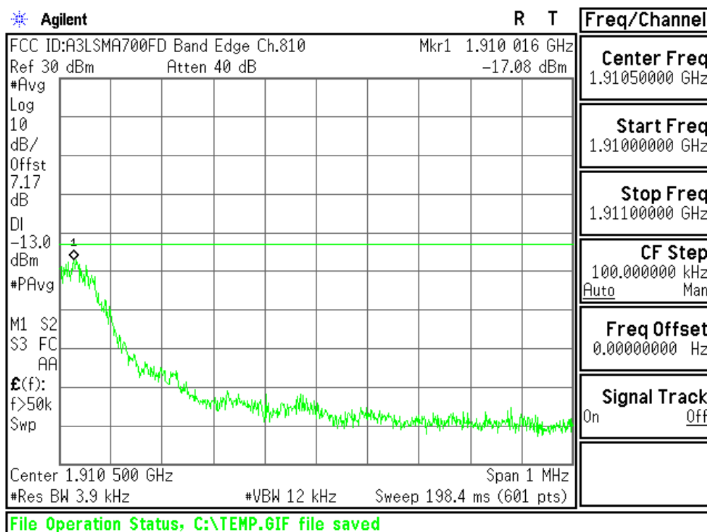
Plot 6-38. Band Edge Plot (PCS GSM Mode – Ch.810)
