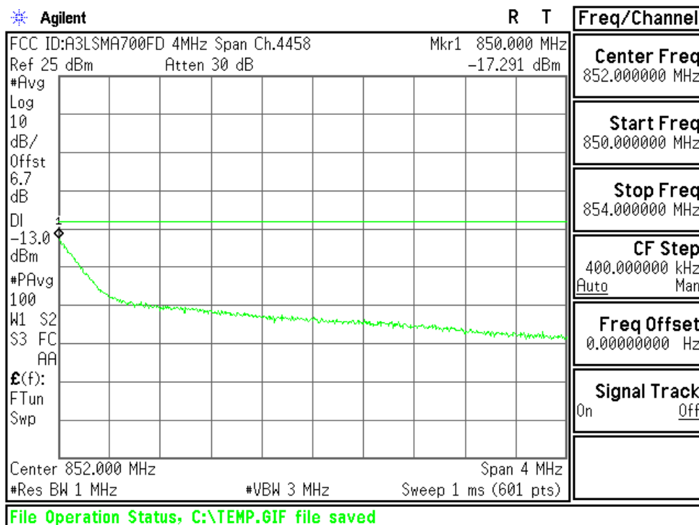
Plot 6-42. 4MHz Span Plot (Cellular WCDMA Mode - Ch.4233(DL4458))
