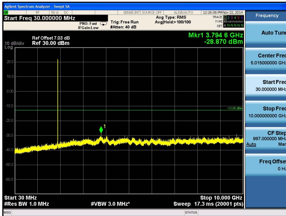
Plot 6-29. Conducted Spurious Plot (PCS WCDMA Mode - Ch.9538(DL9938))
