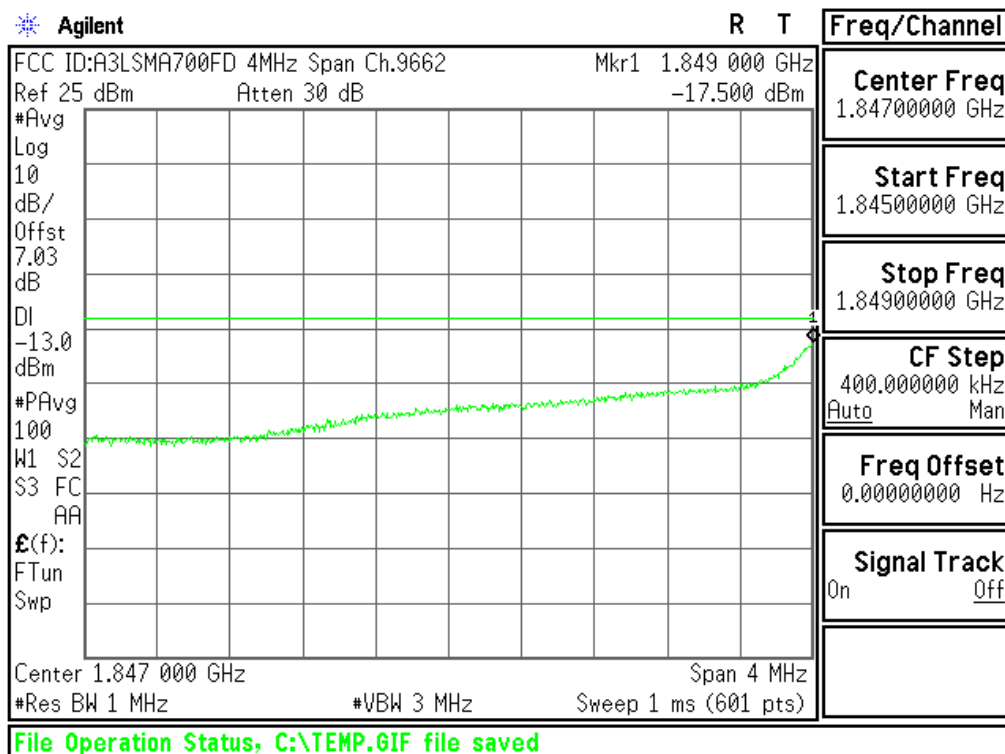
Plot 6-44. 4MHz Span Plot (PCS WCDMA Mode - Ch.9262(DL9662))
