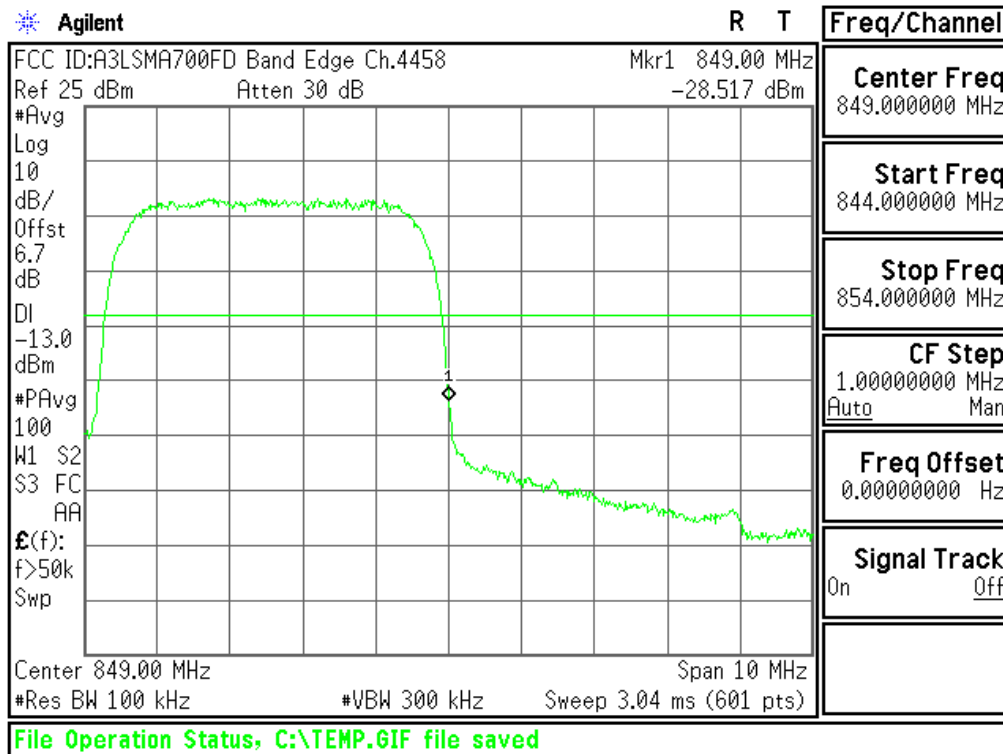
Plot 6-41. Band Edge Plot (Cellular WCDMA Mode - Ch.4233(DL4458))
