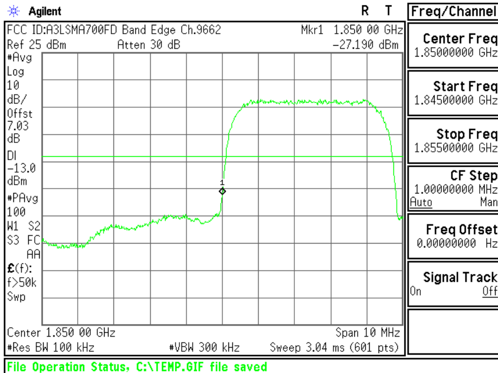
Plot 6-43. Band Edge Plot (PCS WCDMA Mode - Ch.9262(DL9662))
