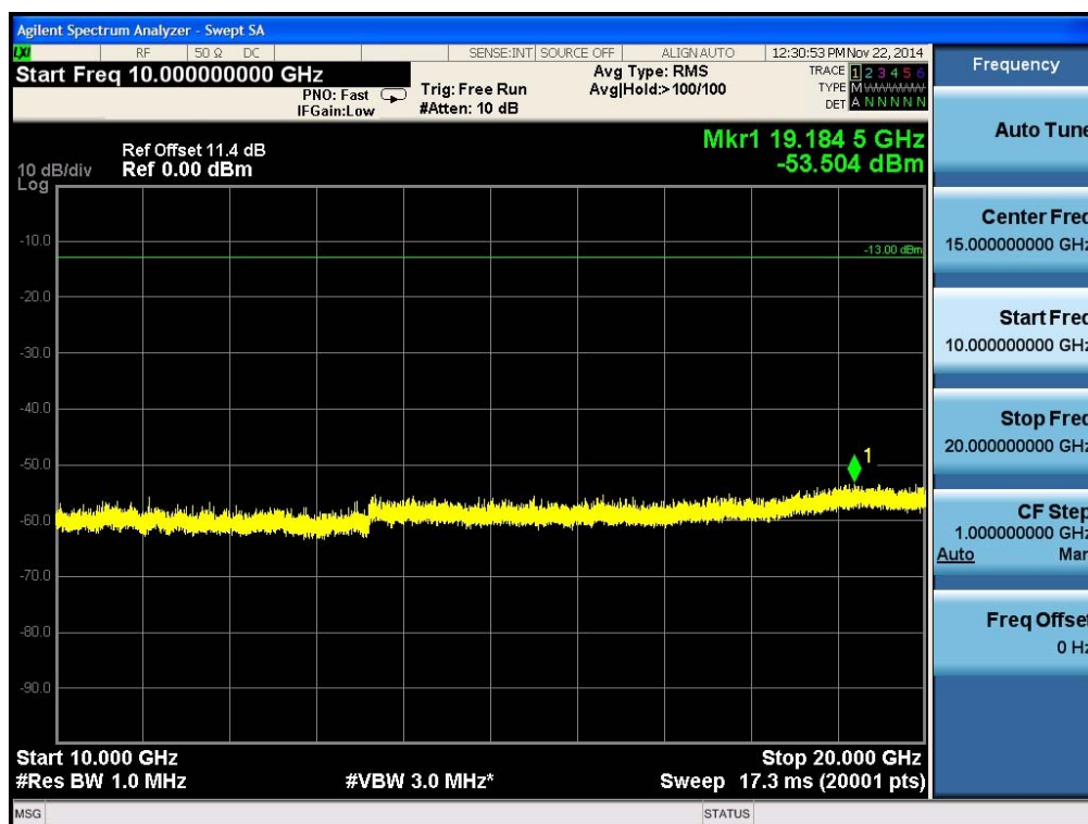
Plot 6-26. Conducted Spurious Plot (PCS WCDMA Mode - Ch.9262(DL9662))
