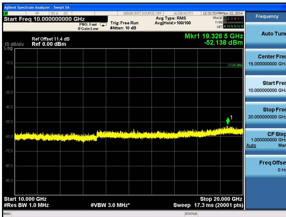
Plot 6-28. Conducted Spurious Plot (PCS WCDMA Mode - Ch.9400(DL9800))
