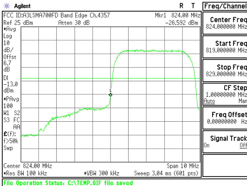
Plot 6-39. Band Edge Plot (Cellular WCDMA Mode - Ch.4132(DL4357))
