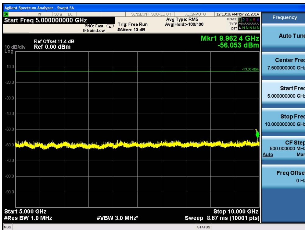
Plot 6-24. Conducted Spurious Plot (Cellular WCDMA Mode - Ch.4233(DL4458))
