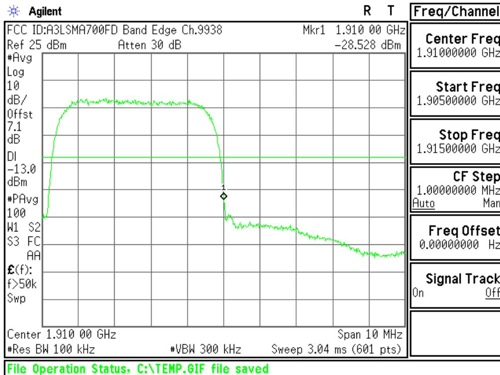
Plot 6-45. Band Edge Plot (PCS WCDMA Mode - Ch.9538(DL9938))
