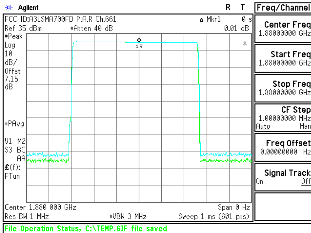
Plot 6-47. Peak-Average Ratio Plot (PCS GSM Mode - Ch.661)
