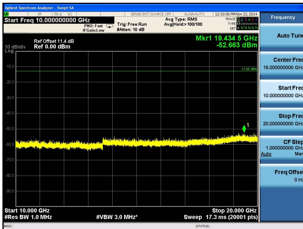
Plot 6-30. Conducted Spurious Plot (PCS WCDMA Mode - Ch.9538(DL9938))
