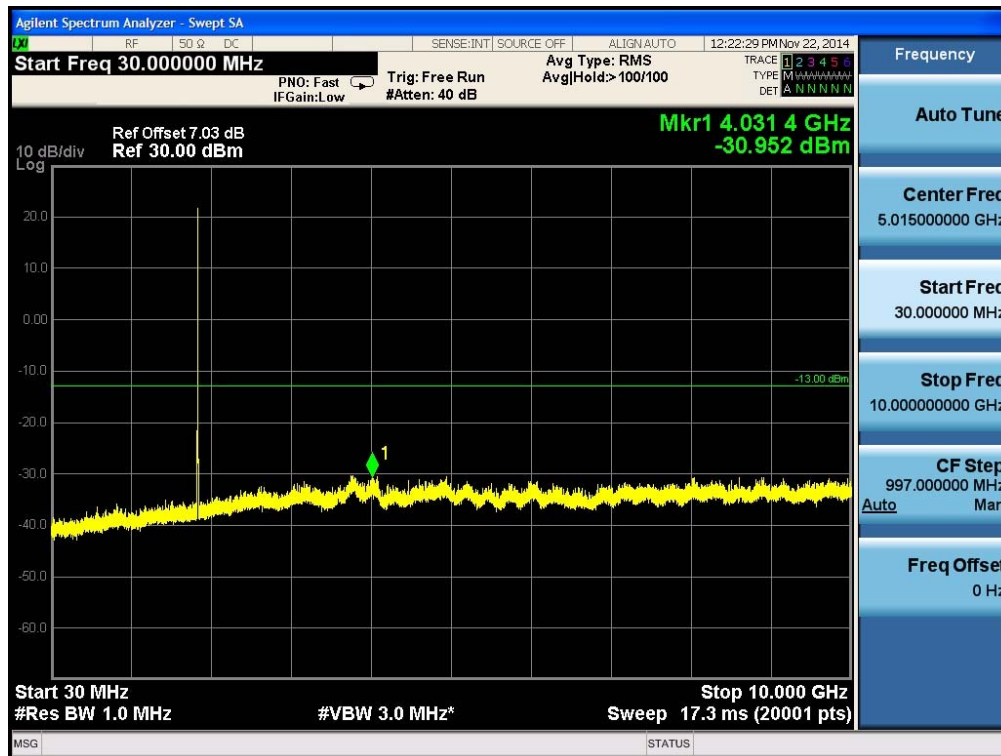
Plot 6-25. Conducted Spurious Plot (PCS WCDMA Mode - Ch.9262(DL9662))
