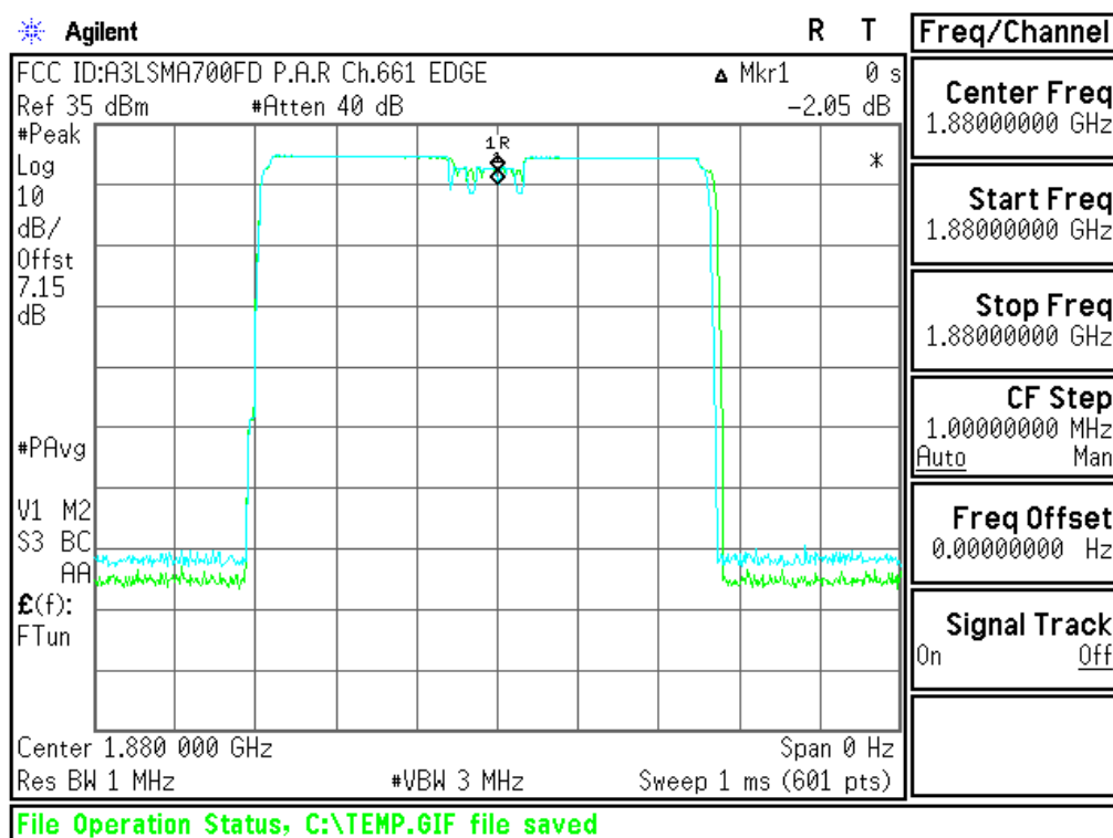
Plot 6-48. Peak-Average Ratio Plot (EDGE1900 Mode - Ch.661)
