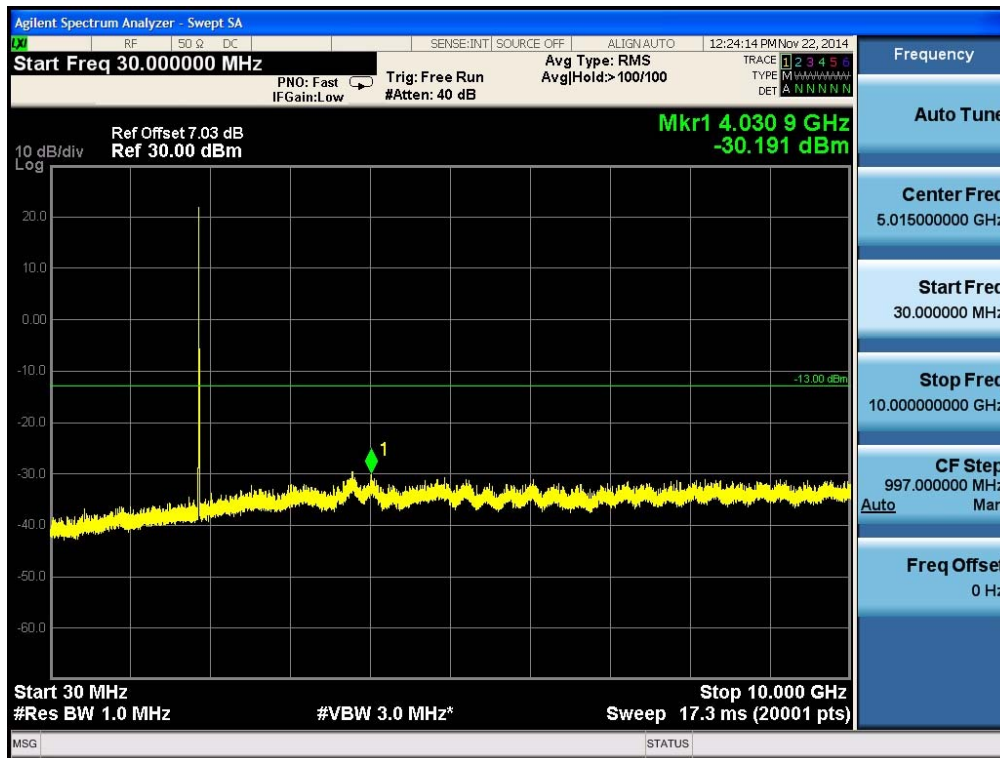
Plot 6-27. Conducted Spurious Plot (PCS WCDMA Mode - Ch.9400(DL9800))
