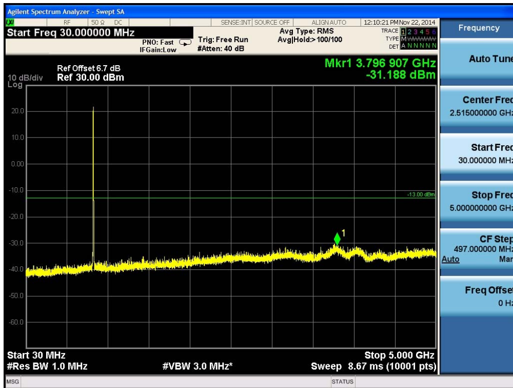
Plot 6-23. Conducted Spurious Plot (Cellular WCDMA Mode - Ch.4233(DL4458))
