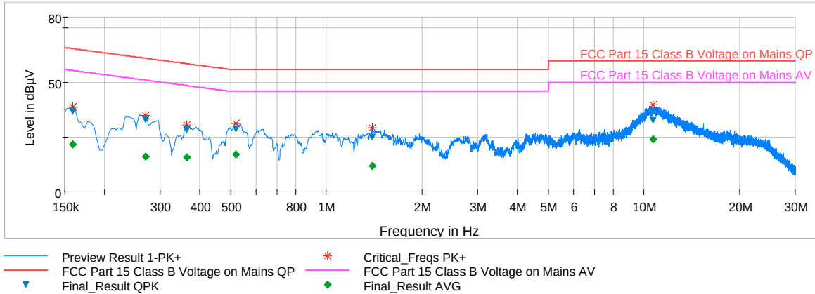
Plot 6-68. Line Conducted Plot with 802.11a UNII Band 2A (L1)
