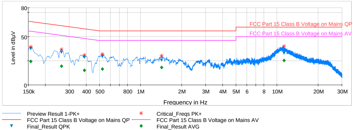
Plot 6-66. Line Conducted Plot with 802.11a UNII Band 1 (L1)
