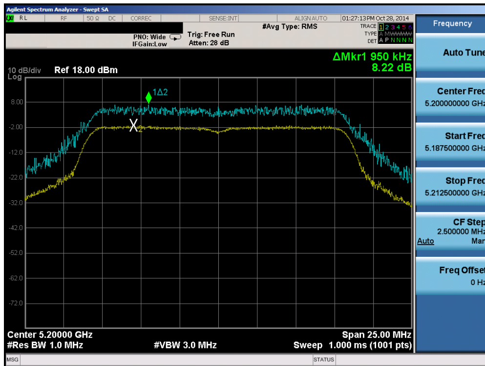
Plot 6-56. Peak Excursion Ratio Plot (802.11a (UNII Band 1) – Ch. 40)
