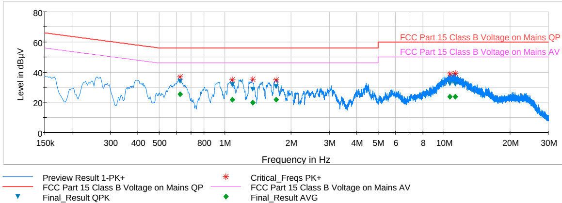
Plot 6-69. Line Conducted Plot with 802.11a UNII Band 2A (N)
