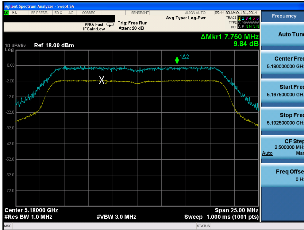
Plot 6-57. Peak Excursion Ratio Plot (20MHz BW 802.11n (UNII Band 1) – Ch. 36)
