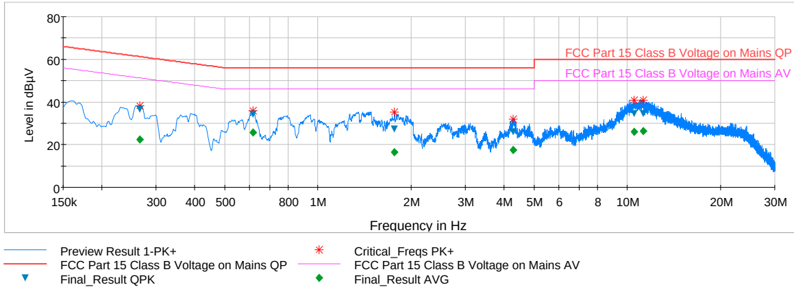
Plot 6-67. Line Conducted Plot with 802.11a UNII Band 1 (N)
