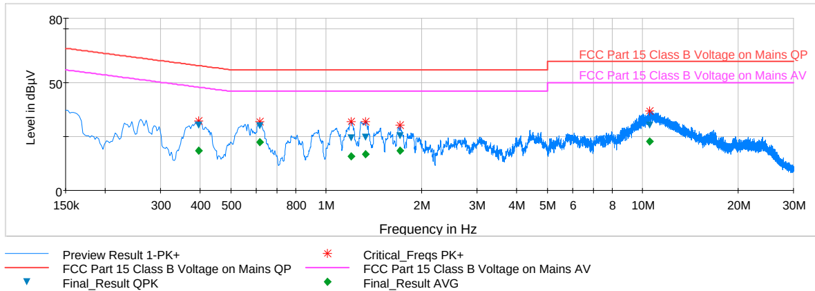
Plot 6-70. Line Conducted Plot with 802.11a UNII Band 2C (L1)
