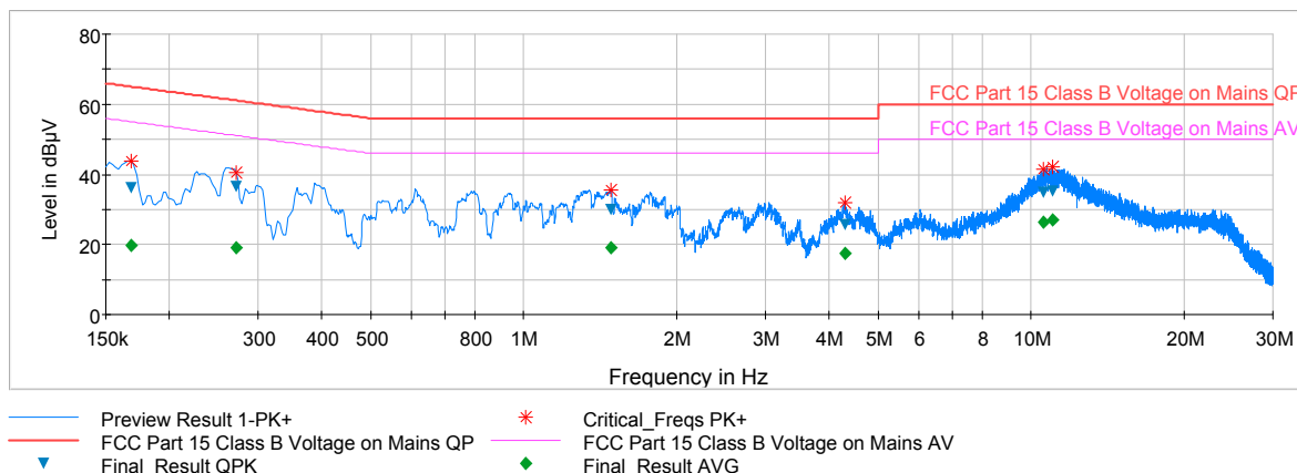
Plot 6-62. Line Conducted Plot with 802.11b (N)
