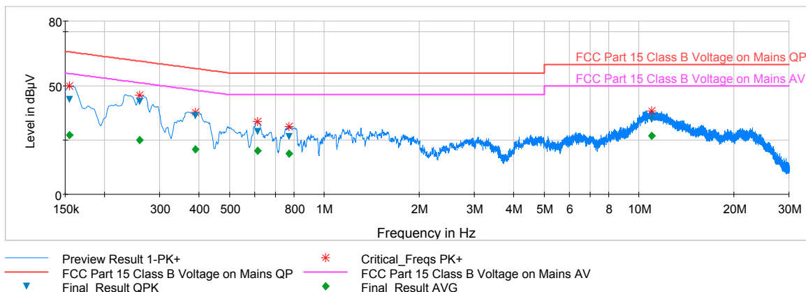
Plot 6-61. Line Conducted Plot with 802.11b (L1)
