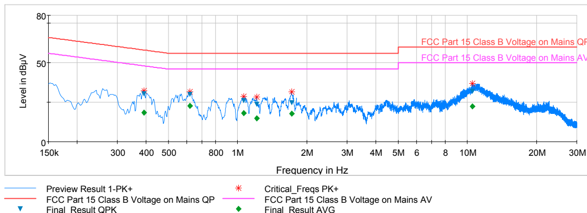
Plot 6-63. Line Conducted Plot with 802.11a (L1)
