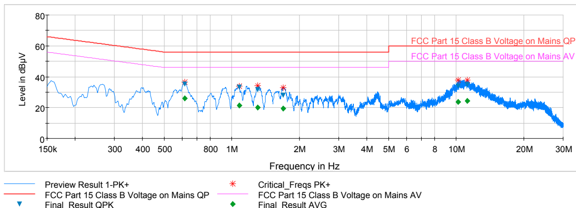
Plot 6-64. Line Conducted Plot with 802.11a (N)
