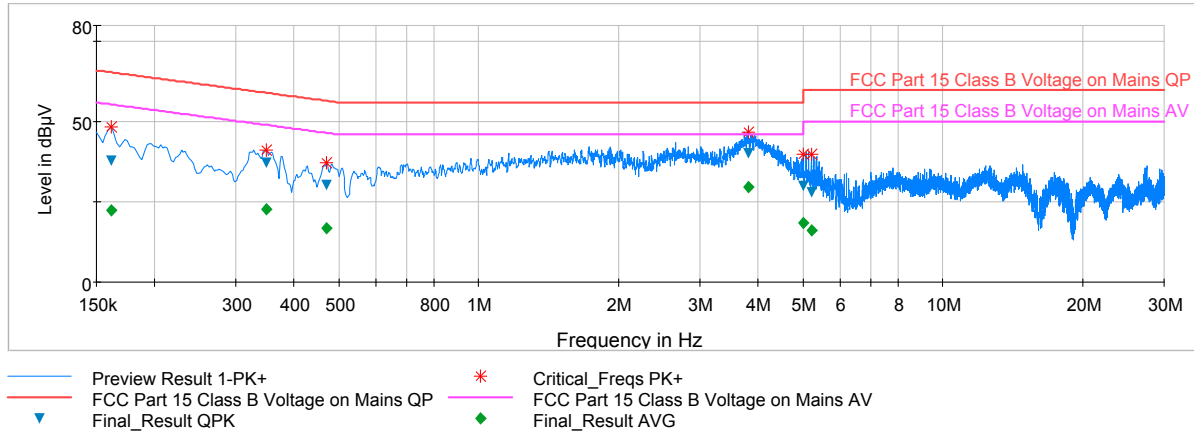
Plot 6-6. Line-Conducted Test Plot (L1)
