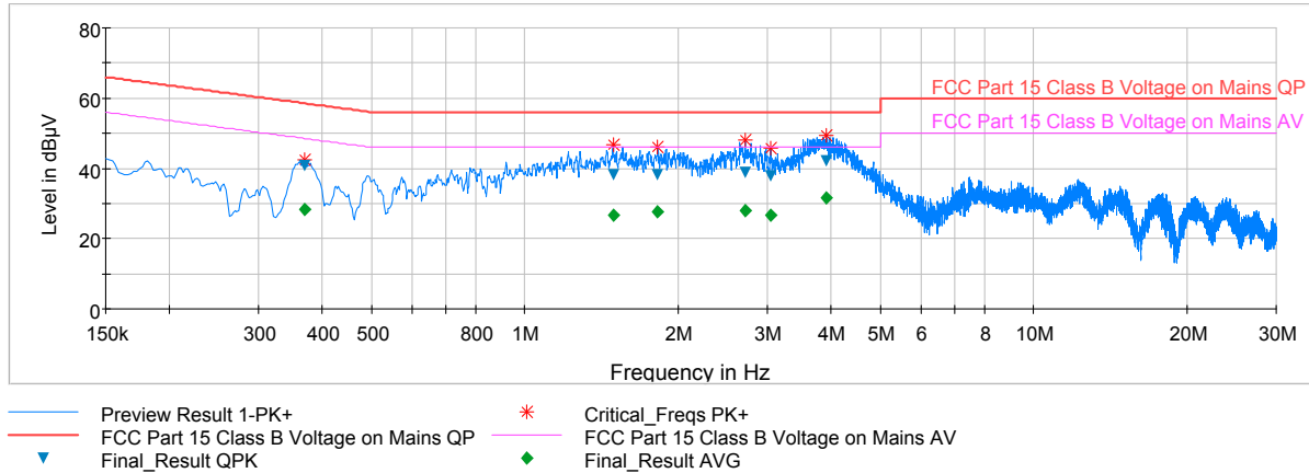
Plot 6-7. Line-Conducted Test Plot (N)
