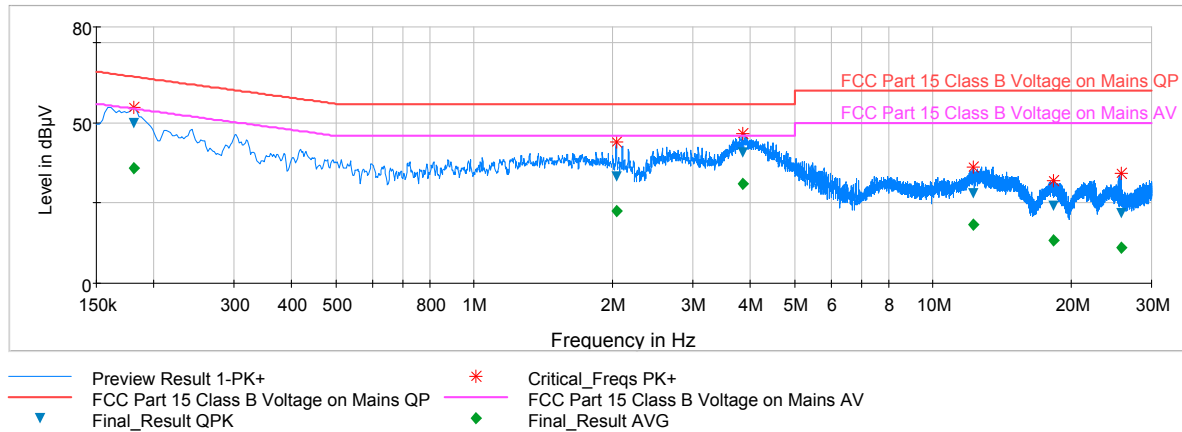
Plot 6-44. Line-Conducted Test Plot (L1)
