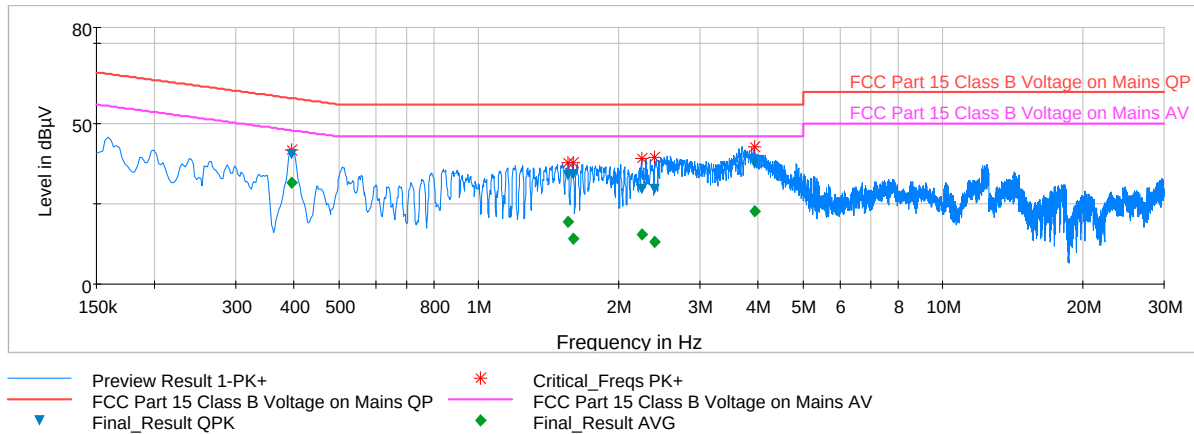
Plot 6-77. Line Conducted Plot with 802.11a UNII Band 2C (L1)
