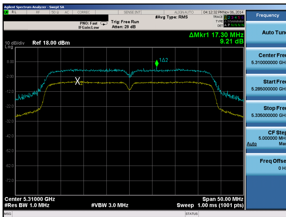
Plot 6-56. Peak Excursion Ratio Plot (40MHz BW 802.11n (UNII Band 2A) – Ch. 62)
