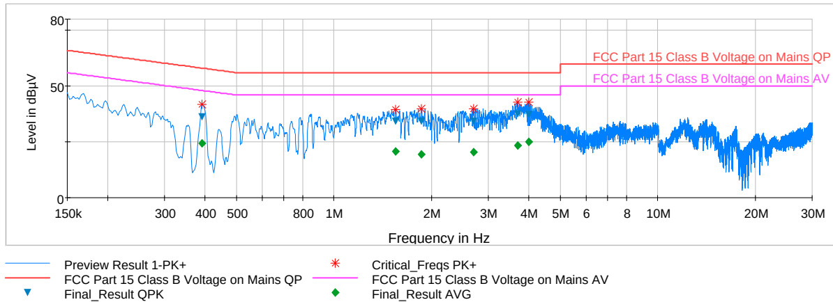
Plot 6-75. Line Conducted Plot with 802.11a UNII Band 2A (L1)
