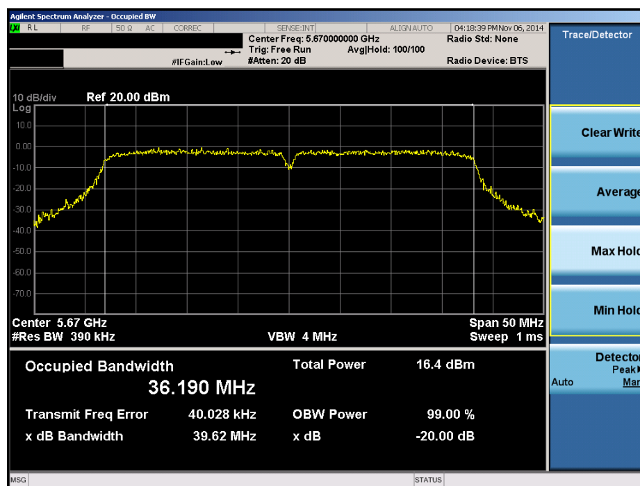
Plot 6-30. 20dB Bandwidth Plot (40MHz BW 802.11n (UNII Band 2C) – Ch. 134)
