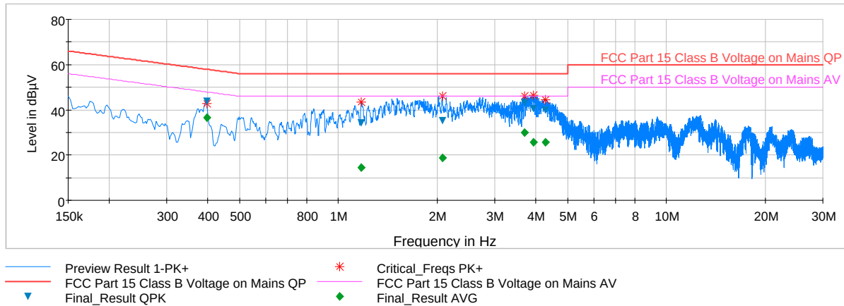
Plot 6-76. Line Conducted Plot with 802.11a UNII Band 2A (N)
