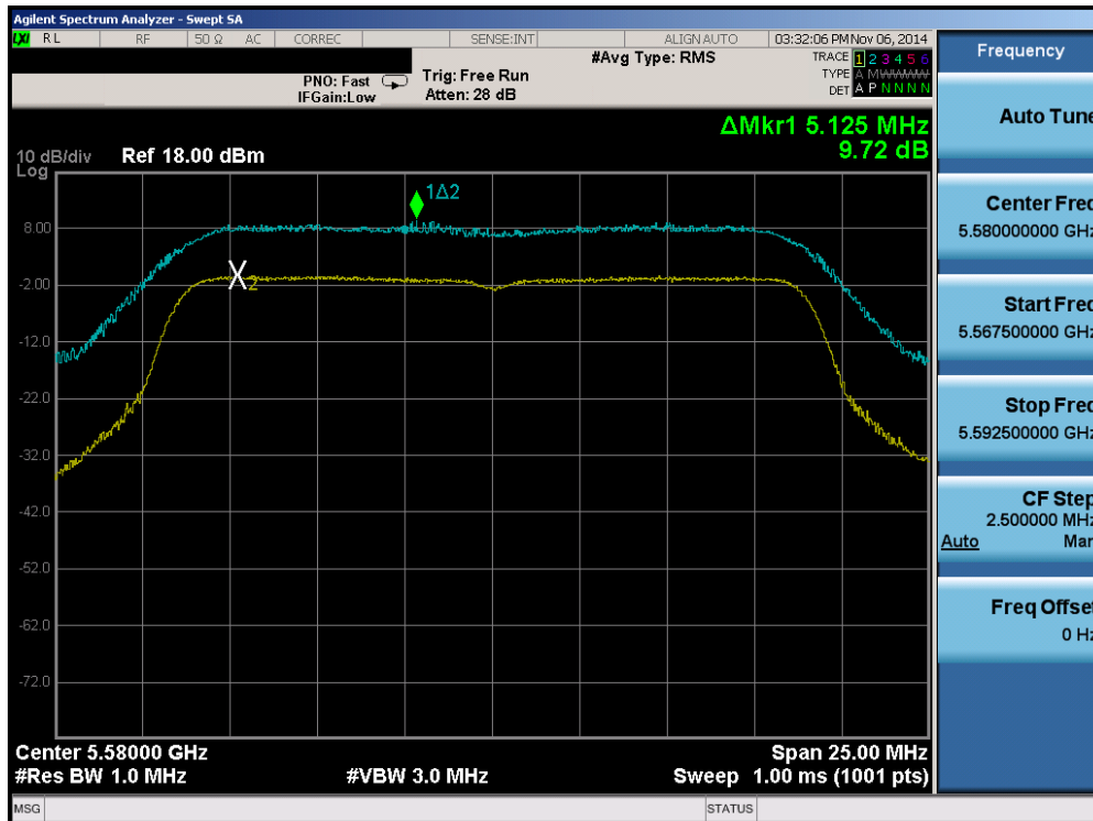
Plot 6-58. Peak Excursion Ratio Plot (20MHz BW 802.11n (UNII Band 2C) – Ch. 116)
