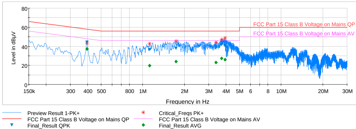
Plot 6-74. Line Conducted Plot with 802.11a UNII Band 1 (N)
