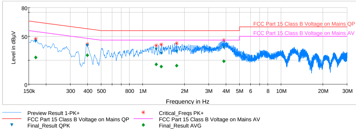
Plot 6-73. Line Conducted Plot with 802.11a UNII Band 1 (L1)
