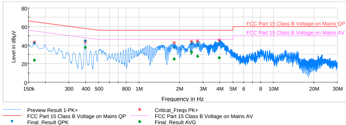
Plot 6-78. Line Conducted Plot with 802.11a UNII Band 2C (N)
