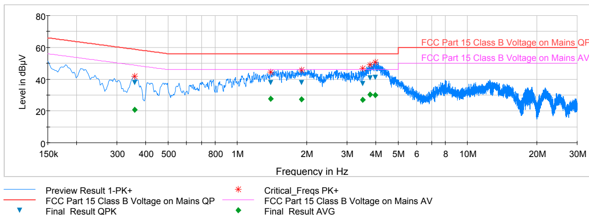
Plot 6-64. Line Conducted Plot with 802.11b (N)
