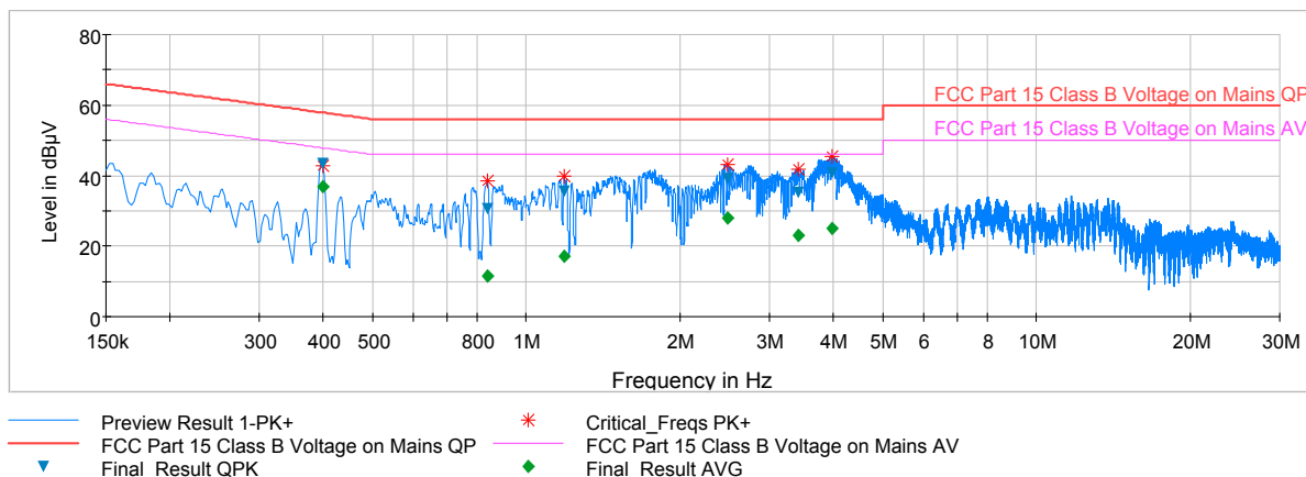
Plot 6-66. Line Conducted Plot with 802.11a (N)
