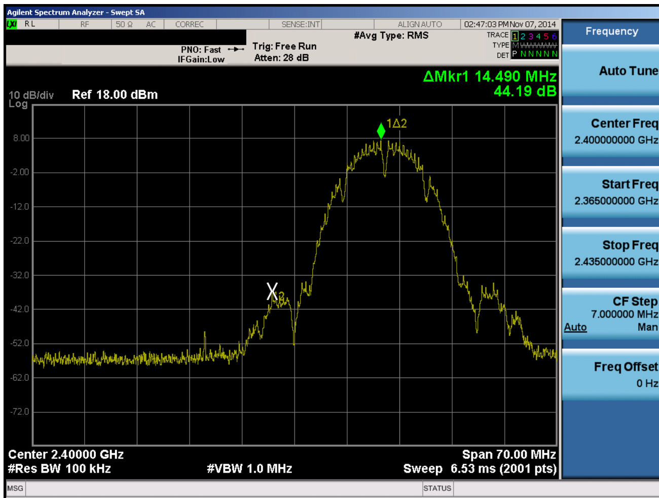
Plot 6-35. Band Edge Plot (802.11b – Ch. 1)
