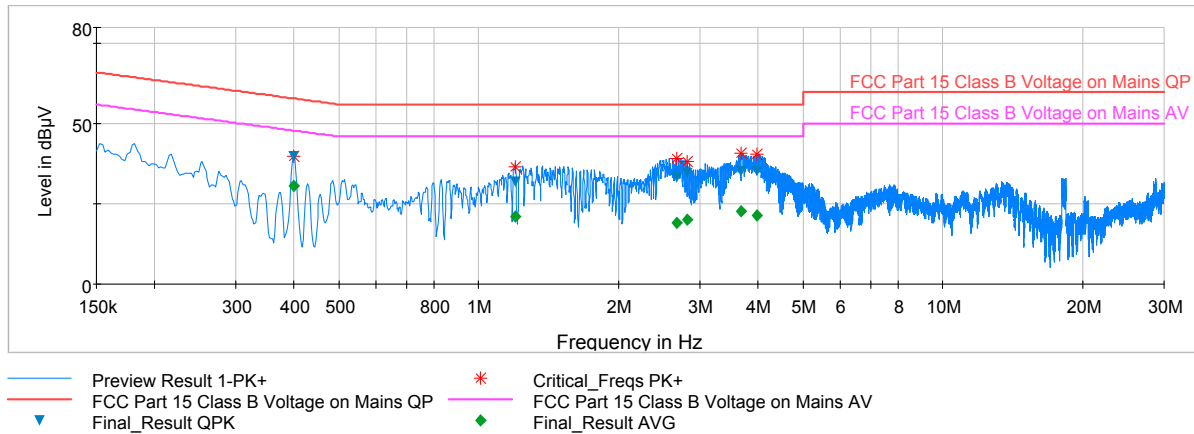
Plot 6-65. Line Conducted Plot with 802.11a (L1)
