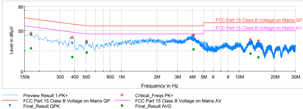
Plot 6-63. Line Conducted Plot with 802.11b (L1)
