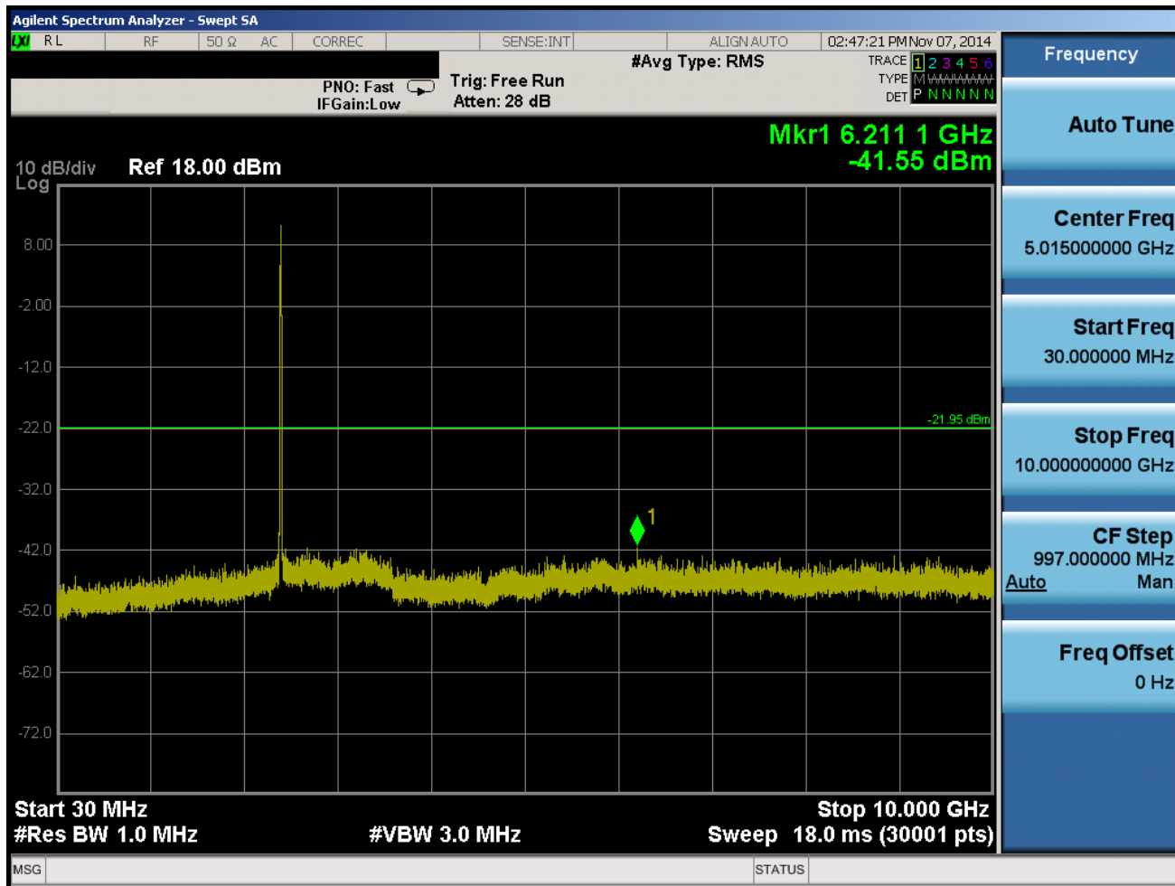
Plot 6-47. Conducted Spurious Plot (802.11b – Ch. 1)
