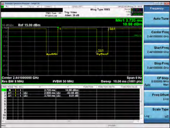
Figure 9-4 Bluetooth Transmission Plot
