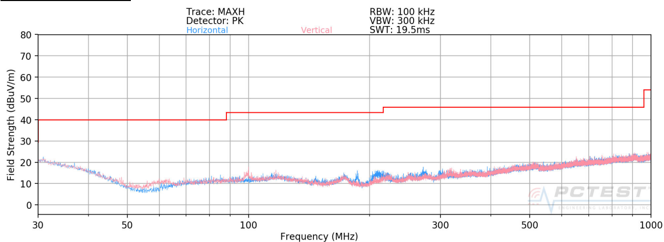
Plot 7-48. Radiated Spurious Plot below 1GHz
