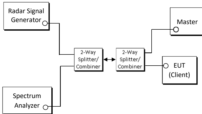
Figure 6-1. Test Setup
