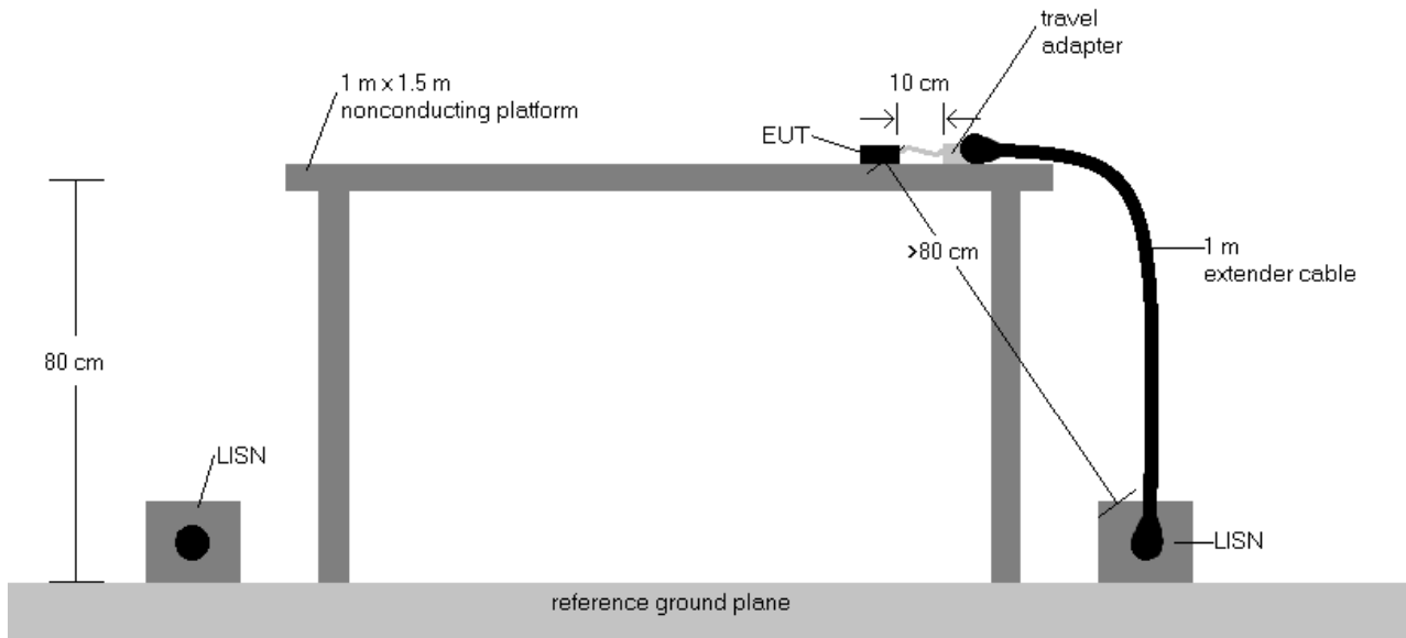
Figure 7-7. Test Instrument & Measurement Setup
