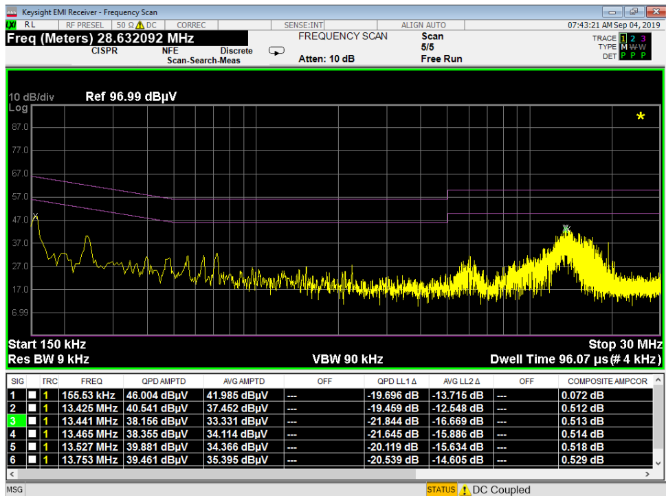
Plot 7-9. Line-Conducted Test Plot Terminated at 50 ohms (N)
