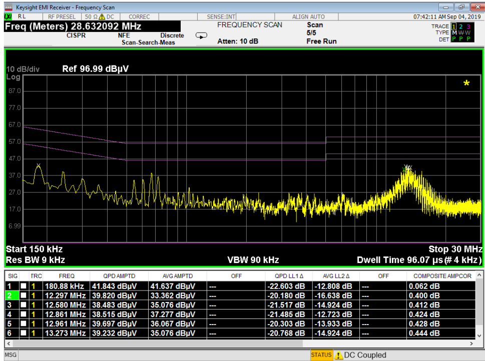
Plot 7-8. Line-Conducted Test Plot Terminated at 50 ohms (L1)
