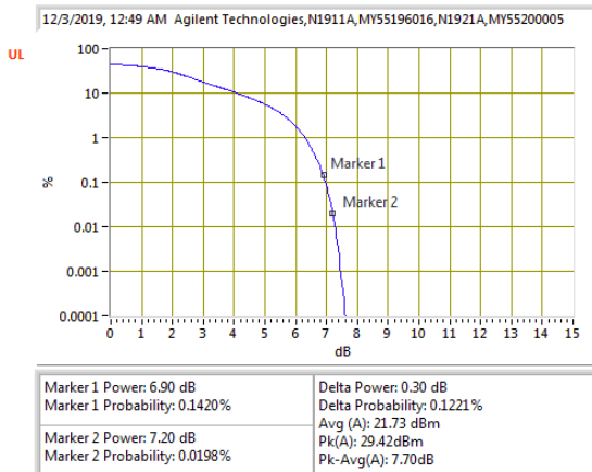
LTE B41 15MHz QPSK Middle Channel
