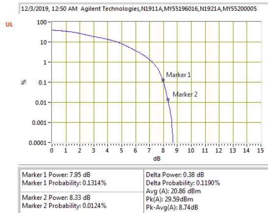
LTE B41 15MHz 16QAM Middle Channel
