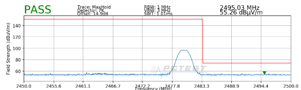
Plot 7-52. Radiated Restricted Upper Band Edge Measurement (Peak)
