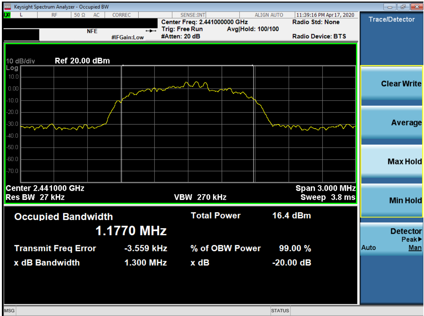
Plot 7-8. 20dB Bandwidth Plot (Bluetooth, 3Mbps – Ch. 39)
