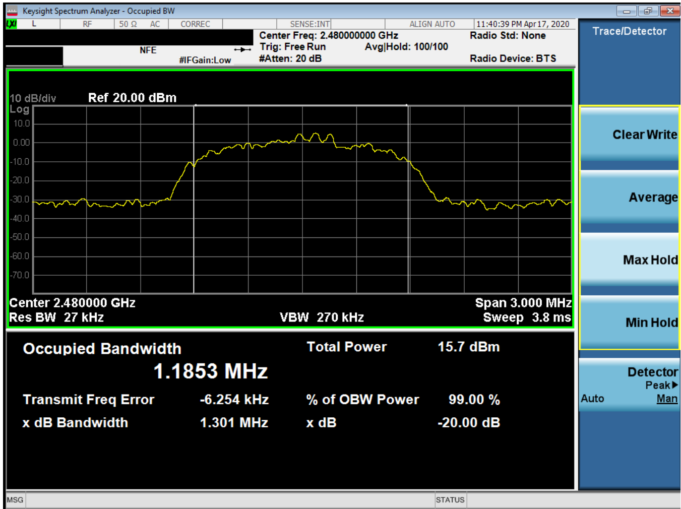
Plot 7-9. 20dB Bandwidth Plot (Bluetooth, 3Mbps – Ch. 78)
