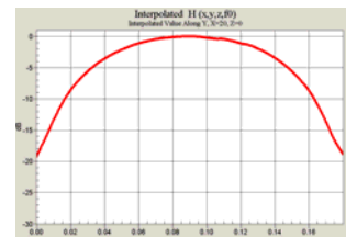
Figure 6-5 2-D Interpolated points from scan along dipole axis
