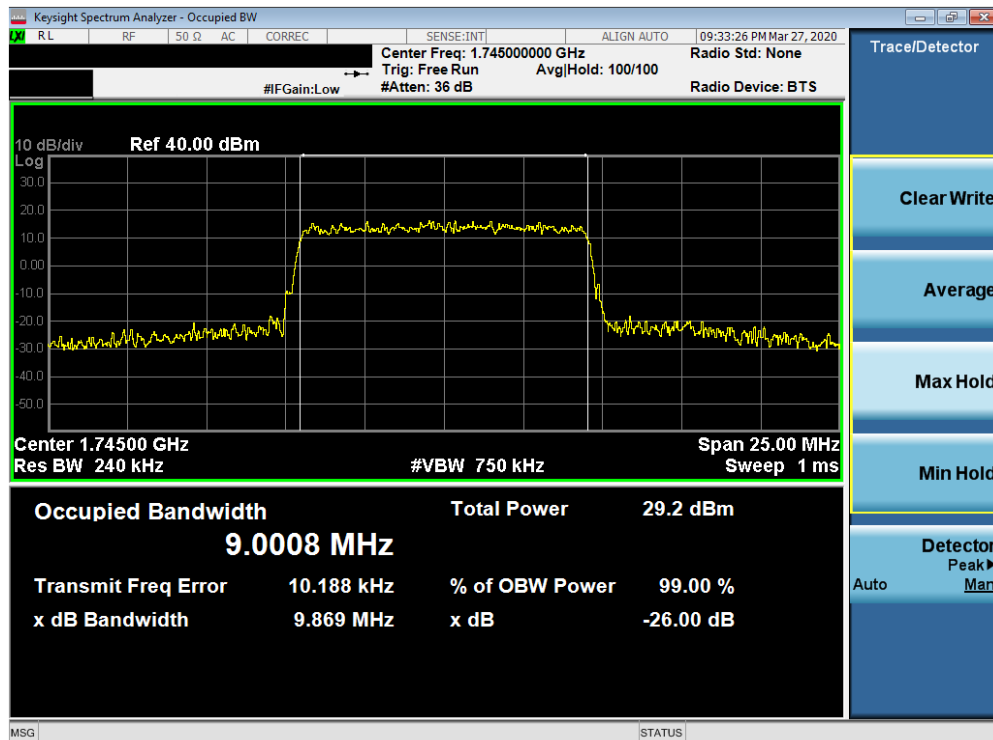
Plot 7-97. Occupied Bandwidth Plot (Band 66/4 - 10.0MHz 64-QAM - Full RB Configuration)
