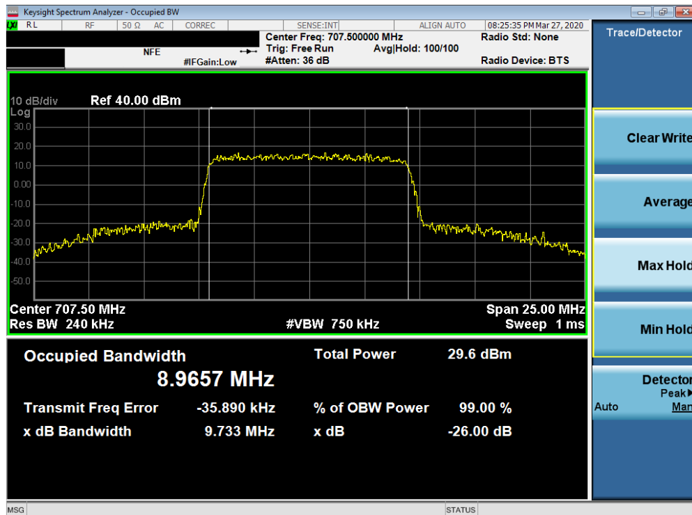
Plot 7-44. Occupied Bandwidth Plot (Band 12 - 10.0MHz 64-QAM - Full RB Configuration)
