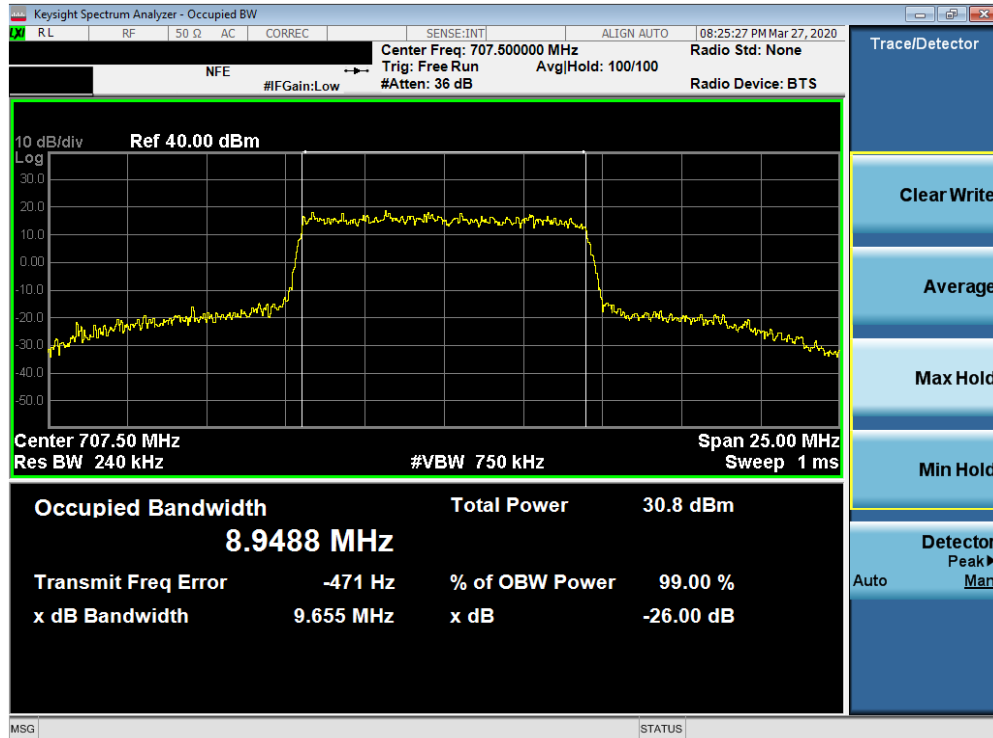
Plot 7-43. Occupied Bandwidth Plot (Band 12 - 10.0MHz 16-QAM - Full RB Configuration)
