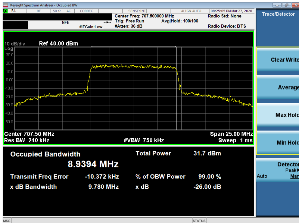
Plot 7-42. Occupied Bandwidth Plot (Band 12 - 10.0MHz QPSK - Full RB Configuration)
