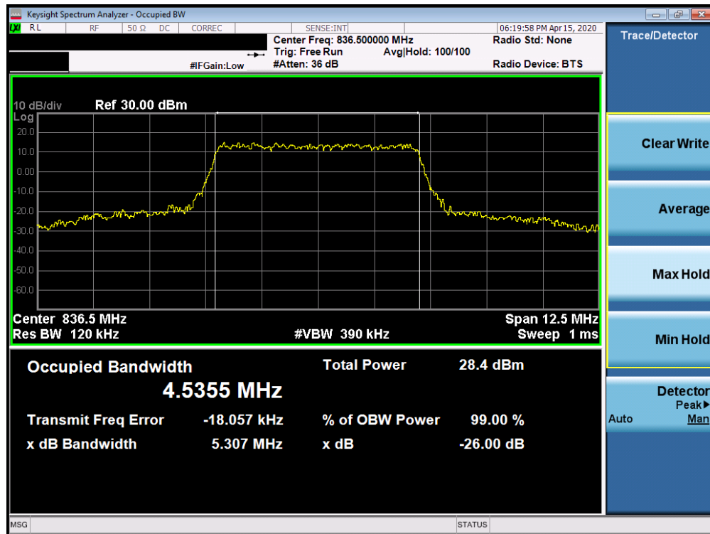
Plot 7-67. Occupied Bandwidth Plot (n5 5MHz QPSK-CP-OFDM - Full RB Configuration)
