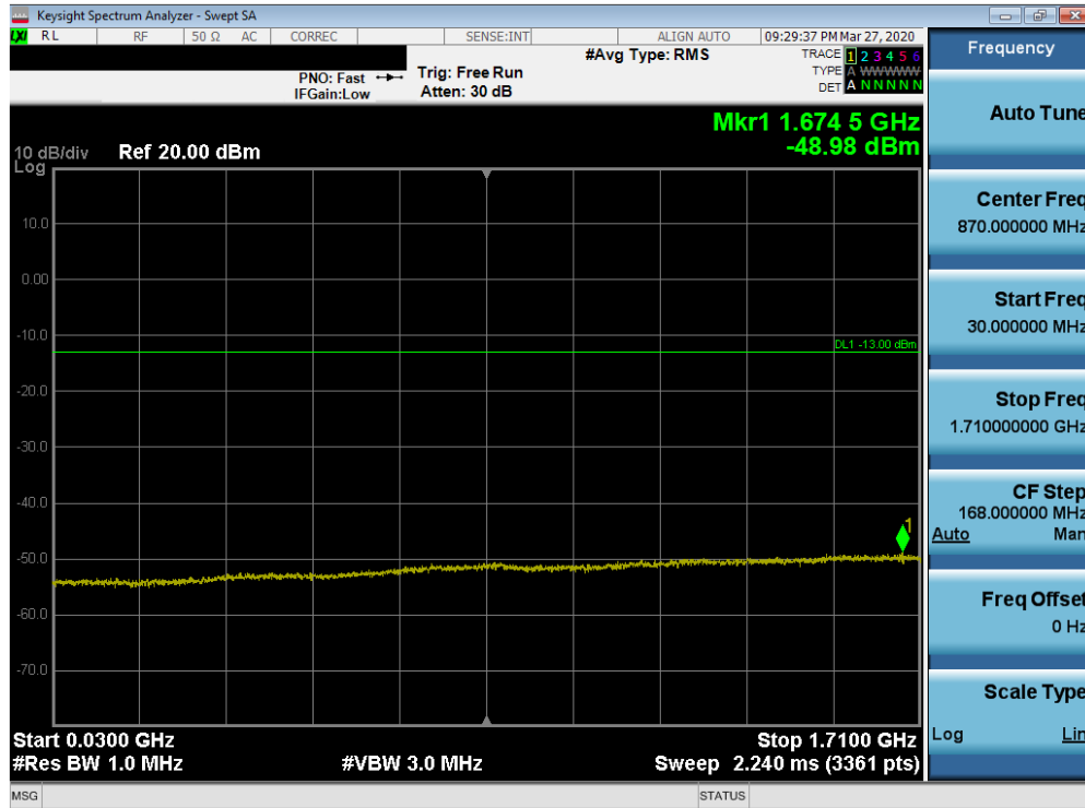
Plot 7-302. Conducted Spurious Plot (Band 66/4 - 20.0MHz QPSK - RB Size 1, RB Offset 0 - High Channel)
