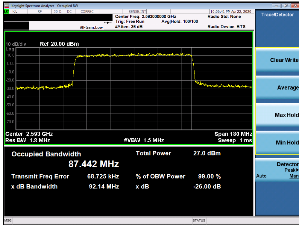
Plot 7-232. Occupied Bandwidth Plot (n41 90MHz 64QAM-CP-OFDM- Full RB Configuration)
