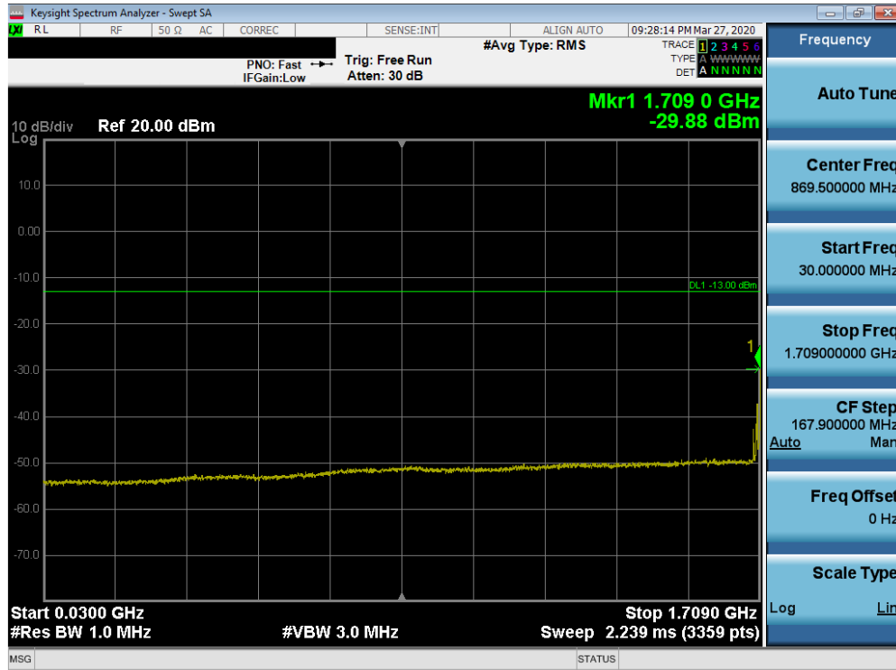
Plot 7-296. Conducted Spurious Plot (Band 66/4 - 20.0MHz QPSK - RB Size 1, RB Offset 0 - Low Channel)
