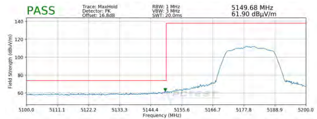
Plot 7-86. Radiated Lower Band Edge Plot (Peak – UNII Band 1)
