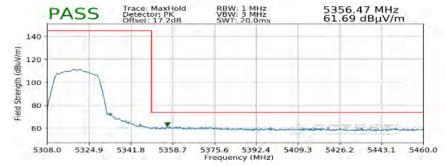
Plot 7-88. Radiated Upper Band Edge Plot (Peak – UNII Band 2A)
