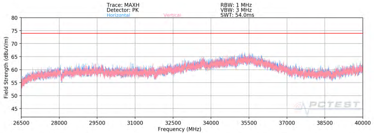
Plot 7-84. Radiated Spurious Plot 26.5GHz - 40GHz (802.11a)
