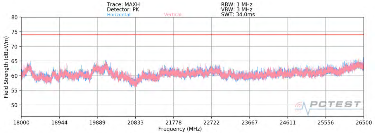
Plot 7-83. Radiated Spurious Plot 18GHz - 26.5GHz (802.11a)
