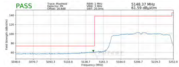
Plot 7-100. Radiated Lower Band Edge Plot (Peak – UNII Band 1)
