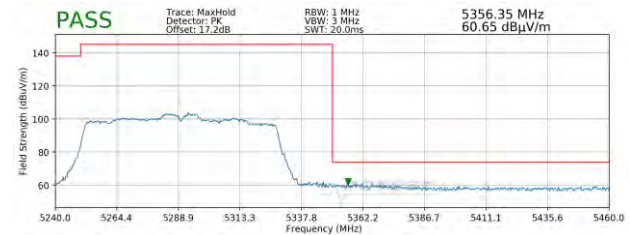
Plot 7-102. Radiated Upper Band Edge Plot (Peak – UNII Band 2A)
