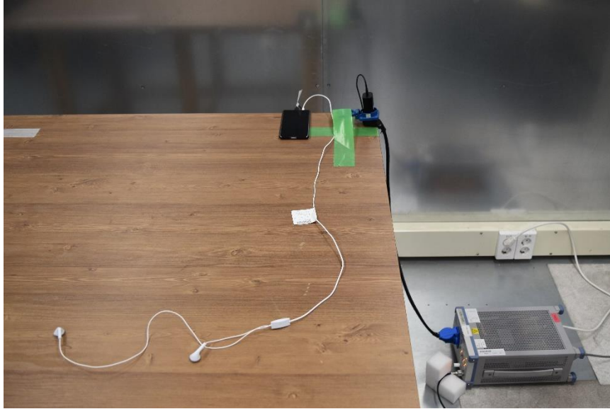
AC LINE CONDUCTED FRONT TEST PHOTO
