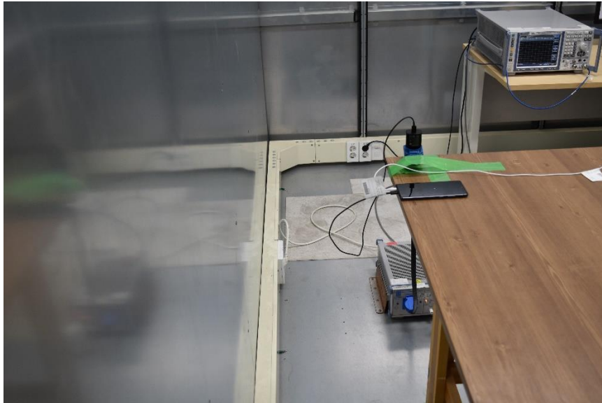
AC LINE CONDUCTED REAR TEST PHOTO
