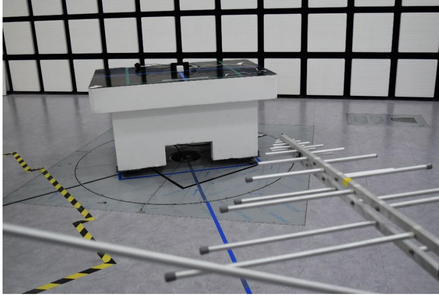
BELOW 1 GHz FRONT TEST PHOTO
