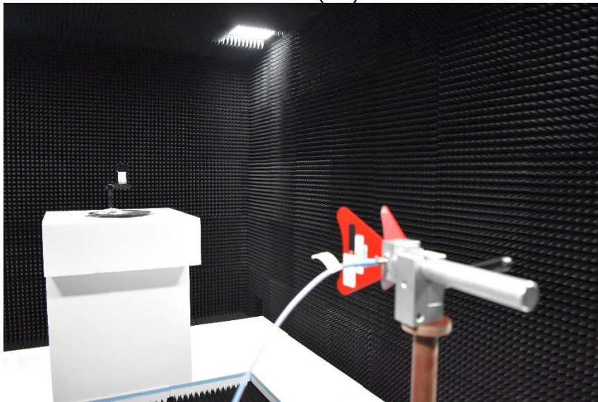
18 - 40 GHz REAR TEST PHOTO (3m)
