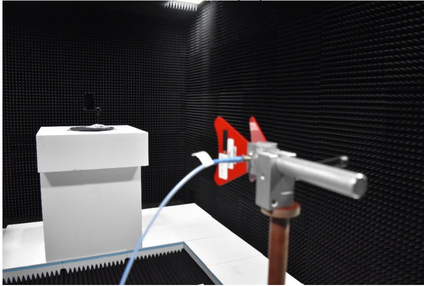
18 - 40 GHz FRONT TEST PHOTO (3m)
