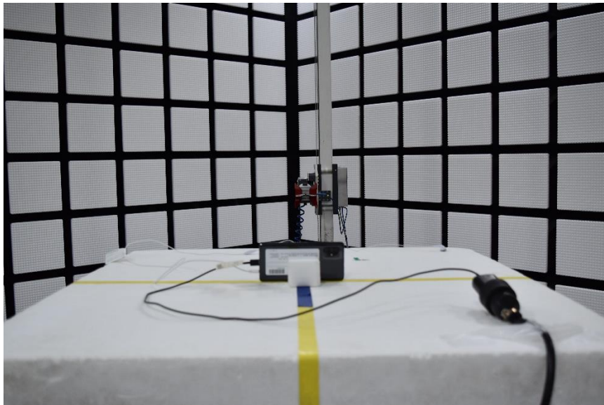
1 - 18 GHz REAR TEST PHOTO
