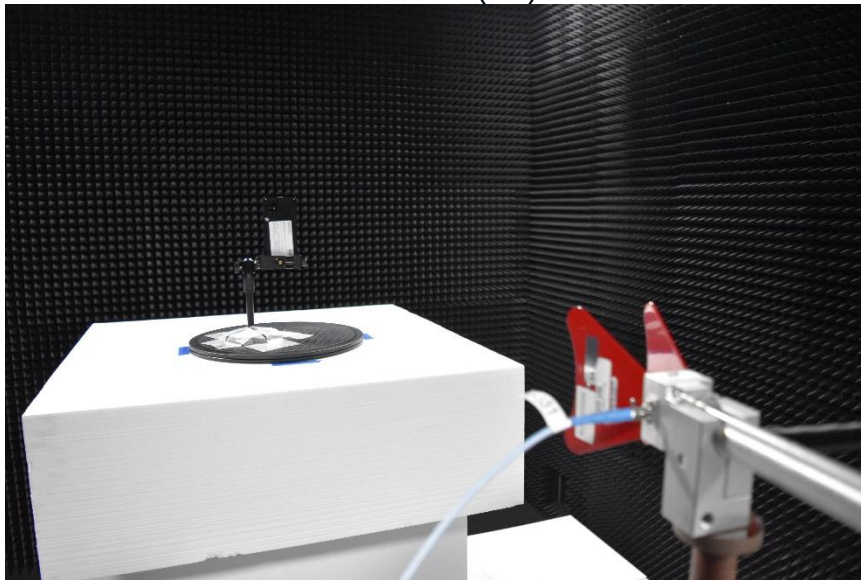
18 - 40 GHz FRONT TEST PHOTO (1m)
