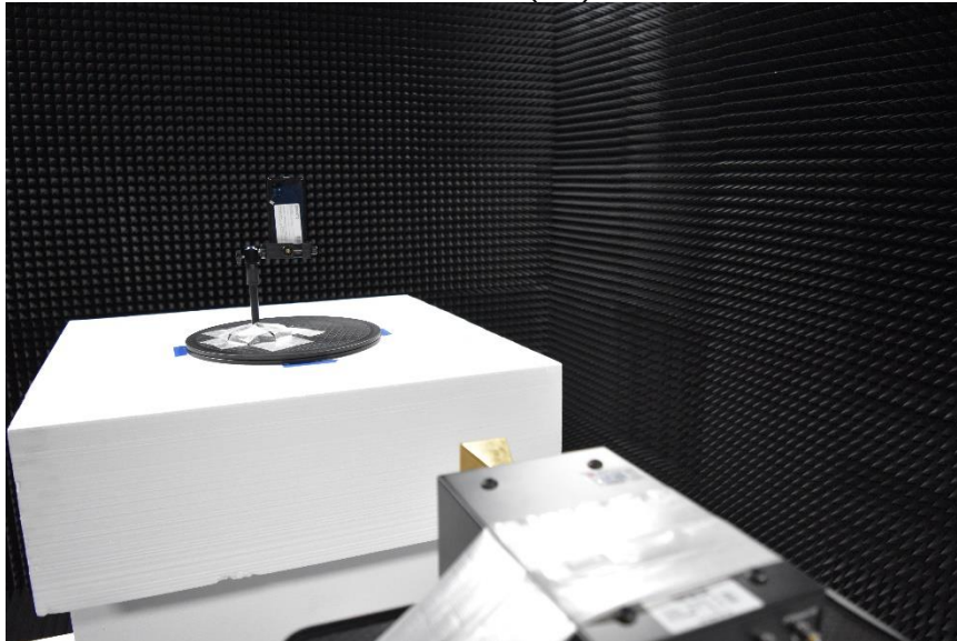
40 - 200 GHz REAR TEST PHOTO (1m)
