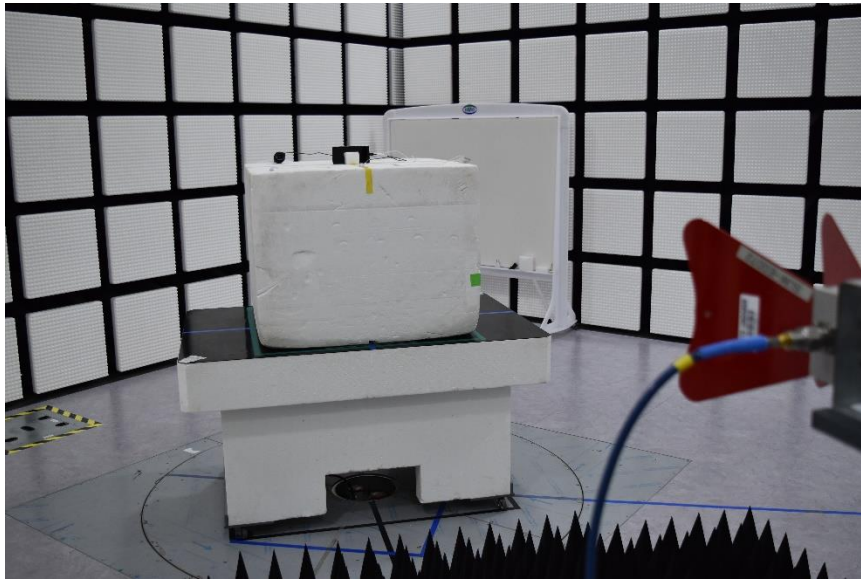
1 - 18 GHz FRONT TEST PHOTO
