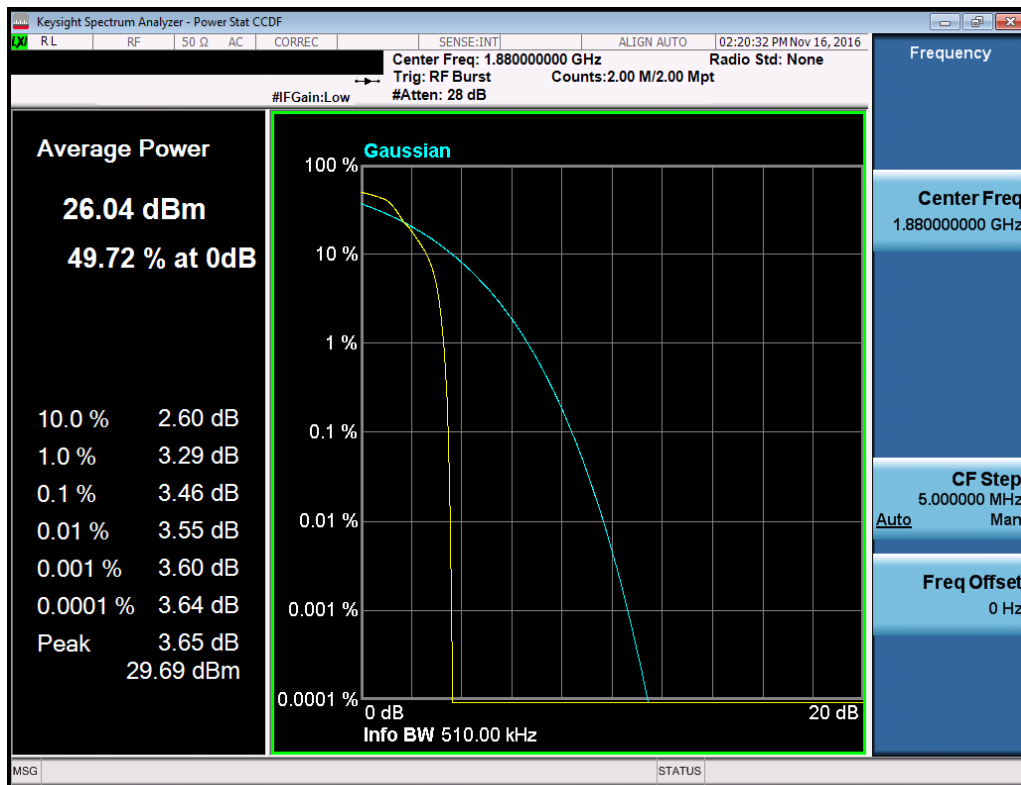
Plot 7-70. Peak-Average Ratio Plot (EDGE1900 Mode – Ch. 661)
