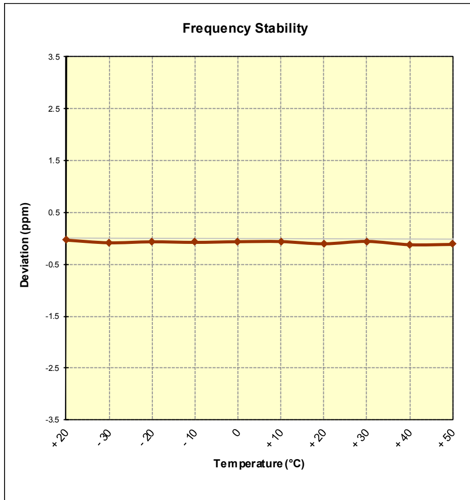
Figure 7-10. Frequency Stability Graph (AWS WCDMA Mode – Ch. 1412)
