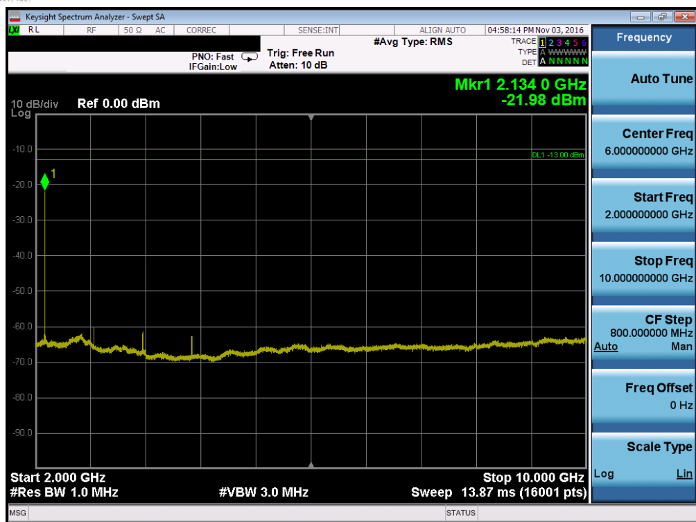
Plot 7-53. Conducted Spurious Plot (Band 17 – 5.0MHz QPSK – RB Size 1, RB Offset 0 – High Channel)
