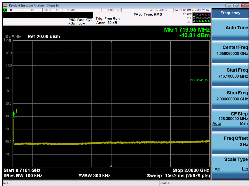
Plot 7-52. Conducted Spurious Plot (Band 17 – 5.0MHz QPSK – RB Size 1, RB Offset 0 – High Channel)
