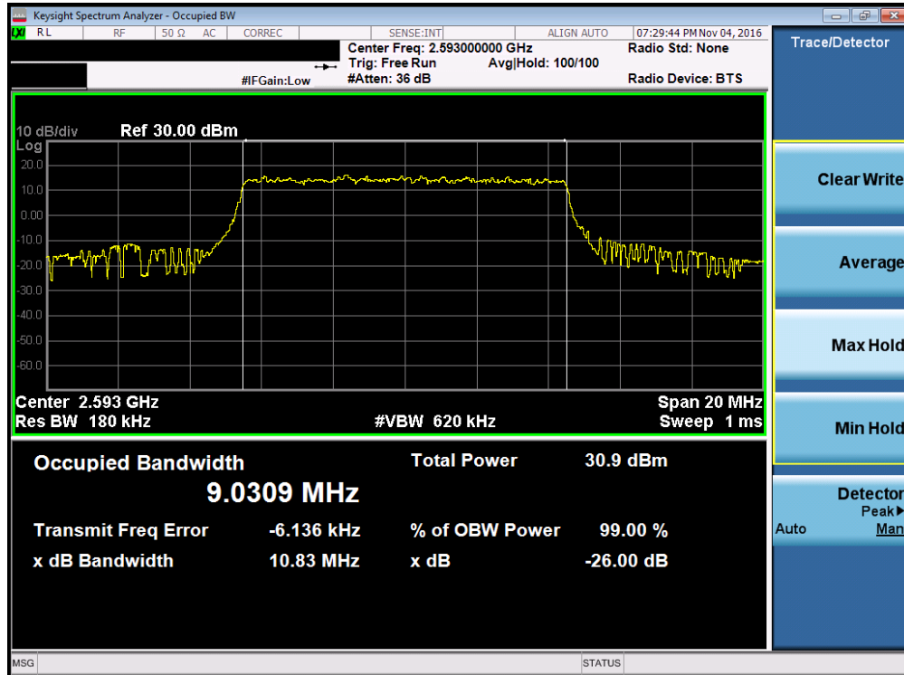
Plot 7-39. Occupied Bandwidth Plot (Band 41 – 10.0MHz QPSK – RB Size 50)
