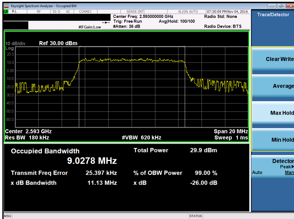
Plot 7-40. Occupied Bandwidth Plot (Band 41 – 10.0MHz 16-QAM – RB Size 50)
