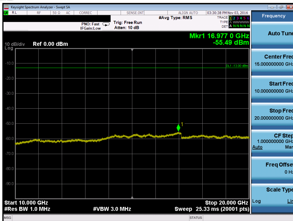
Plot 7-71. Conducted Spurious Plot (Band 4 – 1.4MHz QPSK – RB Size 1, RB Offset 0 – High Channel)
