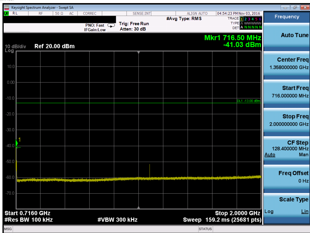
Plot 7-49. Conducted Spurious Plot (Band 17 – 5.0MHz QPSK – RB Size 1, RB Offset 0 – Mid Channel)
