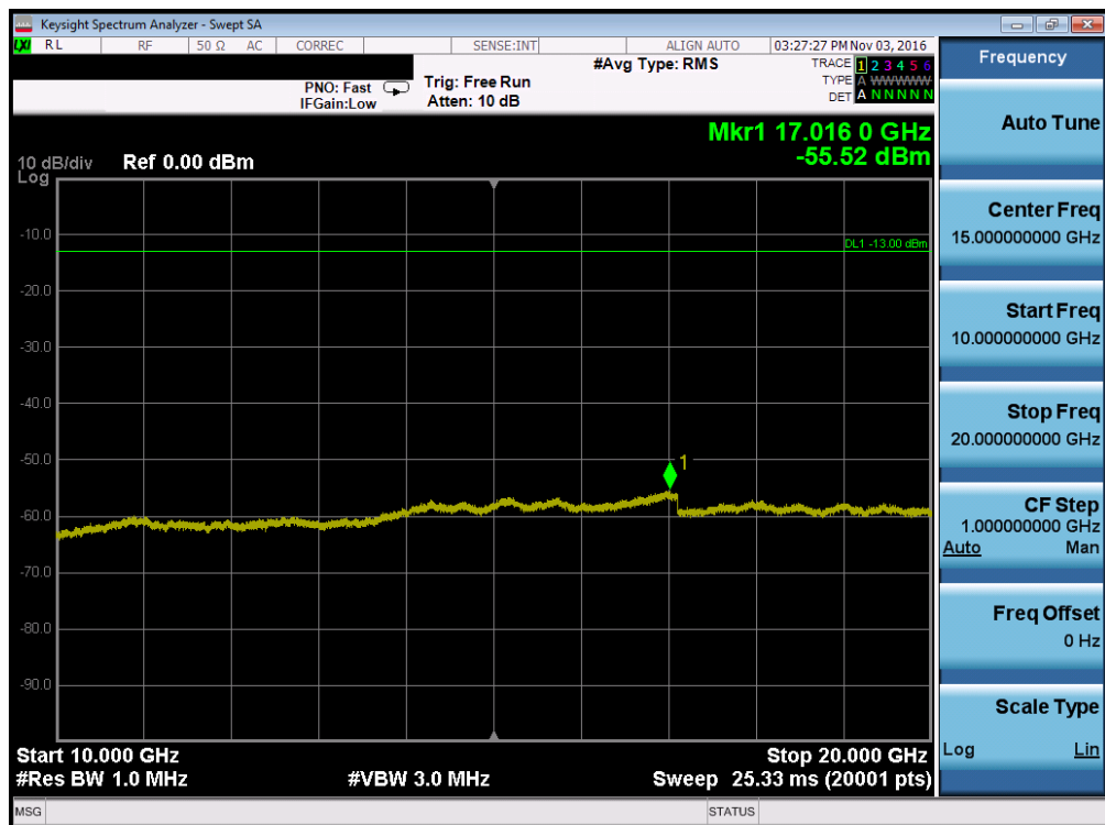
Plot 7-68. Conducted Spurious Plot (Band 4 – 1.4MHz QPSK – RB Size 1, RB Offset 0 – Mid Channel)
