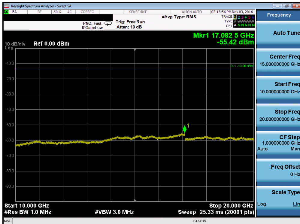
Plot 7-80. Conducted Spurious Plot (Band 2 – 5.0MHz QPSK – RB Size 1, RB Offset 0 – High Channel)
