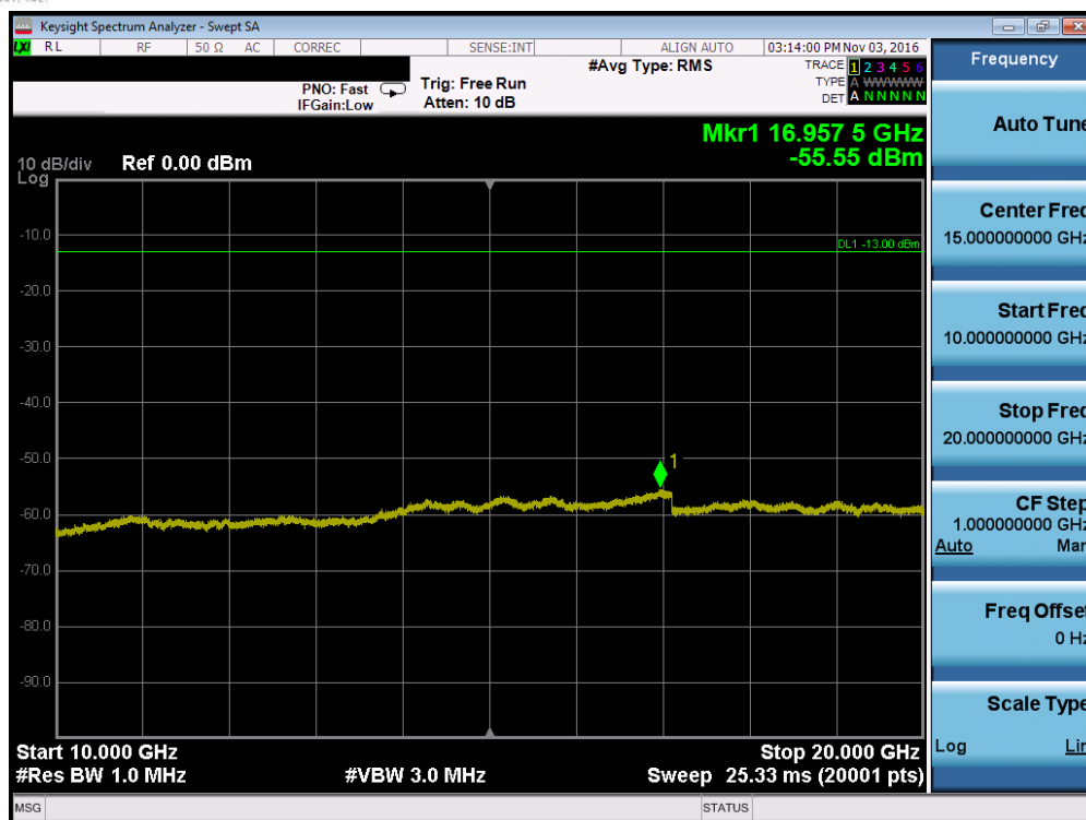
Plot 7-77. Conducted Spurious Plot (Band 2 – 5.0MHz QPSK – RB Size 1, RB Offset 0 – Mid Channel)
