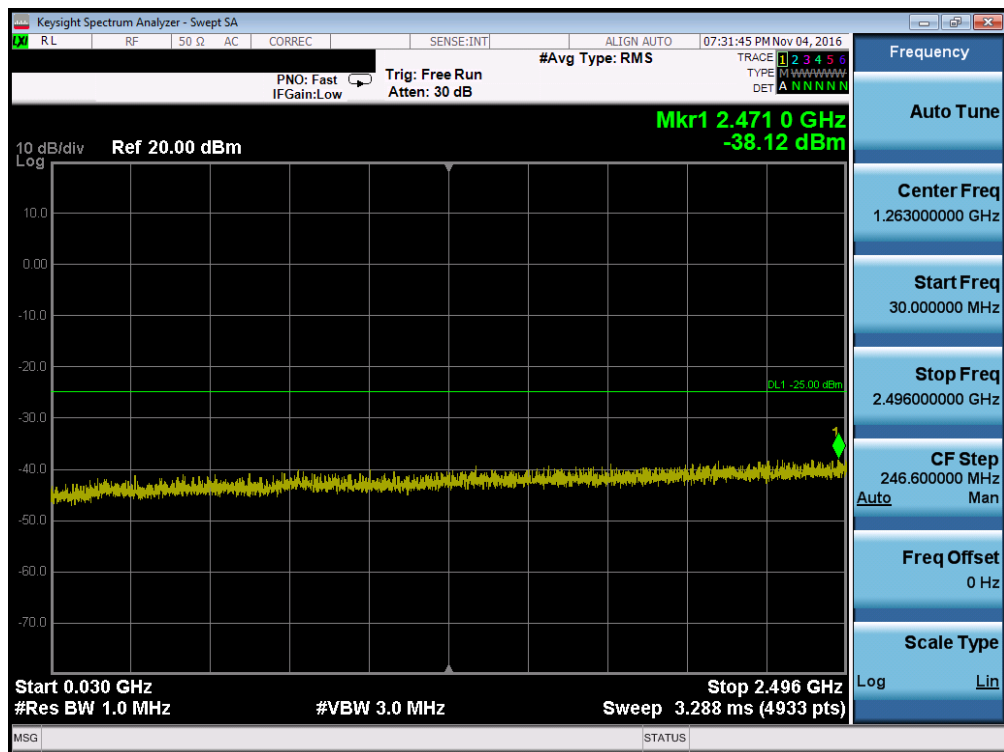
Plot 7-84. Conducted Spurious Plot (Band 41 – 10.0MHz QPSK – RB Size 1, RB Offset 0 – Mid Channel)
