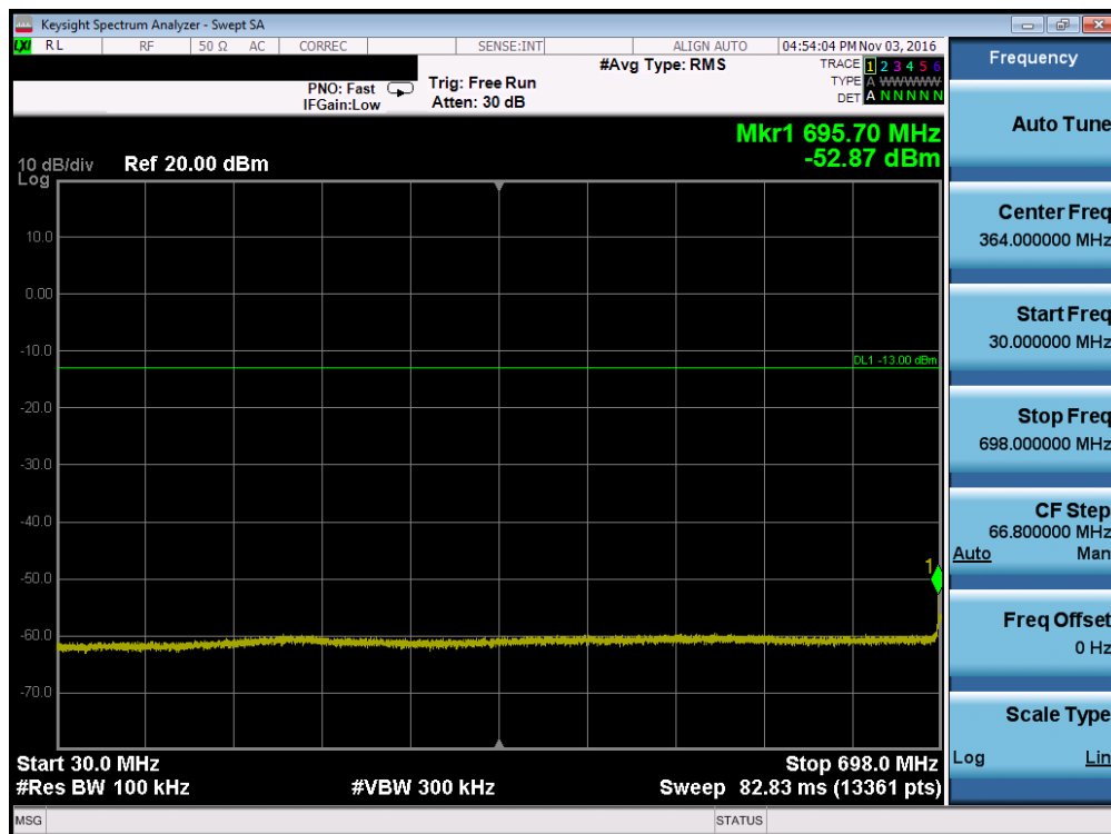
Plot 7-48. Conducted Spurious Plot (Band 17 – 5.0MHz QPSK – RB Size 1, RB Offset 0 – Mid Channel)
