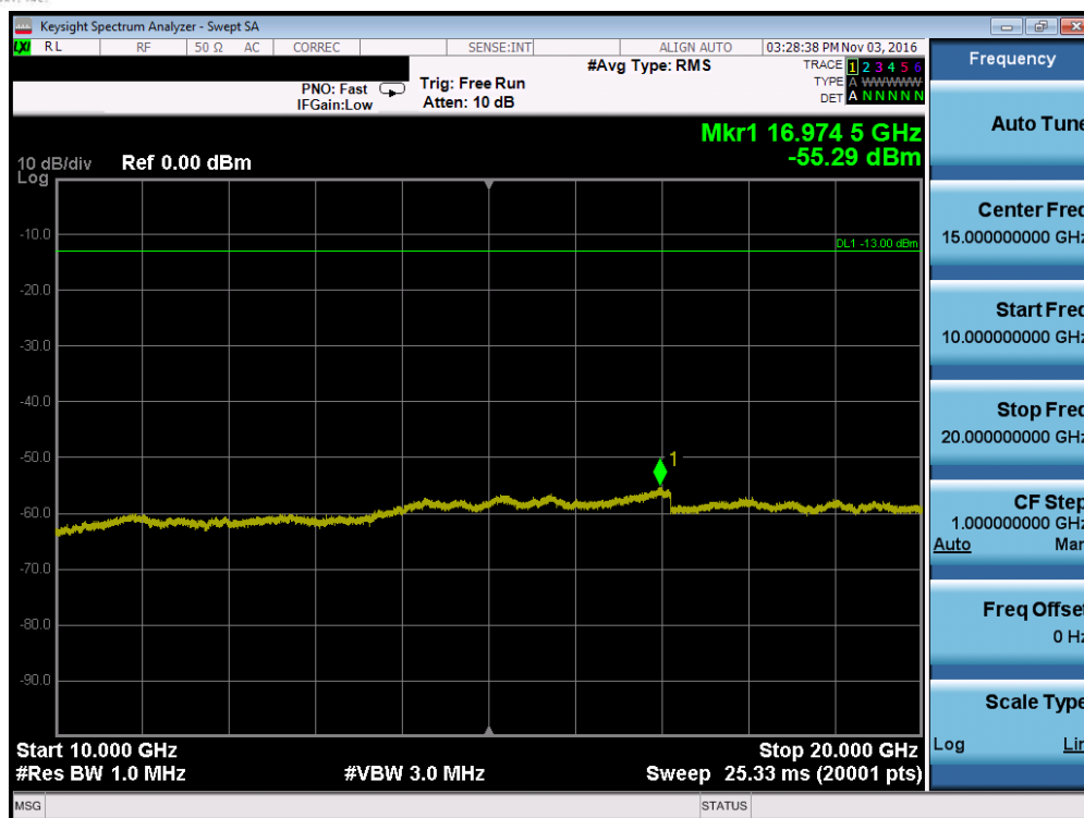
Plot 7-65. Conducted Spurious Plot (Band 4 – 1.4MHz QPSK – RB Size 1, RB Offset 0 – Low Channel)
