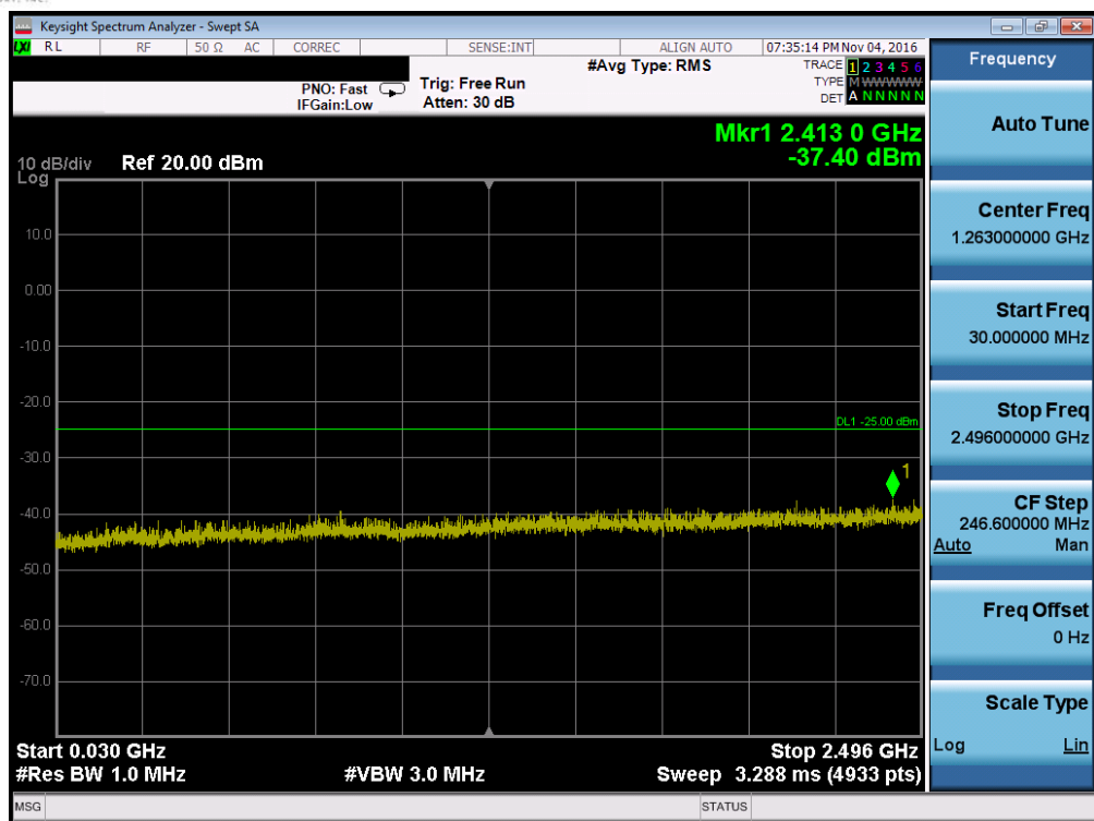
Plot 7-87. Conducted Spurious Plot (Band 41 – 10.0MHz QPSK – RB Size 1, RB Offset 0 – High Channel)
