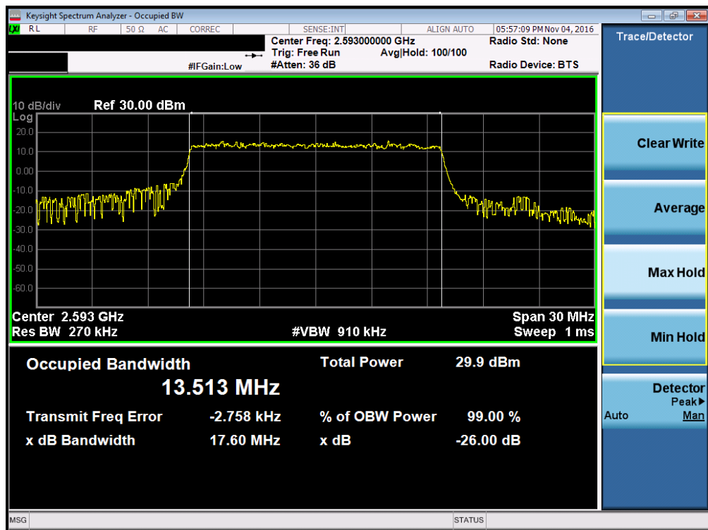
Plot 7-42. Occupied Bandwidth Plot (Band 41 – 15.0MHz 16-QAM – RB Size 75)
