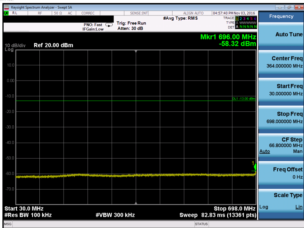
Plot 7-51. Conducted Spurious Plot (Band 17 – 5.0MHz QPSK – RB Size 1, RB Offset 0 – High Channel)
