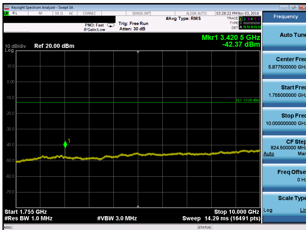
Plot 7-64. Conducted Spurious Plot (Band 4 – 1.4MHz QPSK – RB Size 1, RB Offset 0 – Low Channel)
