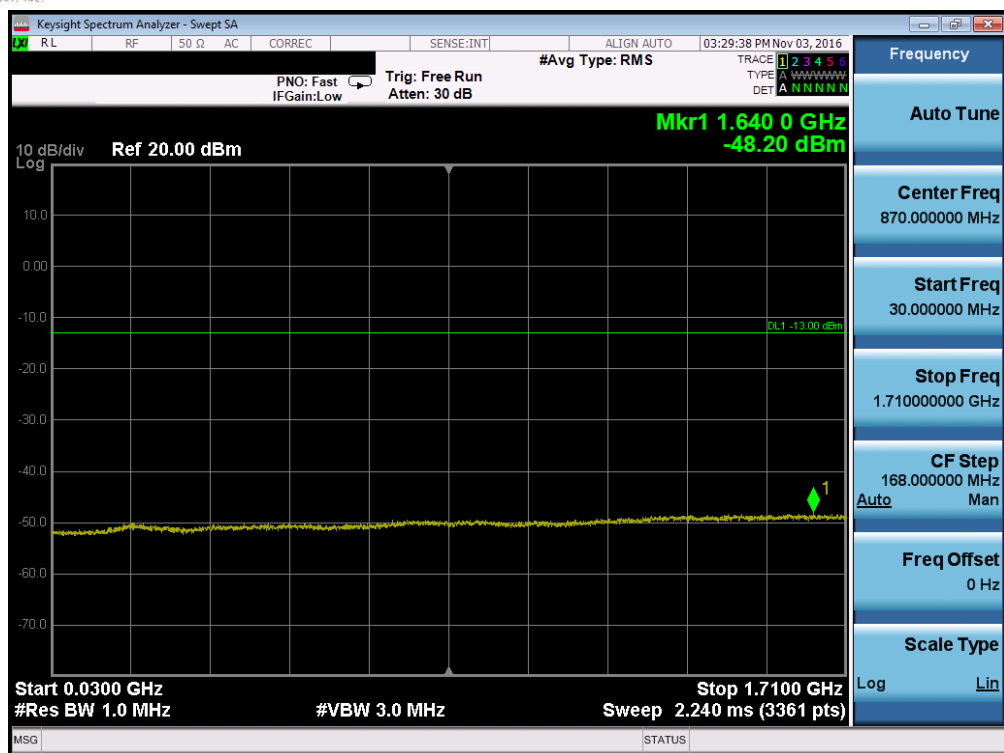
Plot 7-69. Conducted Spurious Plot (Band 4 – 1.4MHz QPSK – RB Size 1, RB Offset 0 – High Channel)
