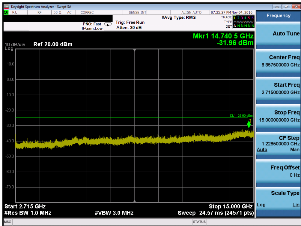
Plot 7-88. Conducted Spurious Plot (Band 41 – 10.0MHz QPSK – RB Size 1, RB Offset 0 – High Channel)
