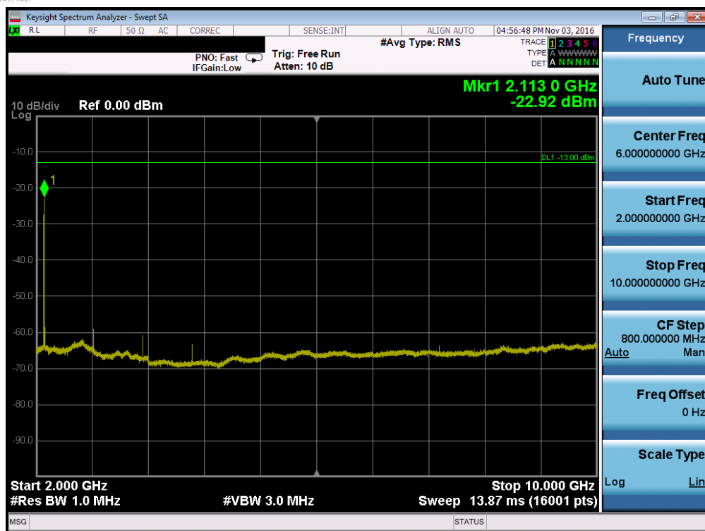
Plot 7-47. Conducted Spurious Plot (Band 17 – 5.0MHz QPSK – RB Size 1, RB Offset 0 – Low Channel)
