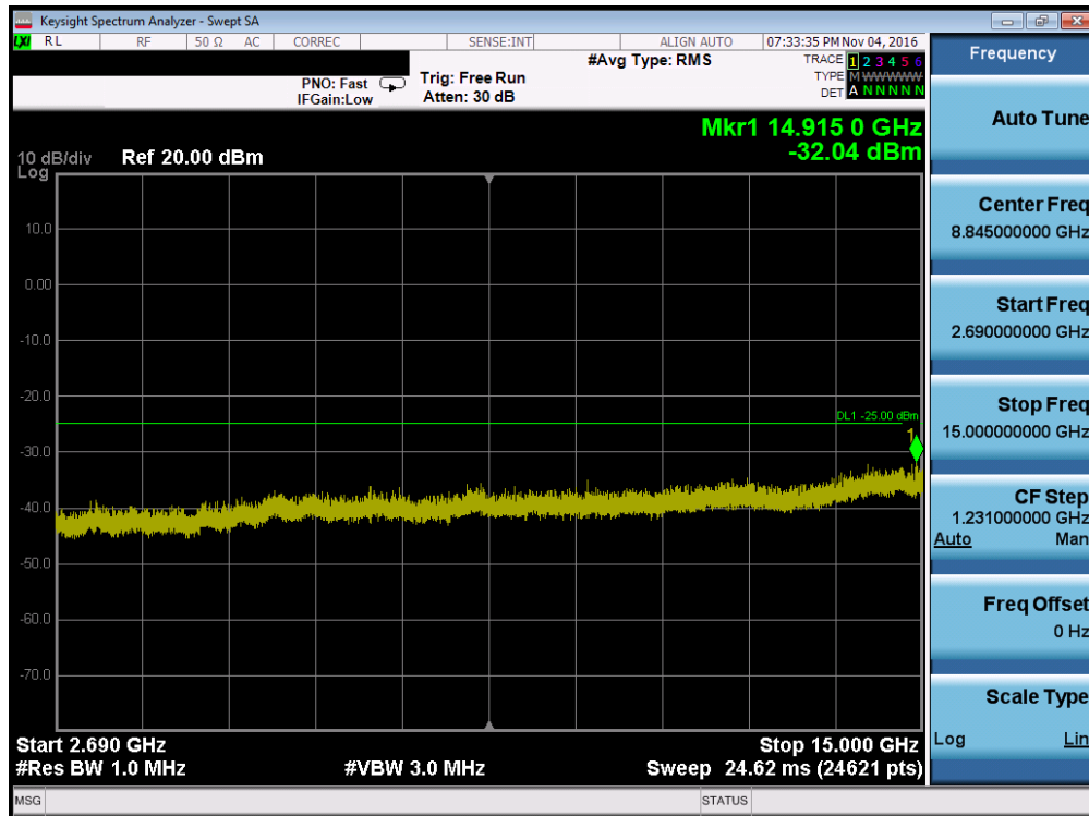
Plot 7-82. Conducted Spurious Plot (Band 41 – 10.0MHz QPSK – RB Size 1, RB Offset 0 – Low Channel)
