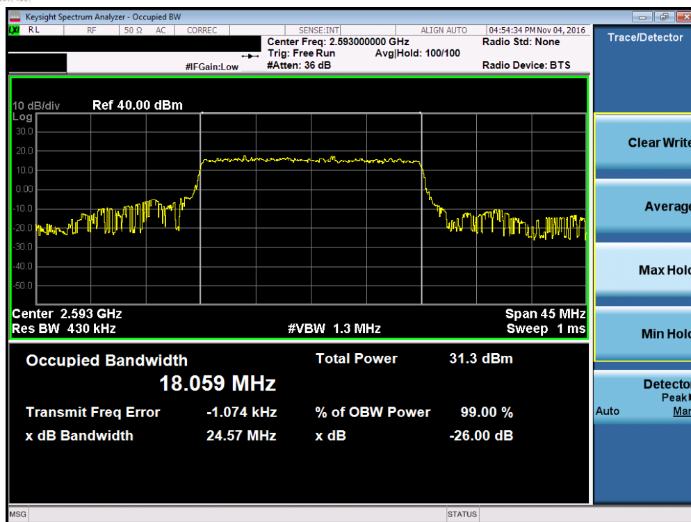
Plot 7-43. Occupied Bandwidth Plot (Band 41 – 20.0MHz QPSK – RB Size 100)
