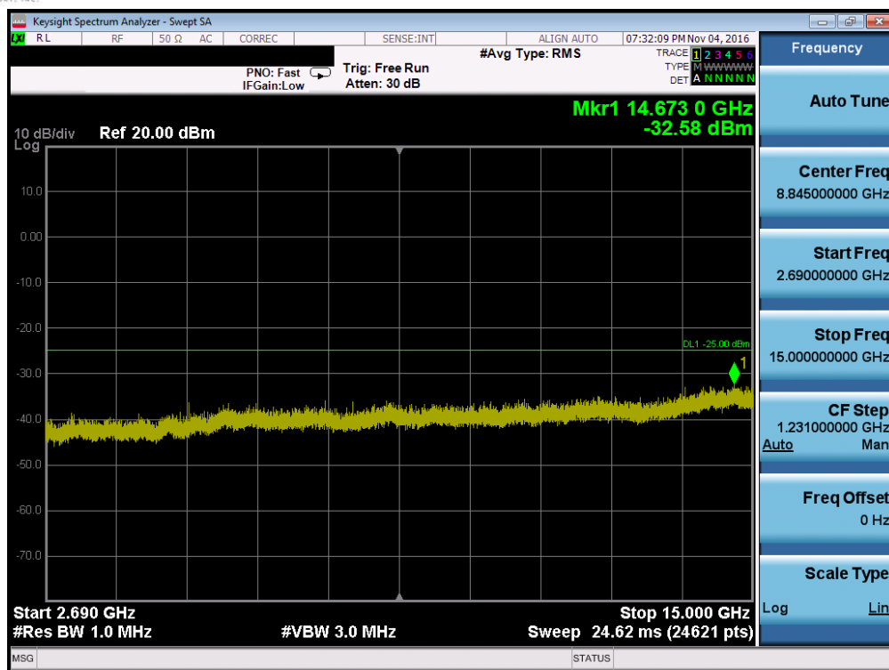
Plot 7-85. Conducted Spurious Plot (Band 41 – 10.0MHz QPSK – RB Size 1, RB Offset 0 – Mid Channel)
