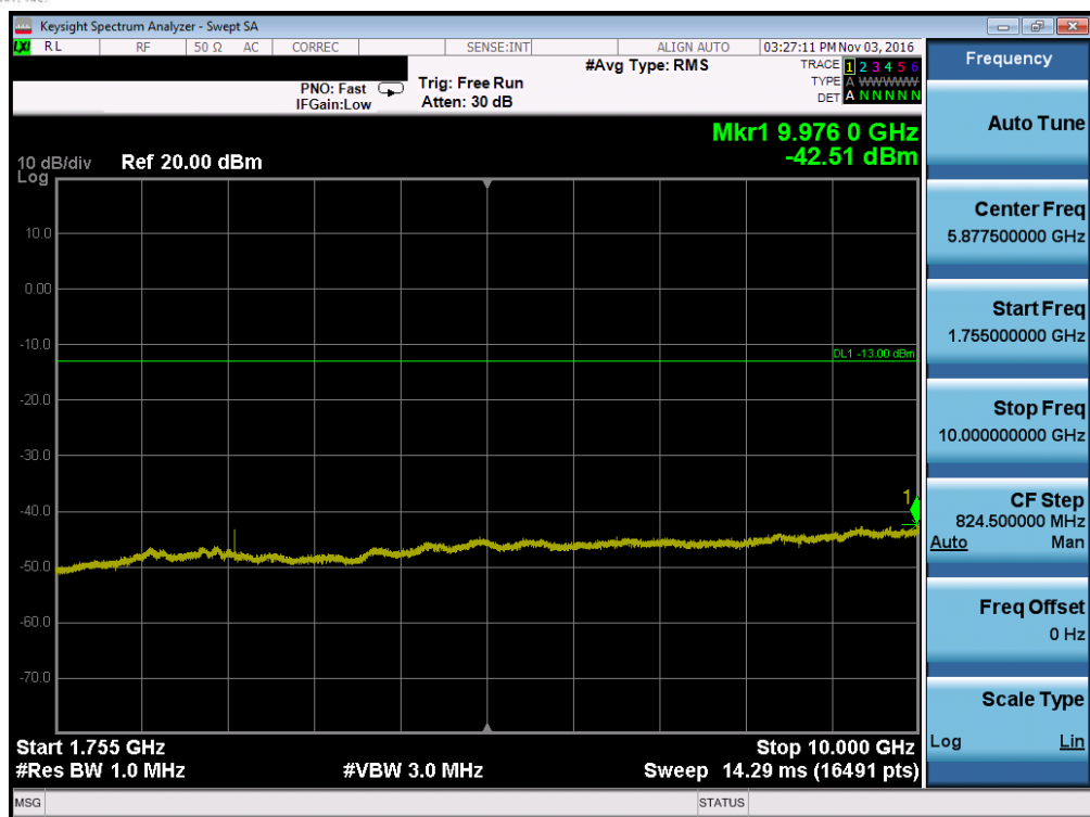
Plot 7-67. Conducted Spurious Plot (Band 4 – 1.4MHz QPSK – RB Size 1, RB Offset 0 – Mid Channel)
