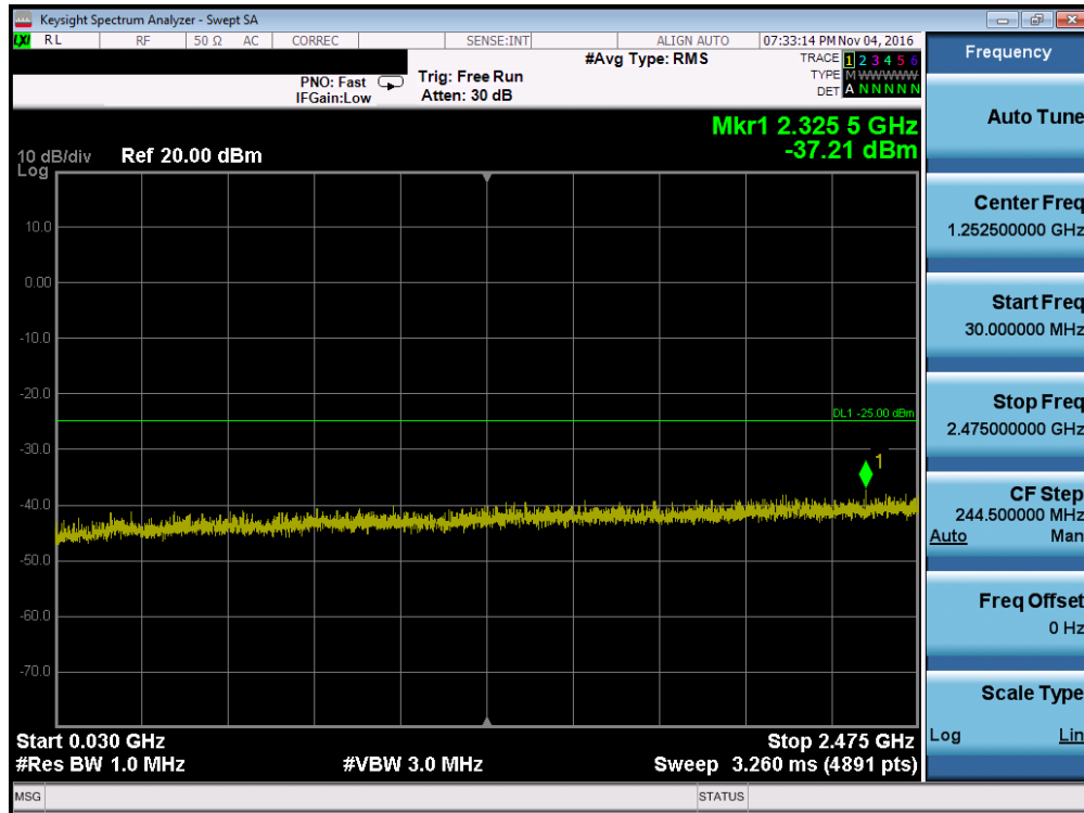
Plot 7-81. Conducted Spurious Plot (Band 41 – 10.0MHz QPSK – RB Size 1, RB Offset 0– Low Channel)
