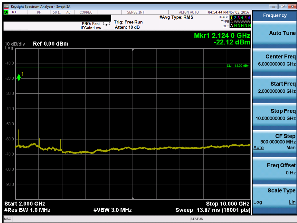
Plot 7-50. Conducted Spurious Plot (Band 17 – 5.0MHz QPSK – RB Size 1, RB Offset 0 – Mid Channel)
