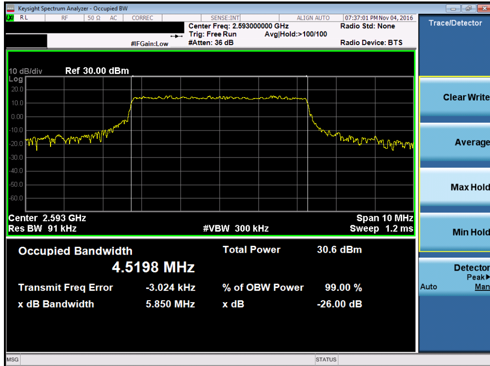
Plot 7-37. Occupied Bandwidth Plot (Band 41 – 5.0MHz QPSK – RB Size 25)
