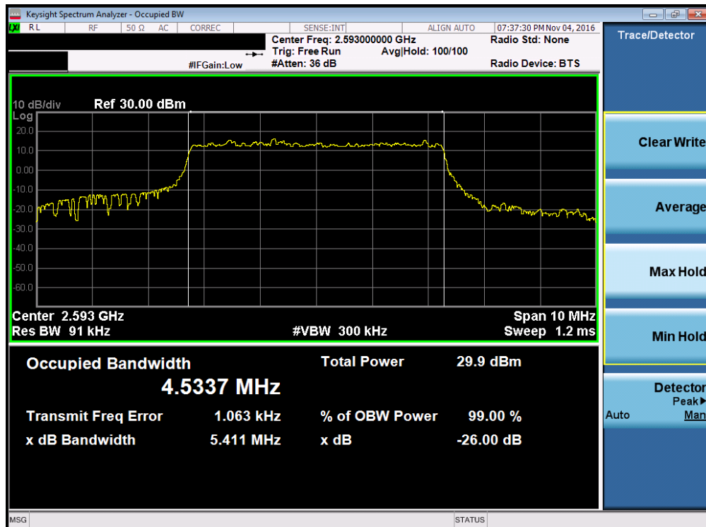
Plot 7-38. Occupied Bandwidth Plot (Band 41 – 5.0MHz 16-QAM – RB Size 25)
