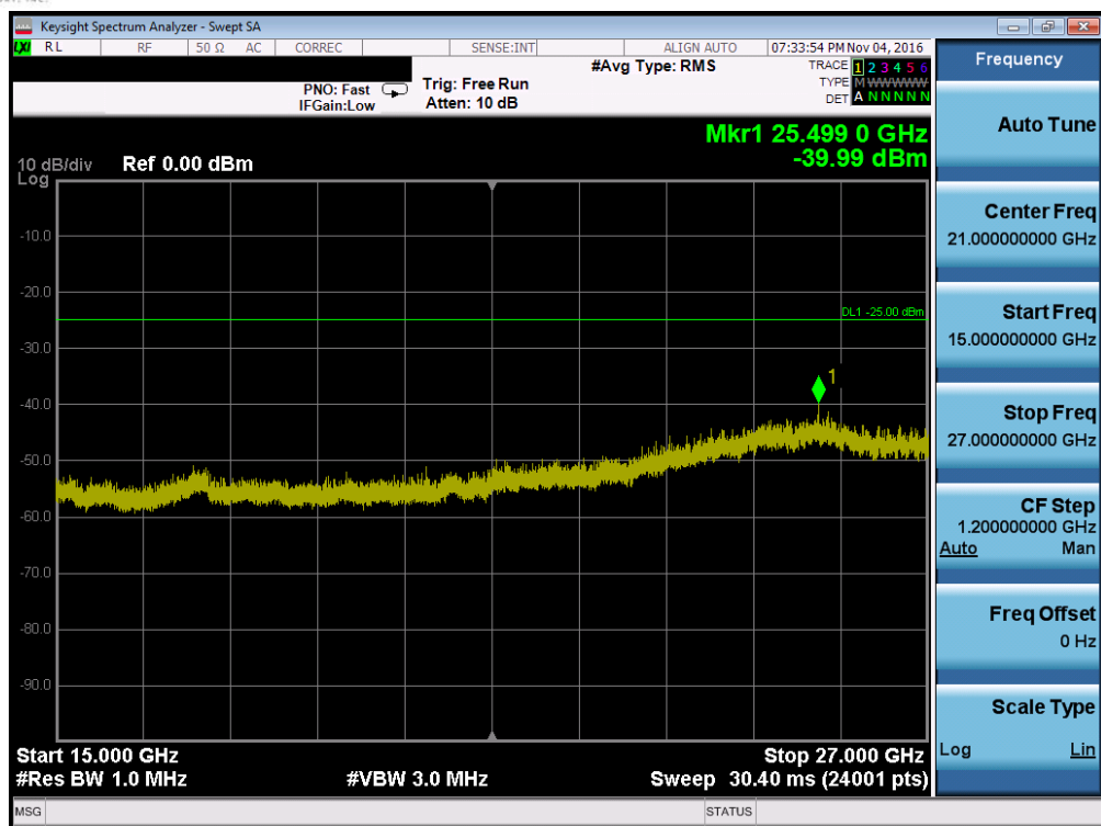
Plot 7-83. Conducted Spurious Plot (Band 41 – 10.0MHz QPSK – RB Size 1, RB Offset 0 – Low Channel)
