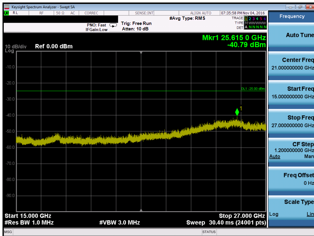
Plot 7-89. Conducted Spurious Plot (Band 41 – 10.0MHz QPSK – RB Size 1, RB Offset 0 – High Channel)
