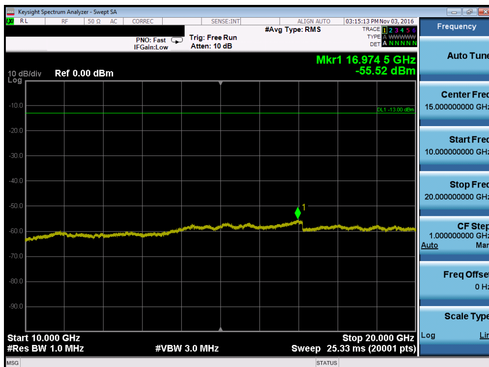
Plot 7-74. Conducted Spurious Plot (Band 2 – 5.0MHz QPSK – RB Size 1, RB Offset 0 – Low Channel)
