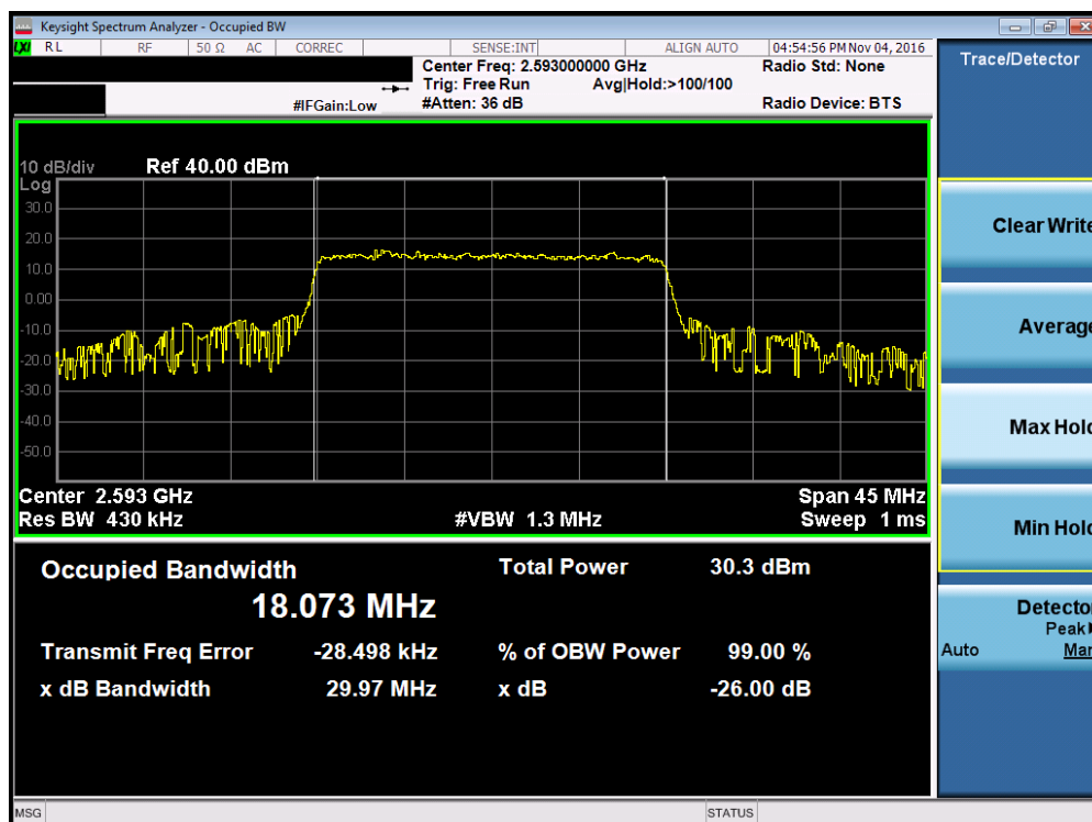
Plot 7-44. Occupied Bandwidth Plot (Band 41 – 20.0MHz 16-QAM – RB Size 100)
