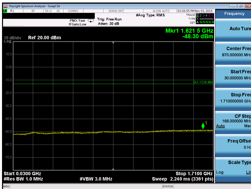
Plot 7-66. Conducted Spurious Plot (Band 4 – 1.4MHz QPSK – RB Size 1, RB Offset 0 – Mid Channel)
