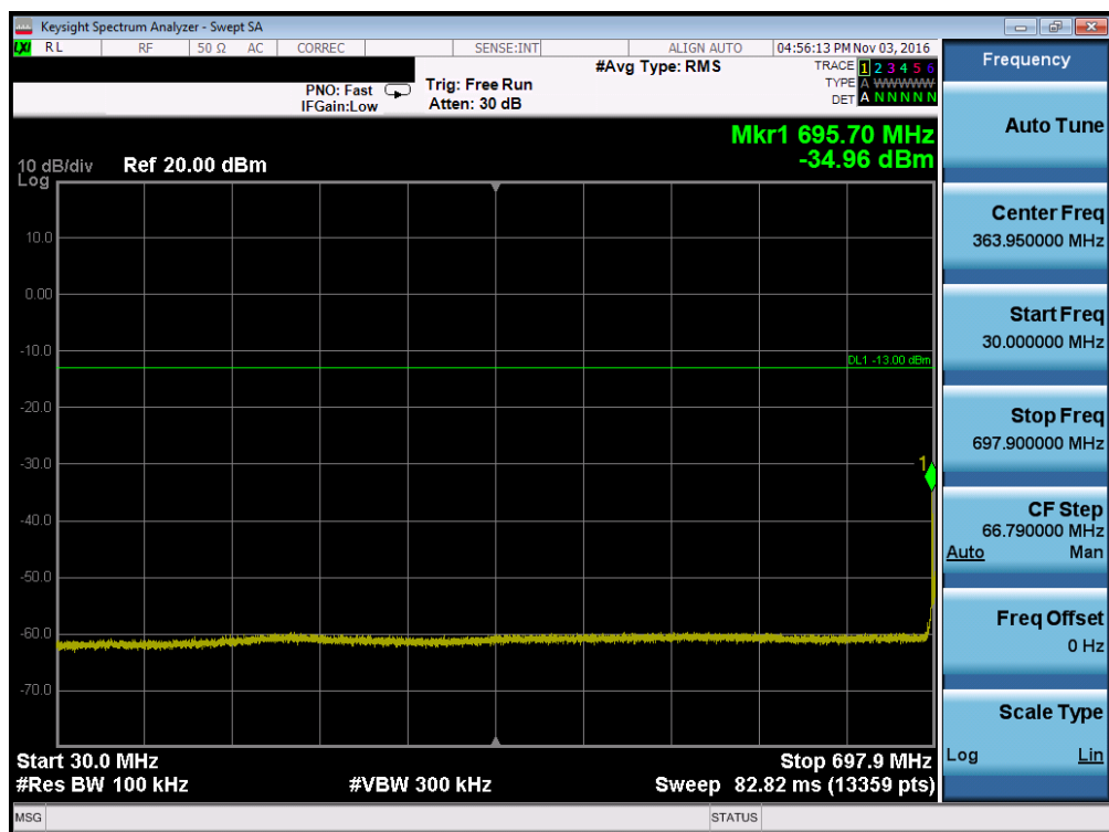
Plot 7-45. Conducted Spurious Plot (Band 17 – 5.0MHz QPSK – RB Size 1, RB Offset 0 – Low Channel)
