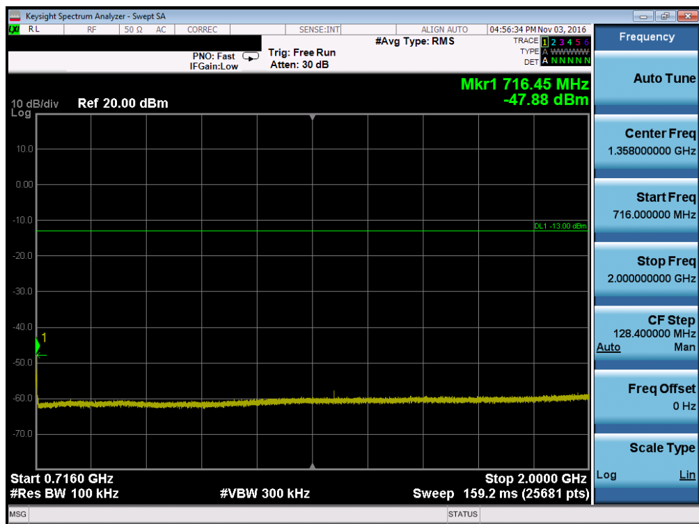
Plot 7-46. Conducted Spurious Plot (Band 17 – 5.0MHz QPSK – RB Size 1, RB Offset 0 – Low Channel)
