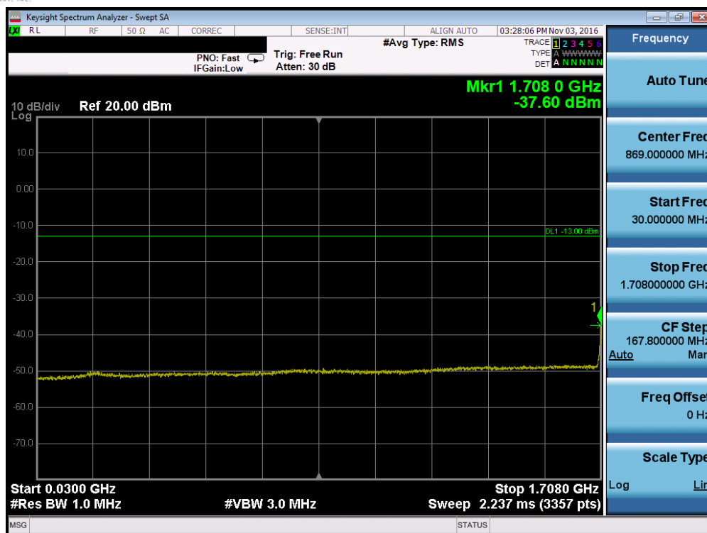
Plot 7-63. Conducted Spurious Plot (Band 4 – 1.4MHz QPSK – RB Size 1, RB Offset 0 – Low Channel)
