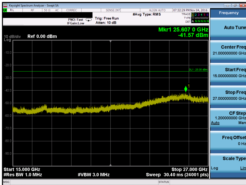
Plot 7-86. Conducted Spurious Plot (Band 41 – 10.0MHz QPSK – RB Size 1, RB Offset 0 – Mid Channel)
