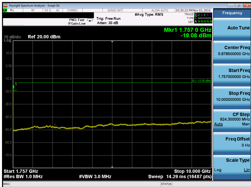
Plot 7-70. Conducted Spurious Plot (Band 4 – 1.4MHz QPSK – RB Size 1, RB Offset 0 – High Channel)
