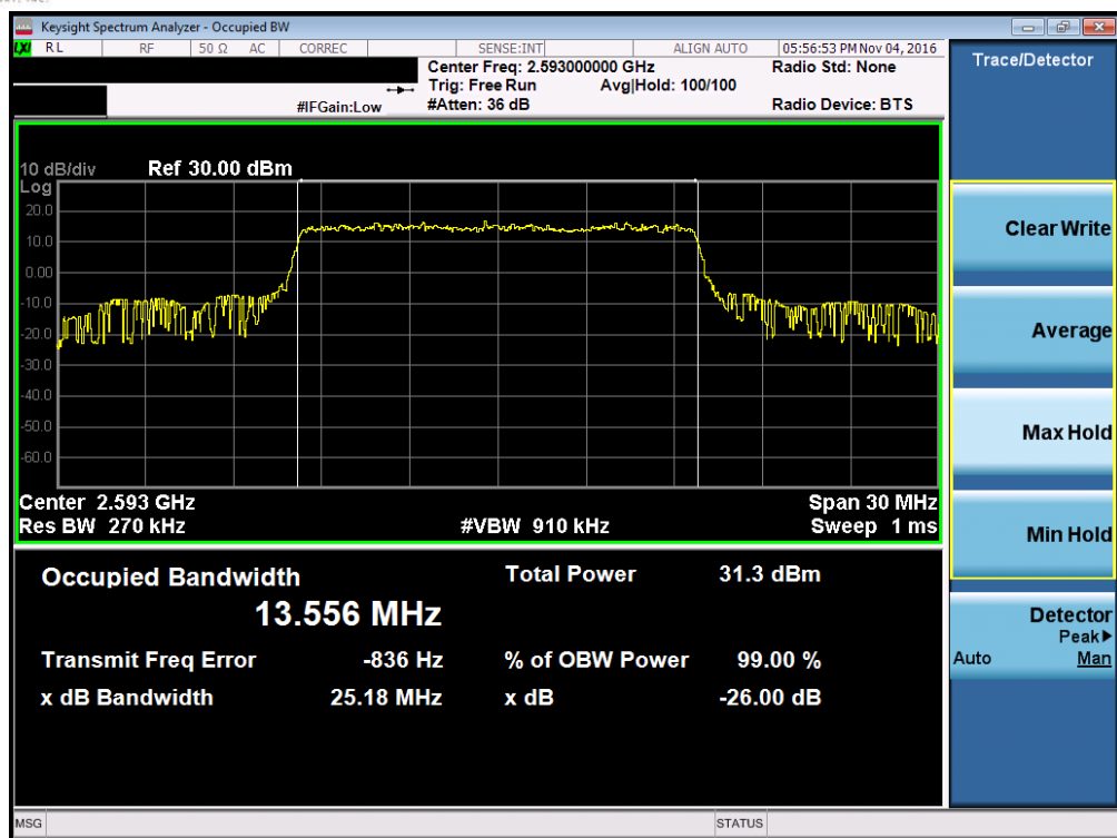
Plot 7-41. Occupied Bandwidth Plot (Band 41 – 15.0MHz QPSK – RB Size 75)
