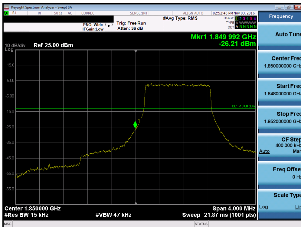
Plot 7-134. Lower Band Edge Plot (Band 2 – 1.4MHz QPSK – RB Size 6)
