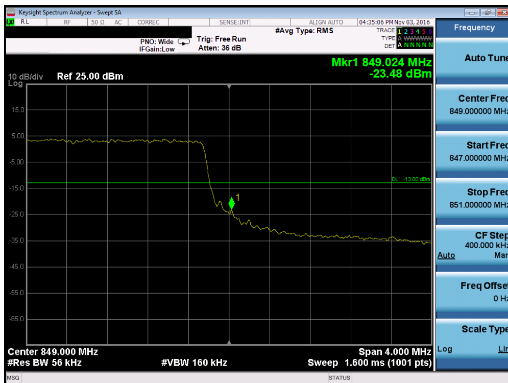
Plot 7-106. Upper Band Edge Plot (Band 5 – 5.0MHz QPSK – RB Size 25)
