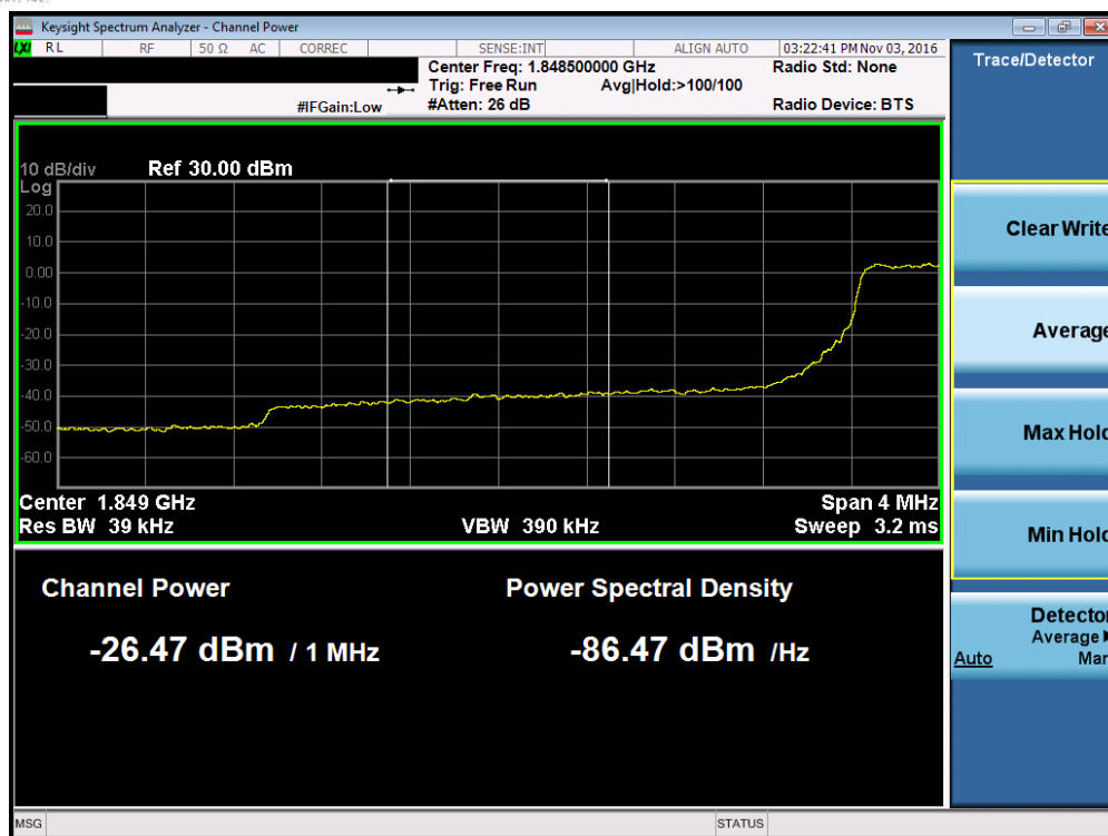
Plot 7-139. Lower Extended Band Edge Plot (Band 2 – 3.0MHz QPSK – RB Size 15)
