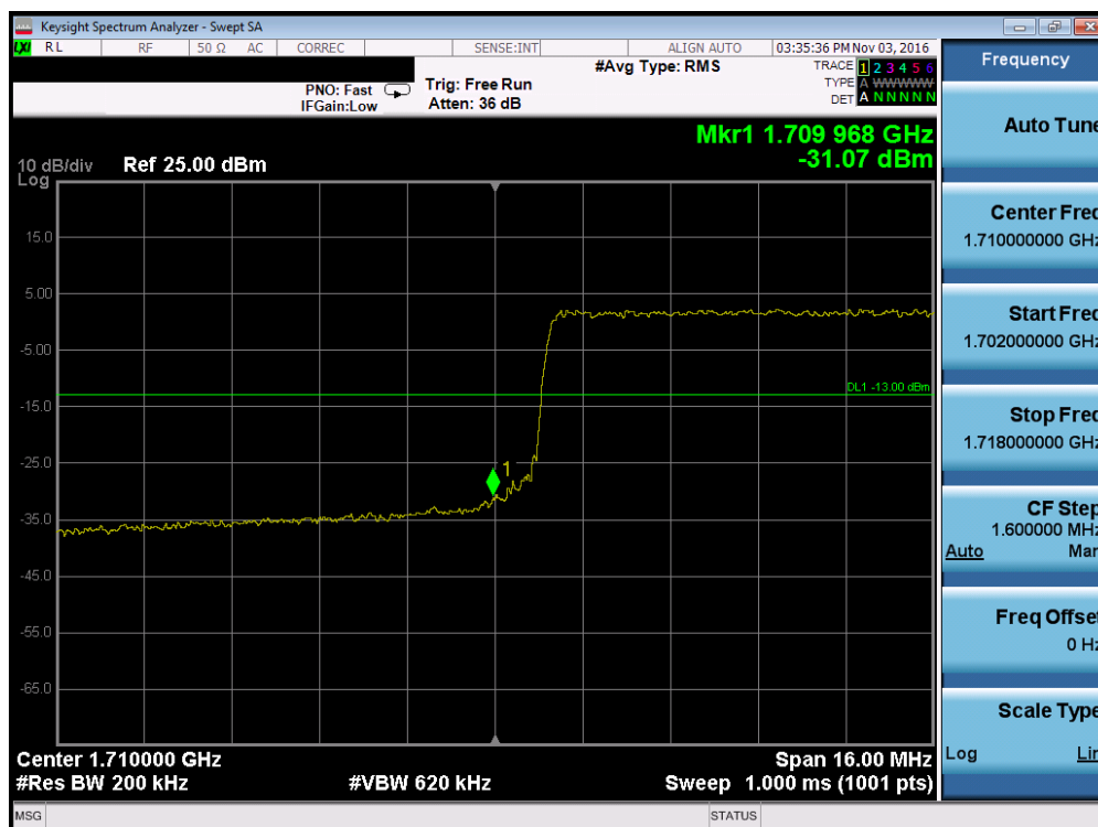
Plot 7-130. Lower Band Edge Plot (Band 4 – 20.0MHz QPSK – RB Size 100)
