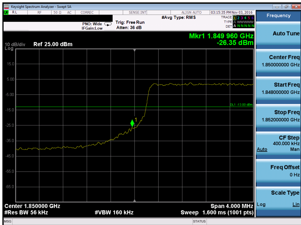
Plot 7-142. Lower Band Edge Plot (Band 2 – 5.0MHz QPSK – RB Size 25)
