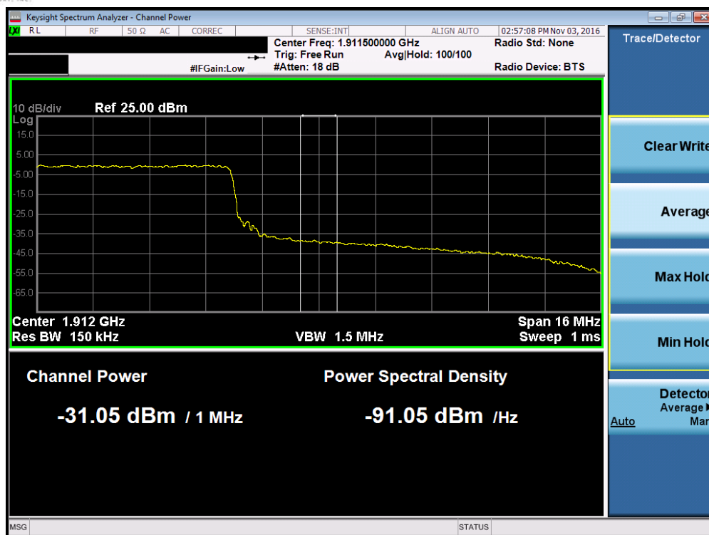
Plot 7-157. Upper Extended Band Edge Plot (Band 2 – 20.0MHz QPSK – RB Size 100)
