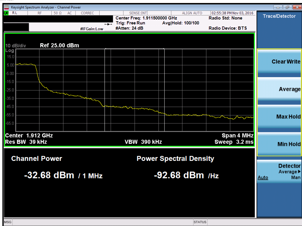
Plot 7-137. Upper Extended Band Edge Plot (Band 2 – 1.4MHz QPSK – RB Size 6)
