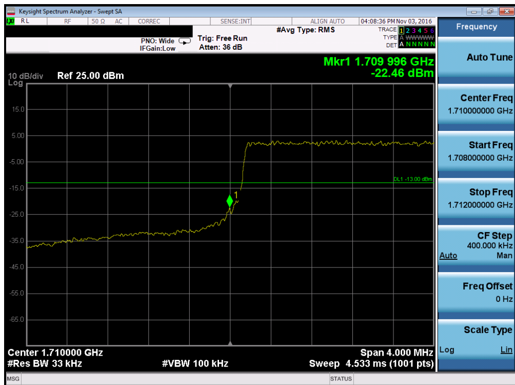
Plot 7-114. Lower Band Edge Plot (Band 4 – 3.0MHz QPSK – RB Size 15)
