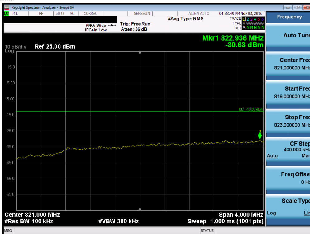
Plot 7-105. Lower Extended Band Edge Plot (Band 5 – 5.0MHz QPSK – RB Size 25)
