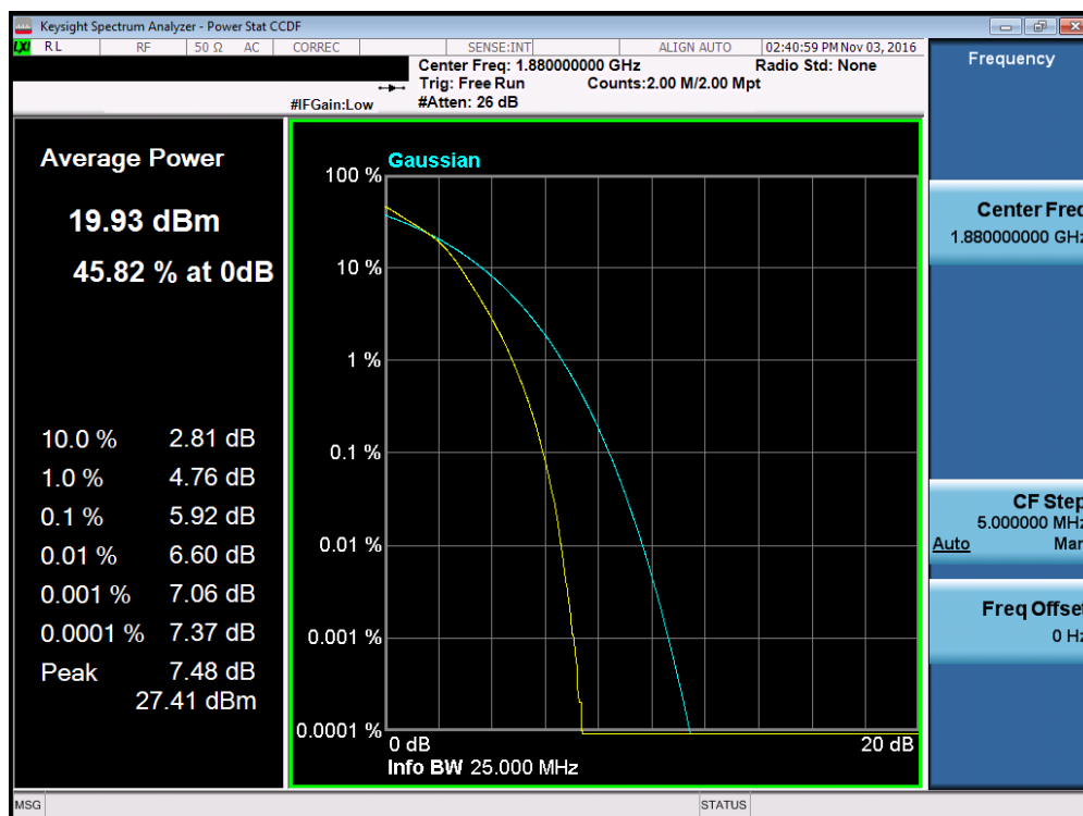
Plot 7-177. PAR Plot (Band 2 – 20.0MHz 16-QAM – RB Size 100)
