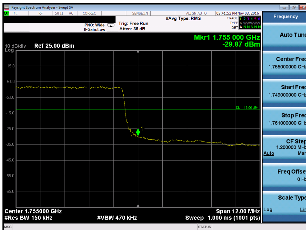
Plot 7-128. Upper Band Edge Plot (Band 4 – 15.0MHz QPSK – RB Size 75)
