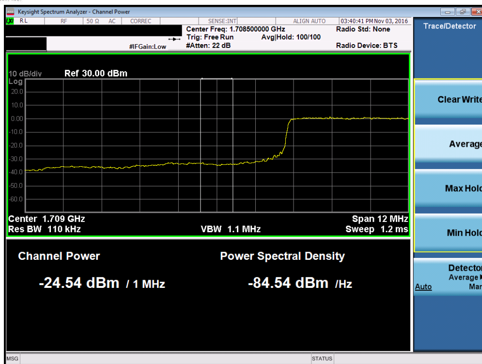
Plot 7-127. Lower Extended Band Edge Plot (Band 4 – 15.0MHz QPSK – RB Size 75)
