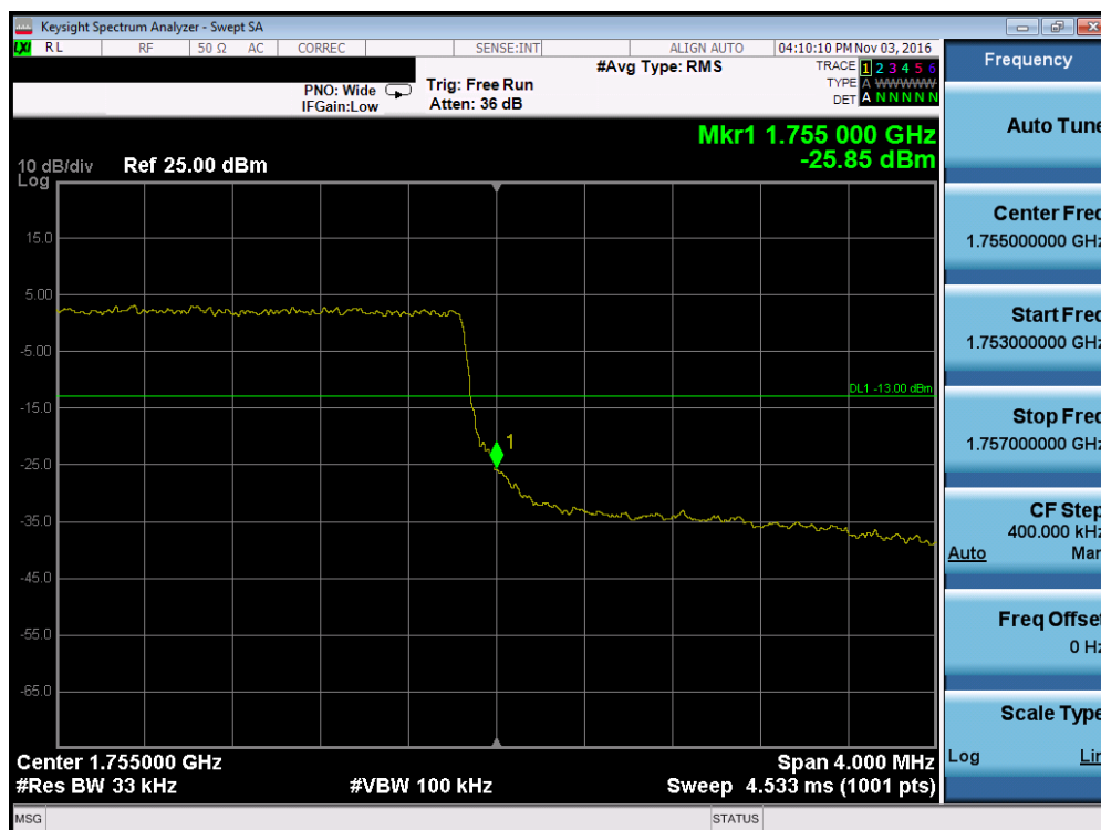
Plot 7-116. Upper Band Edge Plot (Band 4 – 3.0MHz QPSK – RB Size 15)
