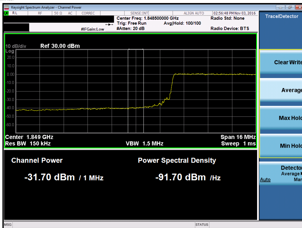
Plot 7-155. Lower Extended Band Edge Plot (Band 2 – 20.0MHz QPSK – RB Size 100)
