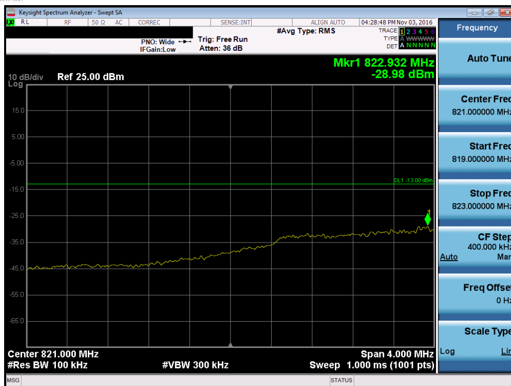
Plot 7-101. Lower Extended Band Edge Plot (Band 5 – 3.0MHz QPSK – RB Size 15)
