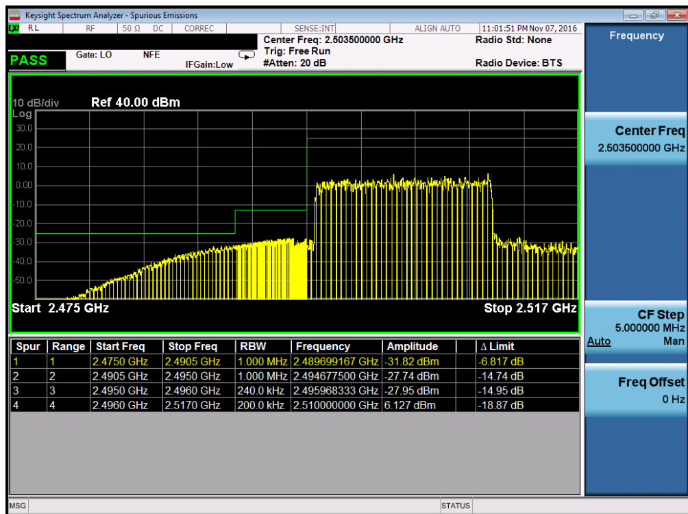
Plot 7-162. Lower ACP Plot (Band 41 – 15.0MHz QPSK – RB Size 75)
