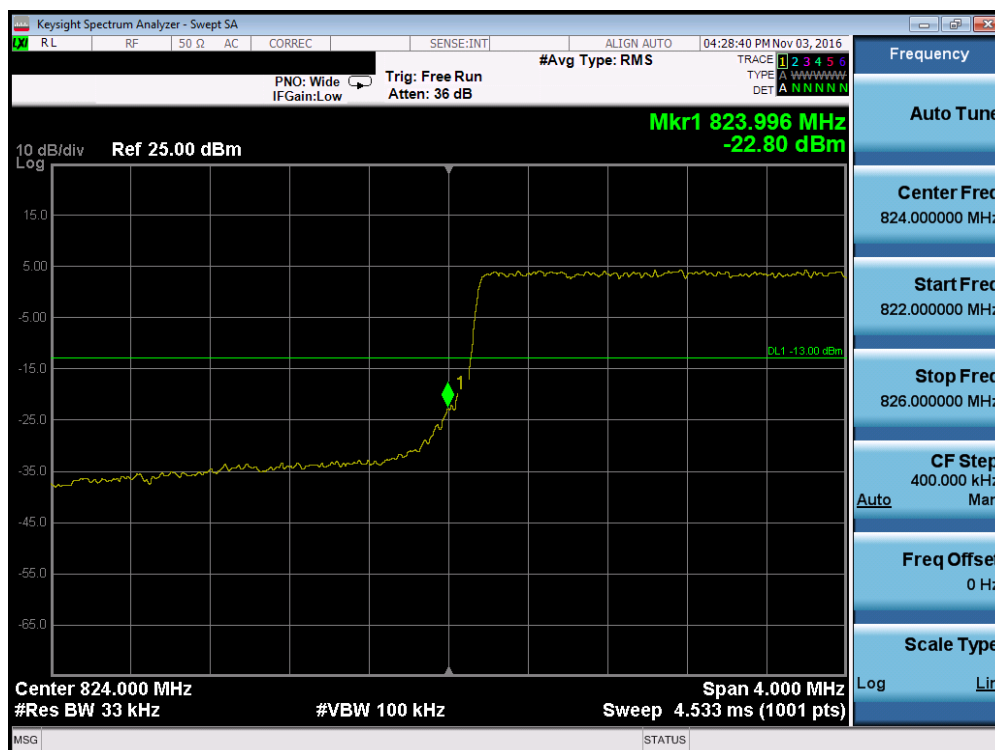
Plot 7-100. Lower Band Edge Plot (Band 5 – 3.0MHz QPSK – RB Size 15)
