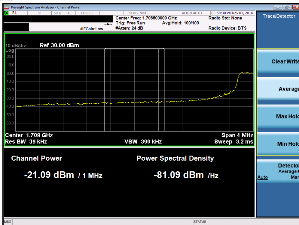
Plot 7-119. Lower Extended Band Edge Plot (Band 4 – 5.0MHz QPSK – RB Size 25)
