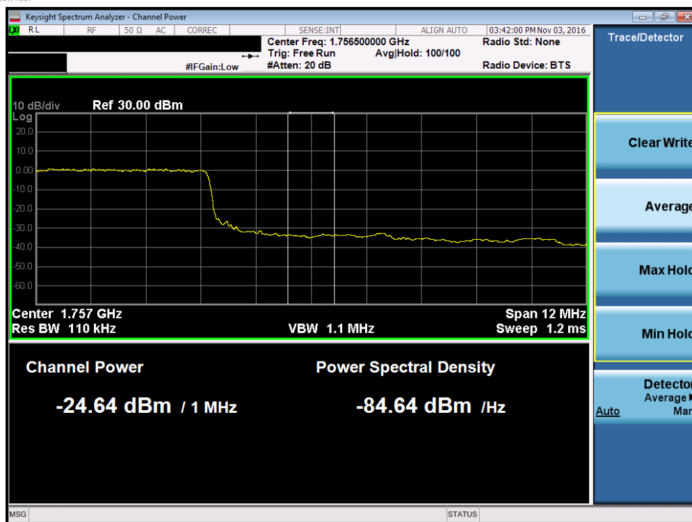
Plot 7-129. Upper Extended Band Edge Plot (Band 4 – 15.0MHz QPSK – RB Size 75)
