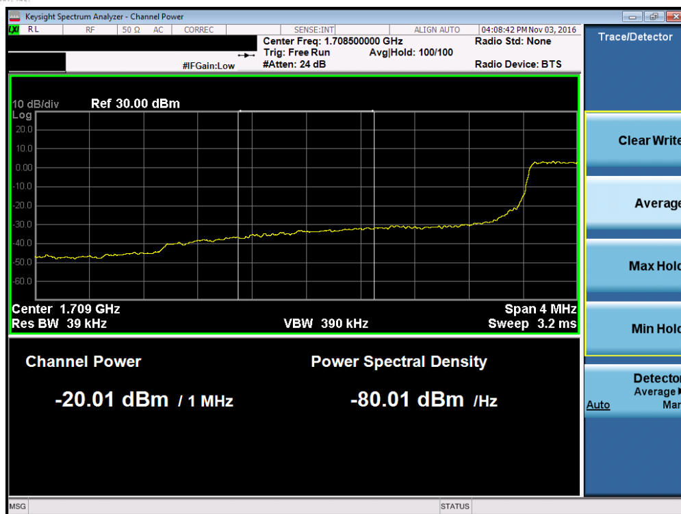
Plot 7-115. Lower Extended Band Edge Plot (Band 4 – 3.0MHz QPSK – RB Size 15)
