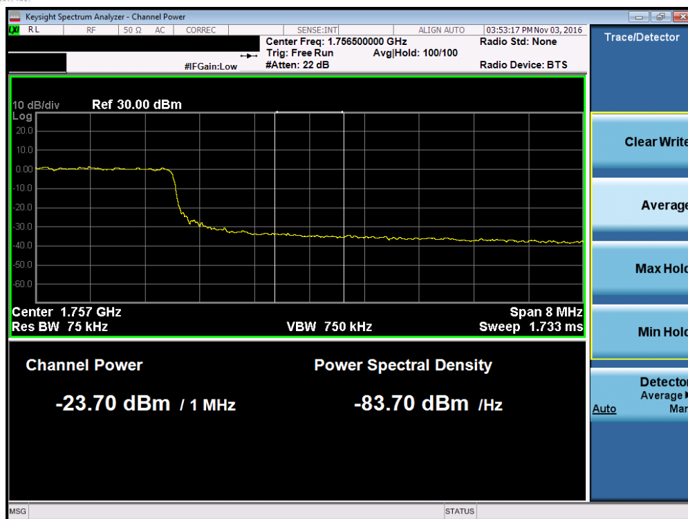
Plot 7-125. Upper Extended Band Edge Plot (Band 4 – 10.0MHz QPSK – RB Size 50)
