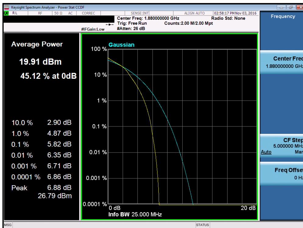
Plot 7-175. PAR Plot (Band 2 – 15.0MHz 16-QAM – RB Size 75)
