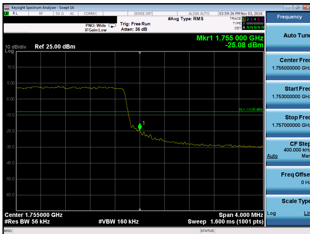
Plot 7-120. Upper Band Edge Plot (Band 4 – 5.0MHz QPSK – RB Size 25)
