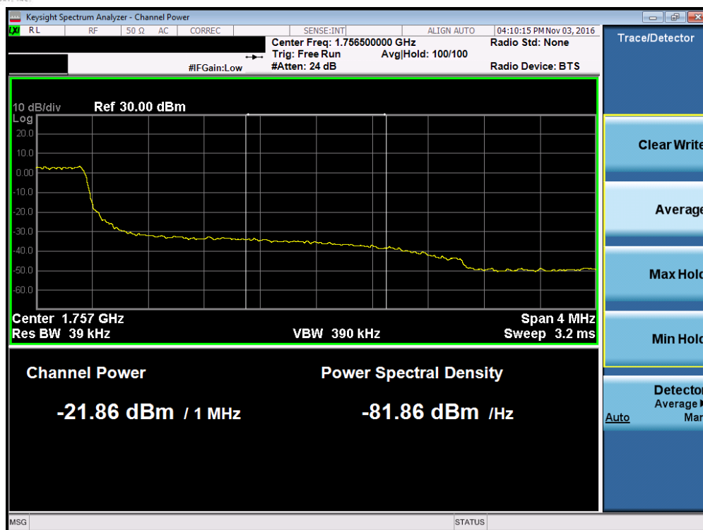
Plot 7-117. Upper Extended Band Edge Plot (Band 4 – 3.0MHz QPSK – RB Size 15)
