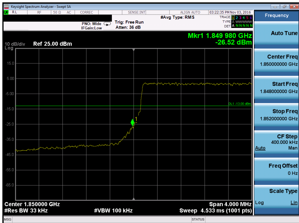
Plot 7-138. Lower Band Edge Plot (Band 2 – 3.0MHz QPSK – RB Size 15)
