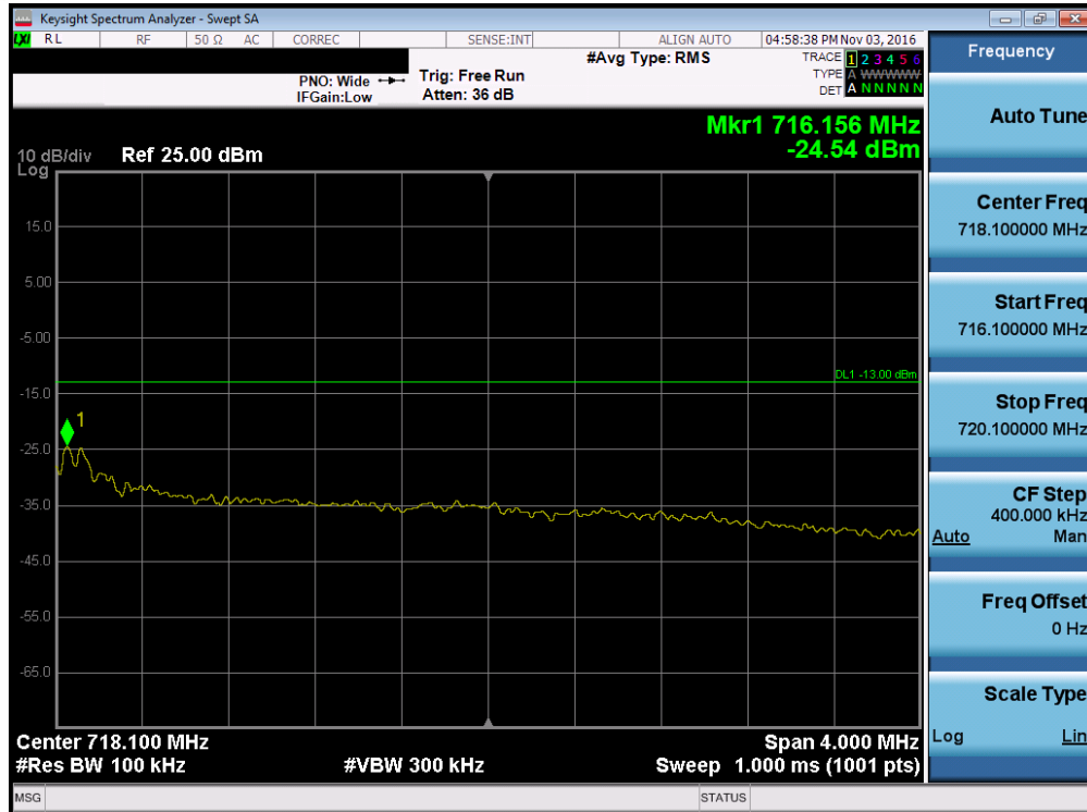
Plot 7-93. Upper Extended Band Edge Plot (Band 17 – 5.0MHz QPSK – RB Size 25)
