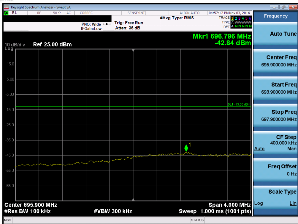
Plot 7-91. Lower Extended Band Edge Plot (Band 17 - 5.0MHz QPSK - RB Size 25)
