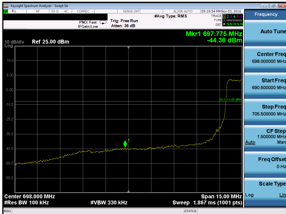
Plot 7-94. Lower Band Edge Plot (Band 17 – 10.0MHz QPSK – RB Size 50)
