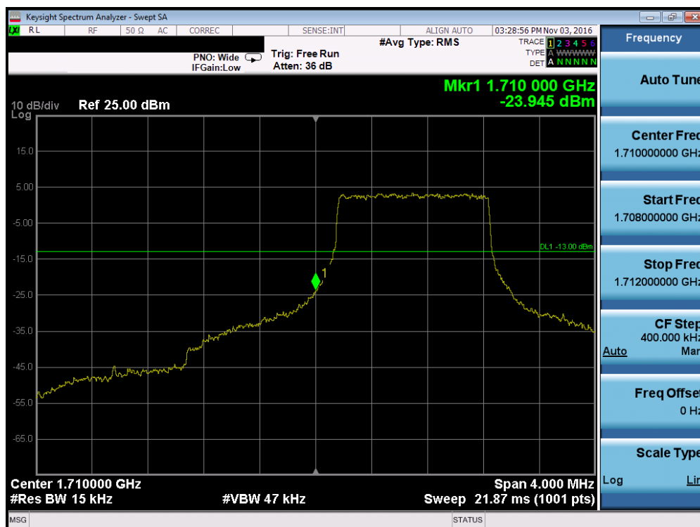
Plot 7-110. Lower Band Edge Plot (Band 4 – 1.4MHz QPSK – RB Size 6)
