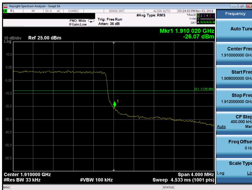
Plot 7-140. Upper Band Edge Plot (Band 2 – 3.0MHz QPSK – RB Size 15)
