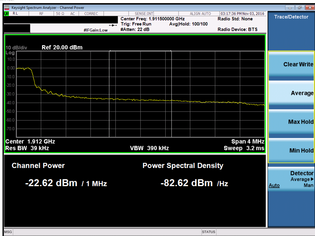
Plot 7-145. Upper Extended Band Edge Plot (Band 2 – 5.0MHz QPSK – RB Size 25)
