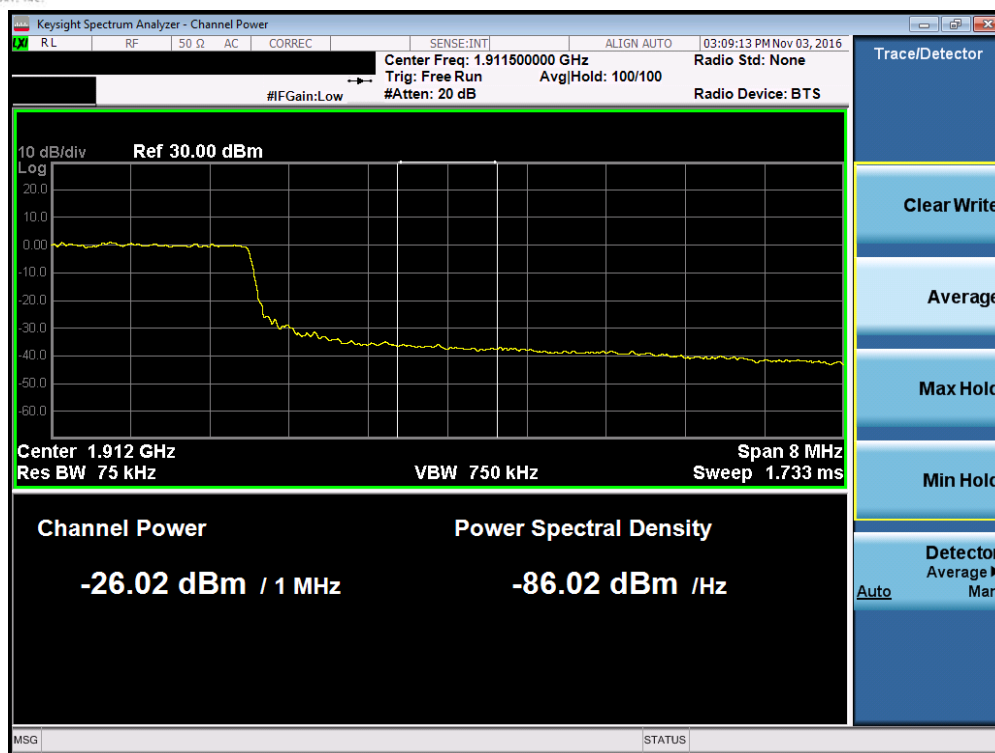
Plot 7-149. Upper Extended Band Edge Plot (Band 2 – 10.0MHz QPSK – RB Size 50)
