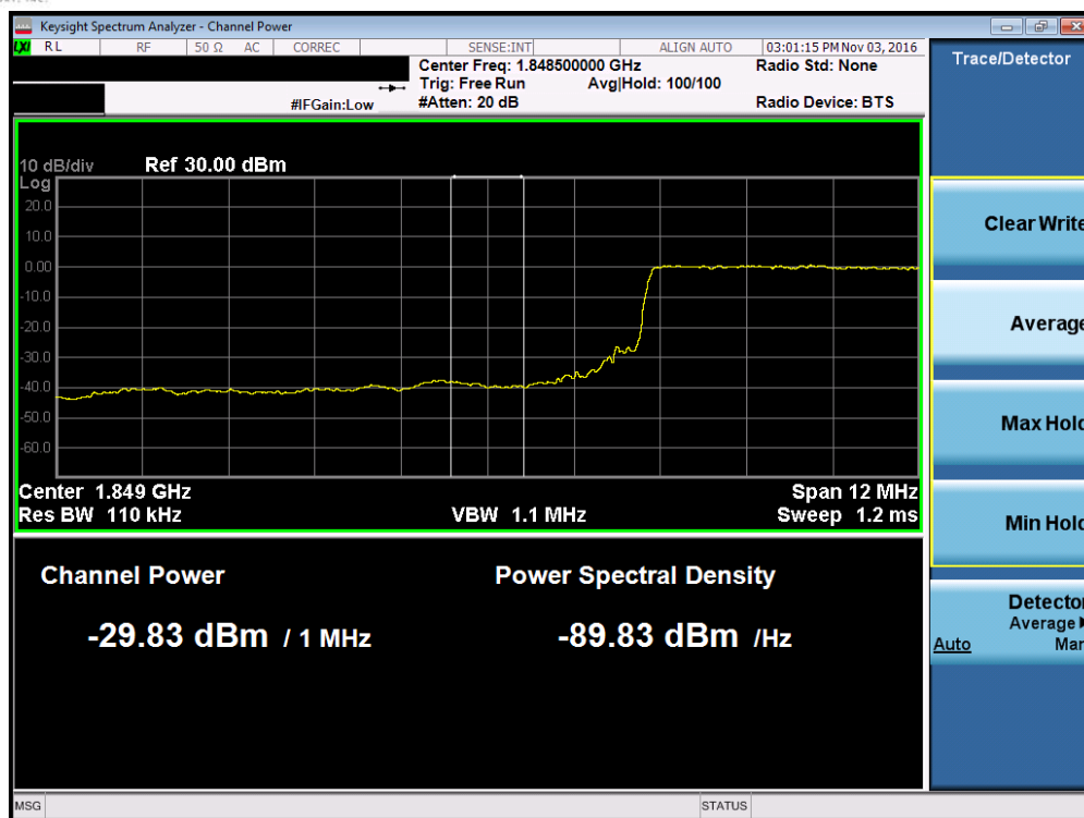
Plot 7-151. Lower Extended Band Edge Plot (Band 2 – 15.0MHz QPSK – RB Size 75)
