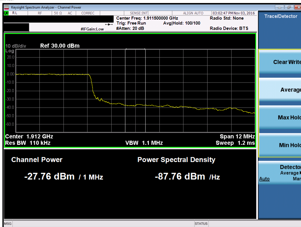
Plot 7-153. Upper Extended Band Edge Plot (Band 2 – 15.0MHz QPSK – RB Size 75)
