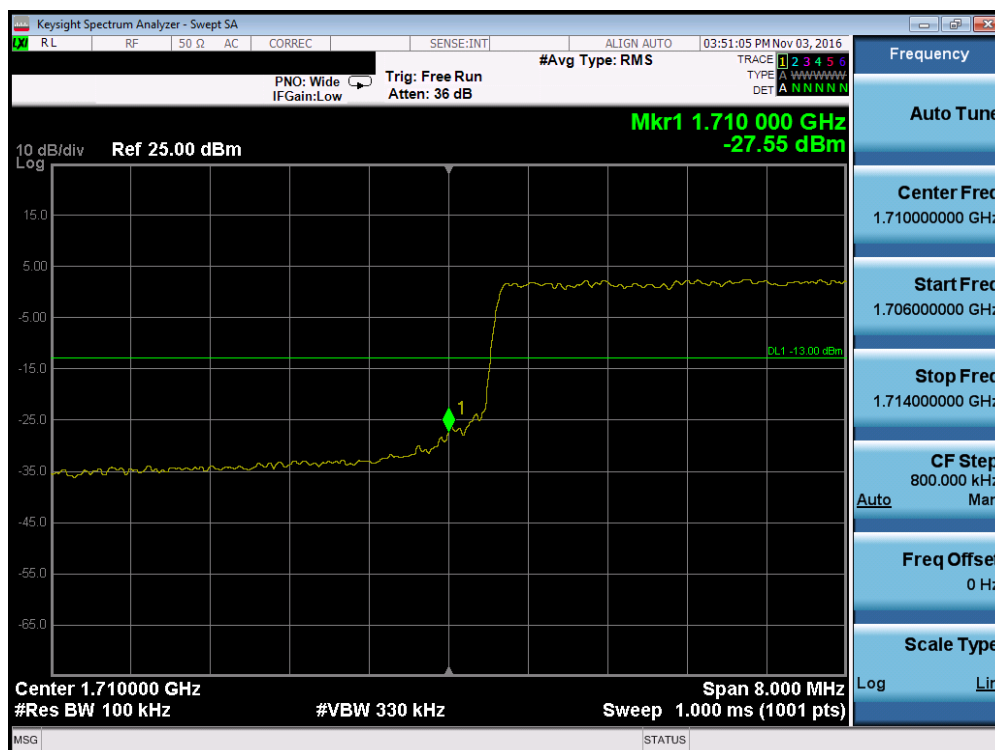
Plot 7-122. Lower Band Edge Plot (Band 4 – 10.0MHz QPSK – RB Size 50)
