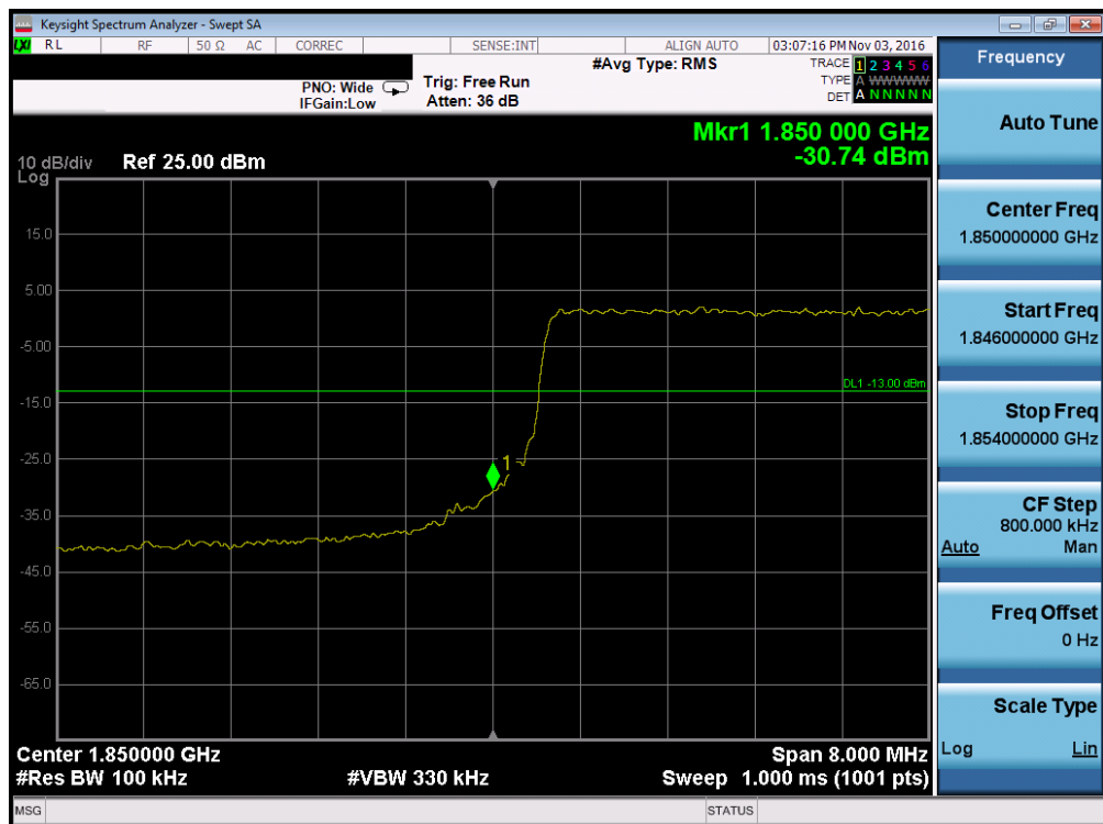
Plot 7-146. Lower Band Edge Plot (Band 2 – 10.0MHz QPSK – RB Size 50)
