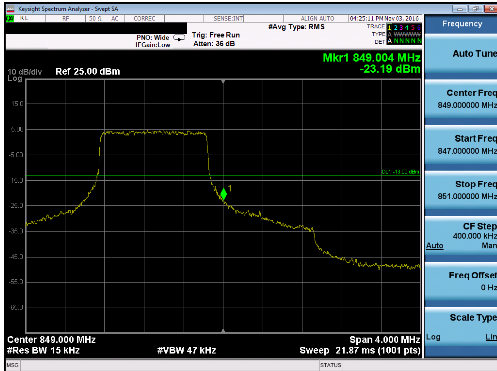
Plot 7-98. Upper Band Edge Plot (Band 5 – 1.4MHz QPSK – RB Size 6)
