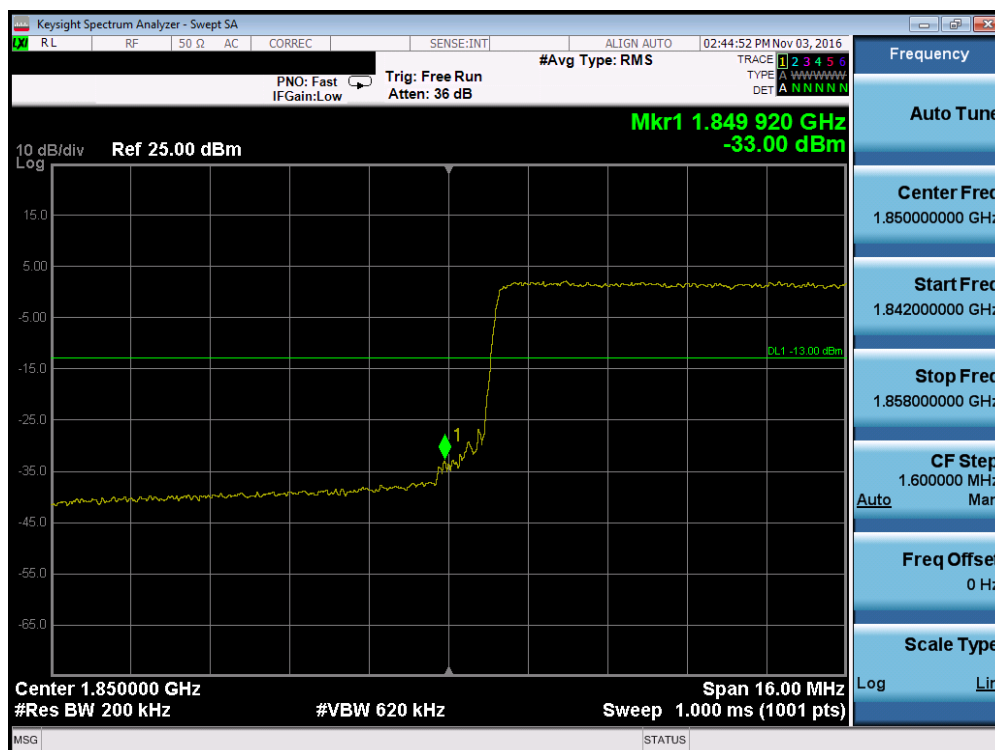
Plot 7-154. Lower Band Edge Plot (Band 2 – 20.0MHz QPSK – RB Size 100)
