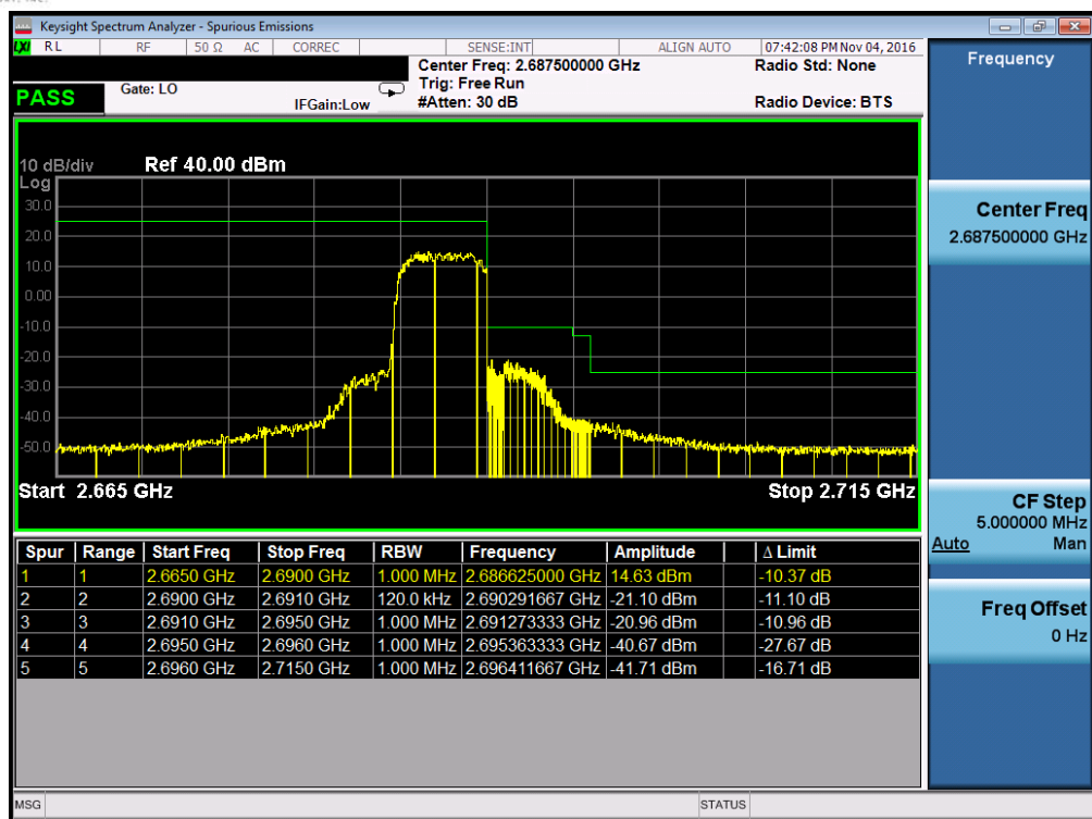
Plot 7-159. Upper ACP Plot (Band 41 – 5.0MHz QPSK – RB Size 25)
