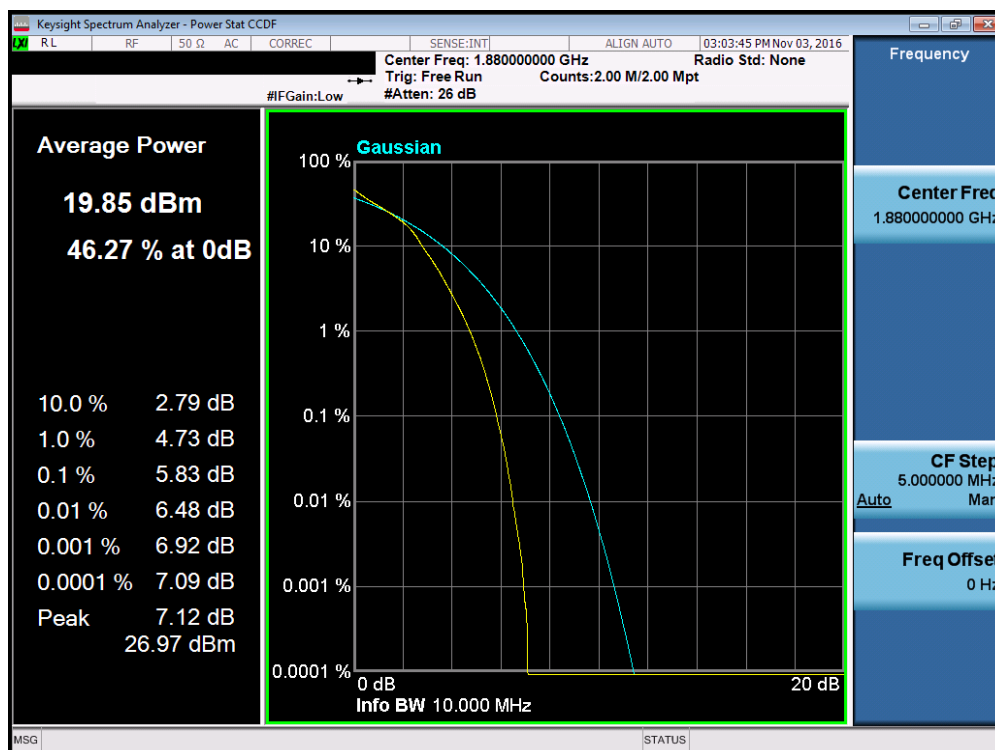
Plot 7-173. PAR Plot (Band 2 – 10.0MHz 16-QAM – RB Size 50)
