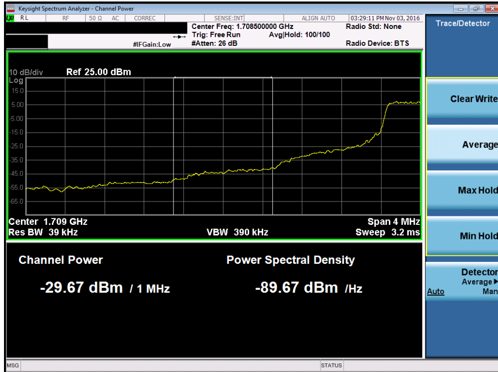
Plot 7-111. Lower Extended Band Edge Plot (Band 4 – 1.4MHz QPSK – RB Size 6)
