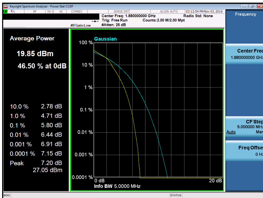
Plot 7-171. PAR Plot (Band 2 – 5.0MHz 16-QAM – RB Size 25)
