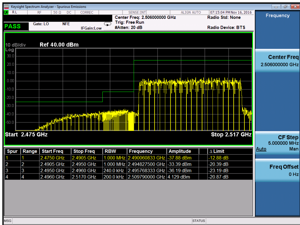
Plot 7-164. Lower ACP Plot (Band 41 – 20.0MHz QPSK – RB Size 100)
