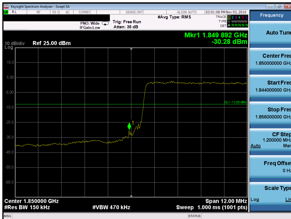
Plot 7-150. Lower Band Edge Plot (Band 2 – 15.0MHz QPSK – RB Size 75)
