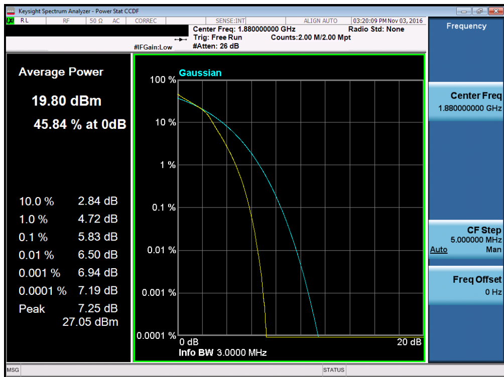
Plot 7-169. PAR Plot (Band 2 – 3.0MHz 16-QAM – RB Size 15)
