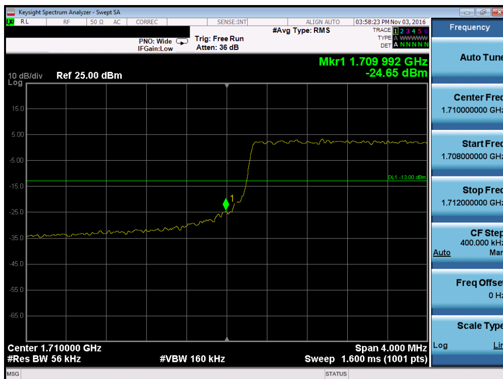
Plot 7-118. Lower Band Edge Plot (Band 4 – 5.0MHz QPSK – RB Size 25)
