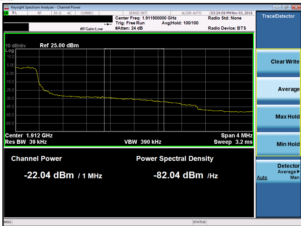
Plot 7-141. Upper Extended Band Edge Plot (Band 2 – 3.0MHz QPSK – RB Size 15)
