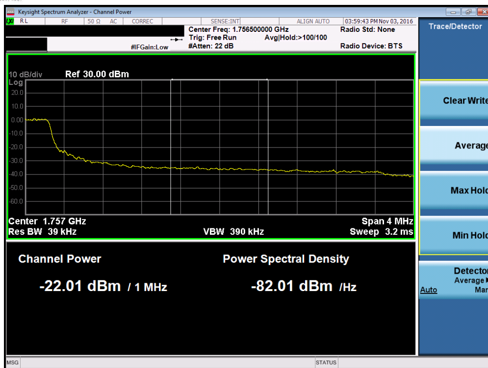
Plot 7-121. Upper Extended Band Edge Plot (Band 4 – 5.0MHz QPSK – RB Size 25)
