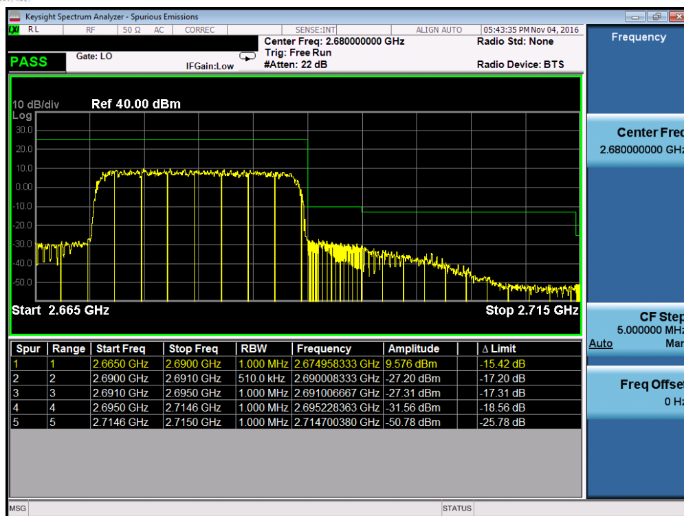
Plot 7-165. Upper ACP Plot (Band 41 – 20.0MHz QPSK – RB Size 100)
