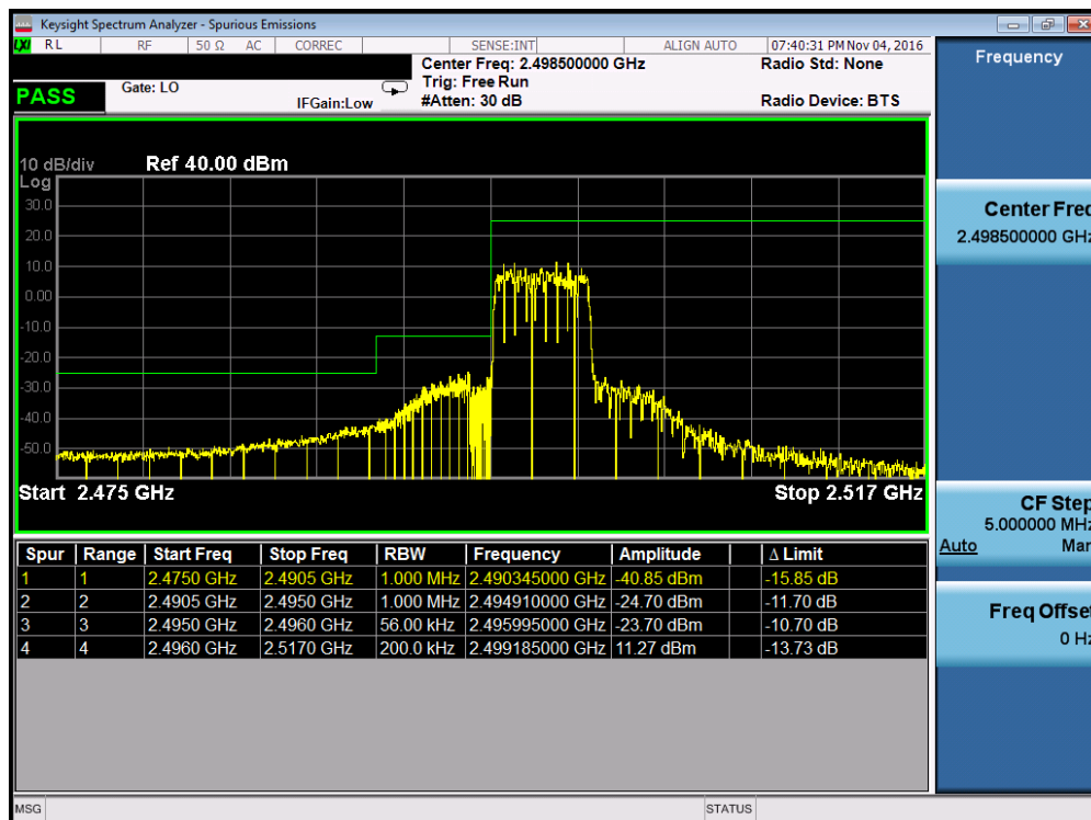
Plot 7-158. Lower ACP Plot (Band 41 – 5.0MHz QPSK – RB Size 25)
