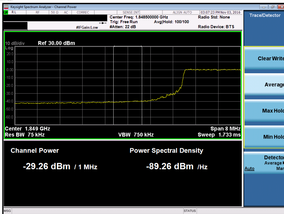
Plot 7-147. Lower Extended Band Edge Plot (Band 2 – 10.0MHz QPSK – RB Size 50)
