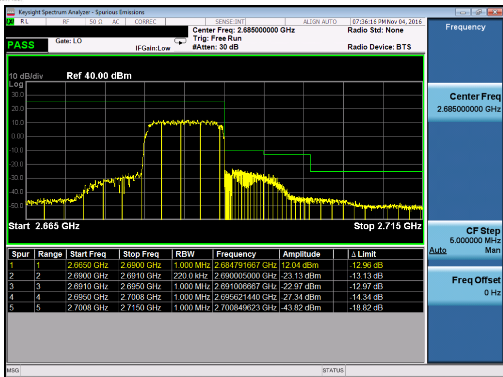
Plot 7-161. Upper ACP Plot (Band 41 – 10.0MHz QPSK – RB Size 50)
