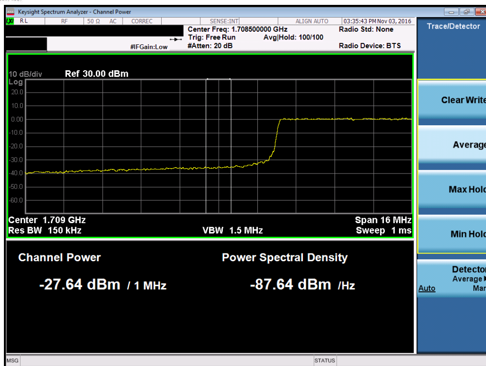
Plot 7-131. Lower Extended Band Edge Plot (Band 4 – 20.0MHz QPSK – RB Size 100)
