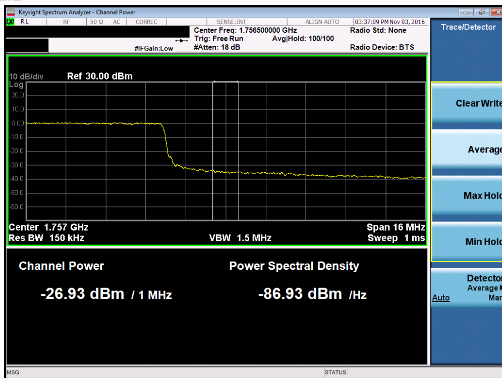
Plot 7-133. Upper Extended Band Edge Plot (Band 4 – 20.0MHz QPSK – RB Size 100)
