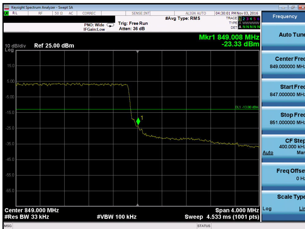
Plot 7-102. Upper Band Edge Plot (Band 5 – 3.0MHz QPSK – RB Size 15)
