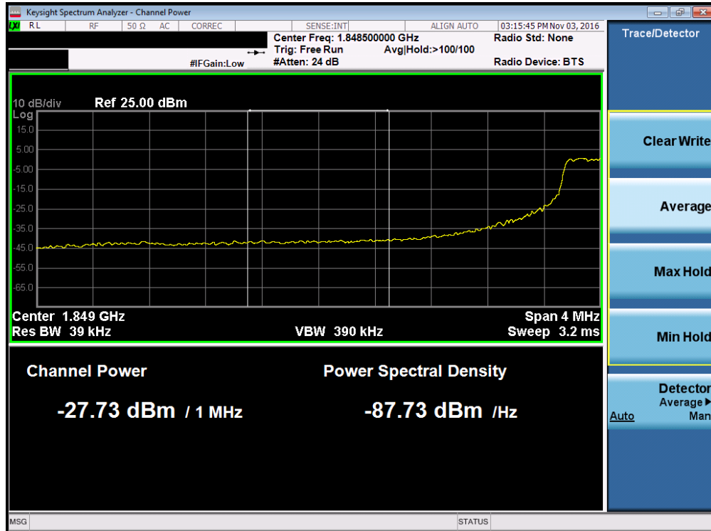
Plot 7-143. Lower Extended Band Edge Plot (Band 2 – 5.0MHz QPSK – RB Size 25)
