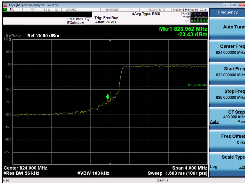
Plot 7-104. Lower Band Edge Plot (Band 5 – 5.0MHz QPSK – RB Size 25)
