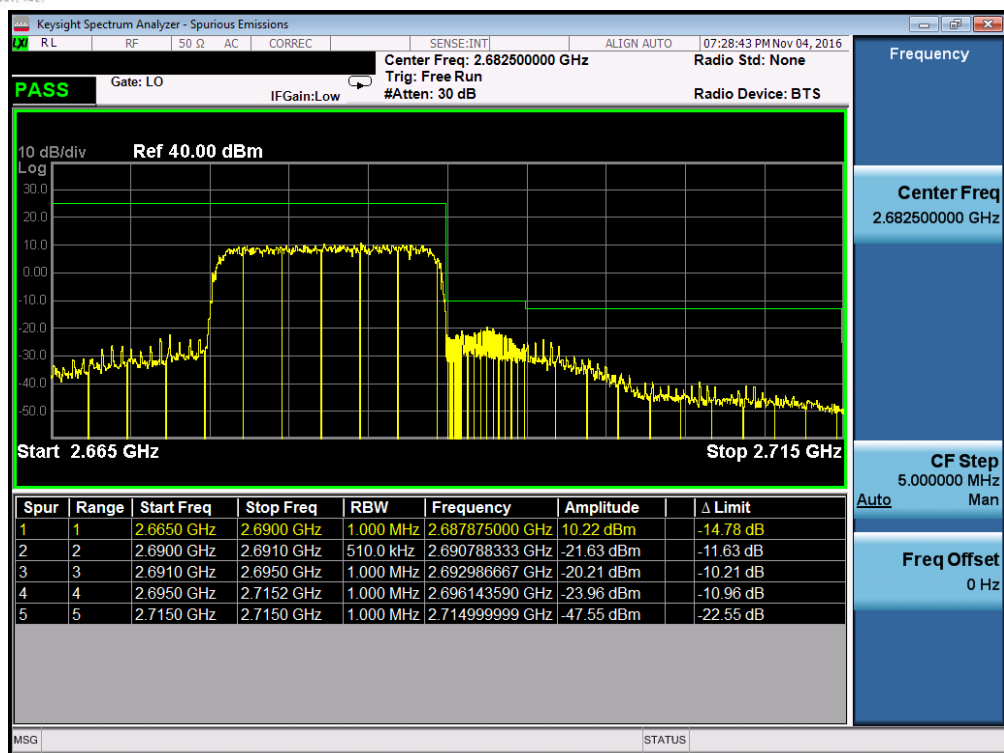
Plot 7-163. Upper ACP Plot (Band 41 – 15.0MHz QPSK – RB Size 75)
