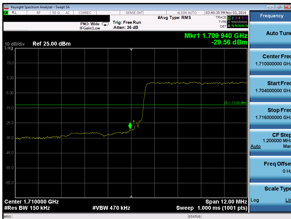
Plot 7-126. Lower Band Edge Plot (Band 4 – 15.0MHz QPSK – RB Size 75)
