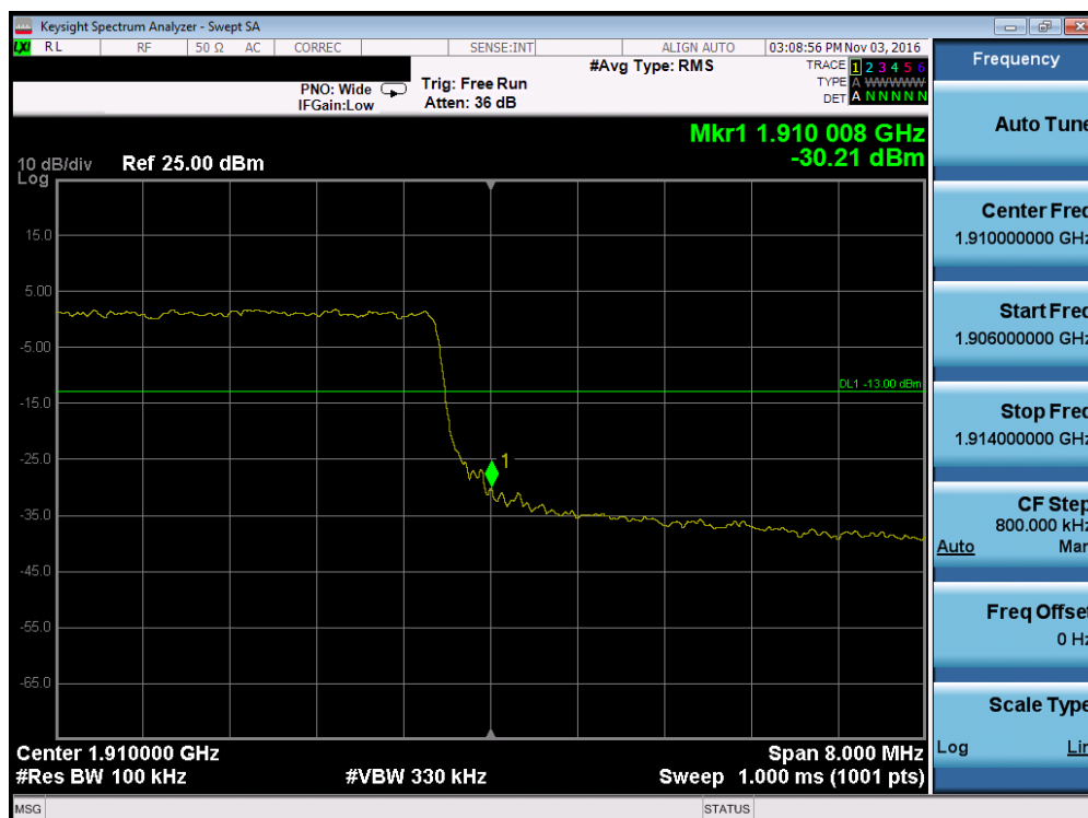
Plot 7-148. Upper Band Edge Plot (Band 2 – 10.0MHz QPSK – RB Size 50)
