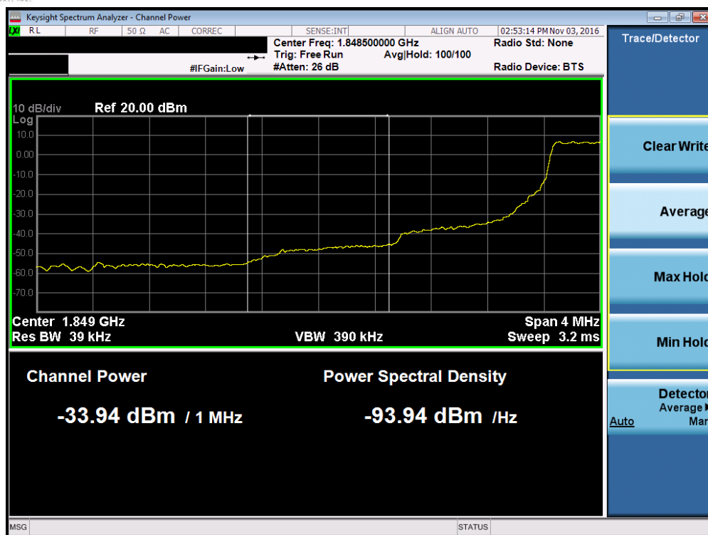
Plot 7-135. Lower Extended Band Edge Plot (Band 2 – 1.4MHz QPSK – RB Size 6)
