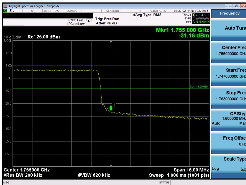
Plot 7-132. Upper Band Edge Plot (Band 4 – 20.0MHz QPSK – RB Size 100)
