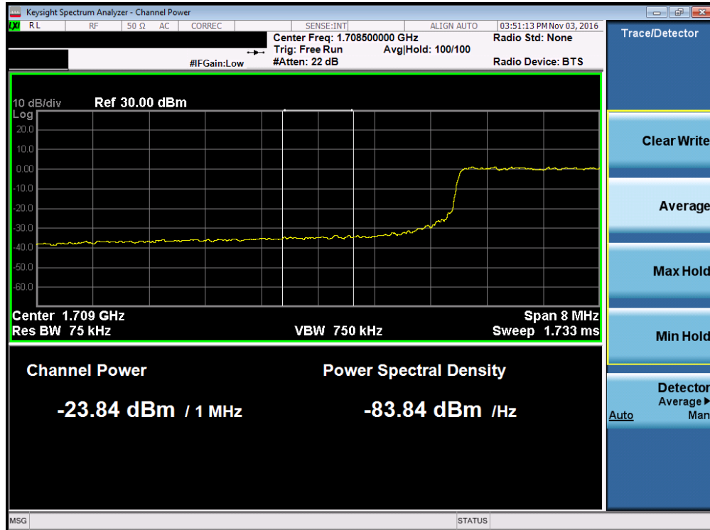
Plot 7-123. Lower Extended Band Edge Plot (Band 4 – 10.0MHz QPSK – RB Size 50)
