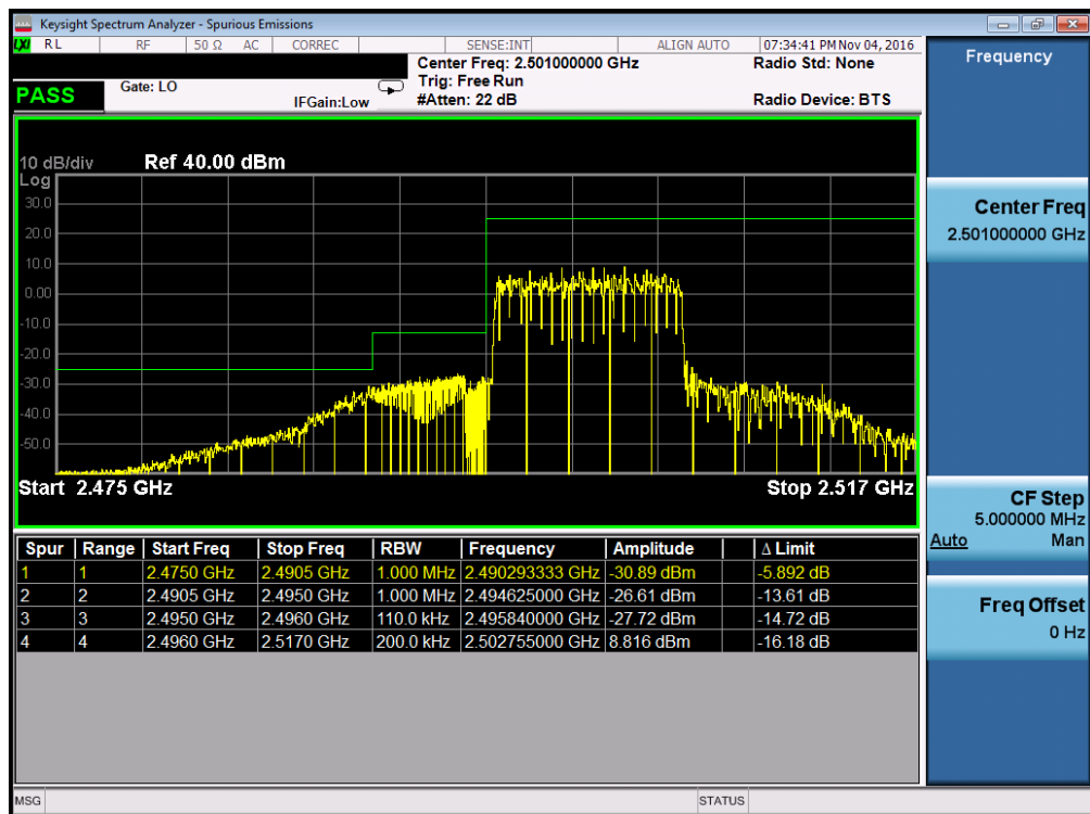
Plot 7-160. Lower ACP Plot (Band 41 – 10.0MHz QPSK – RB Size 50)
