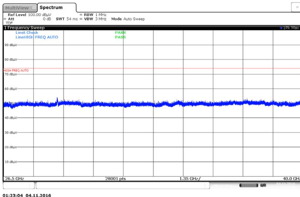
Plot 7-88. Radiated Spurious Plot above 18GHz (802.11a – Ant. Pol. H)
