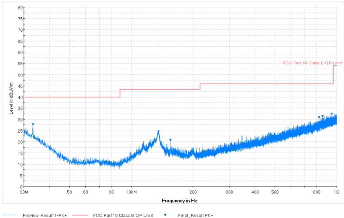
Plot 7-109. Radiated Spurious Plot below 1GHz (802.11a – U3 Ch. 157, Ant. Pol. H)
