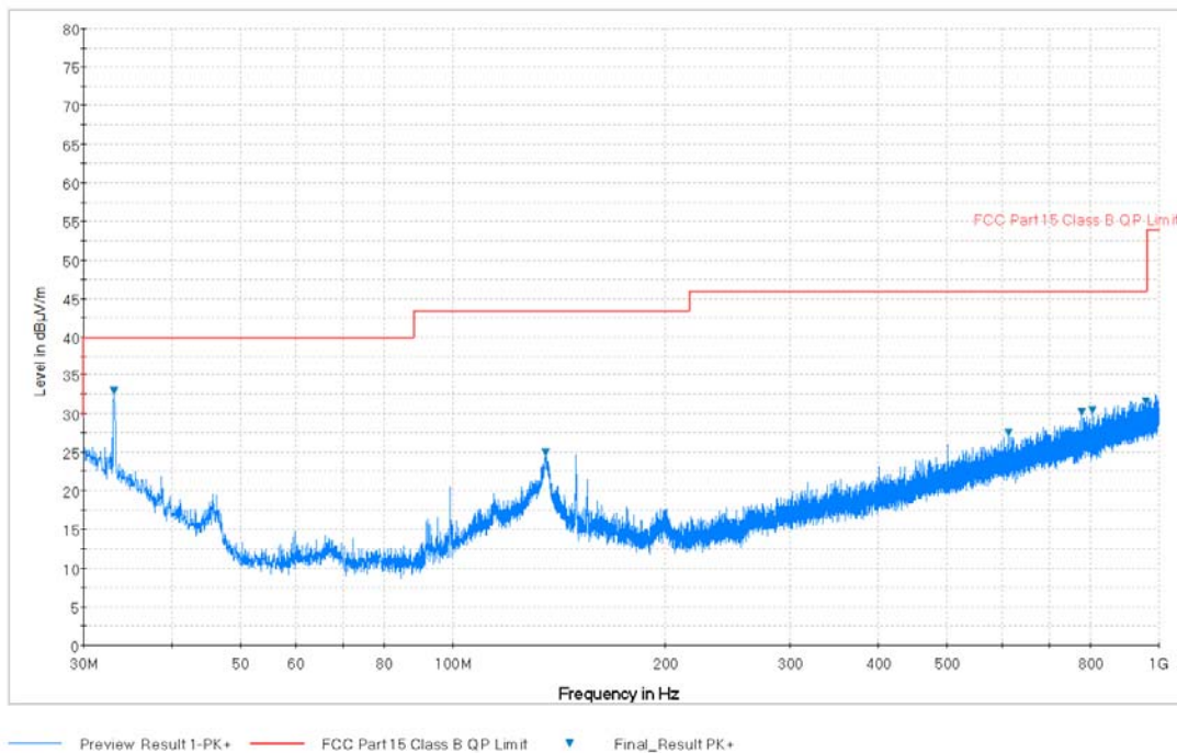
Plot 7-110. Radiated Spurious Plot below 1GHz (802.11a – U3 Ch. 157, Ant. Pol. V)
