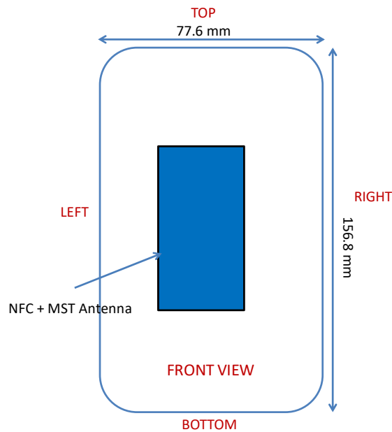
Figure F-2 NFC and MST Antenna Locations
