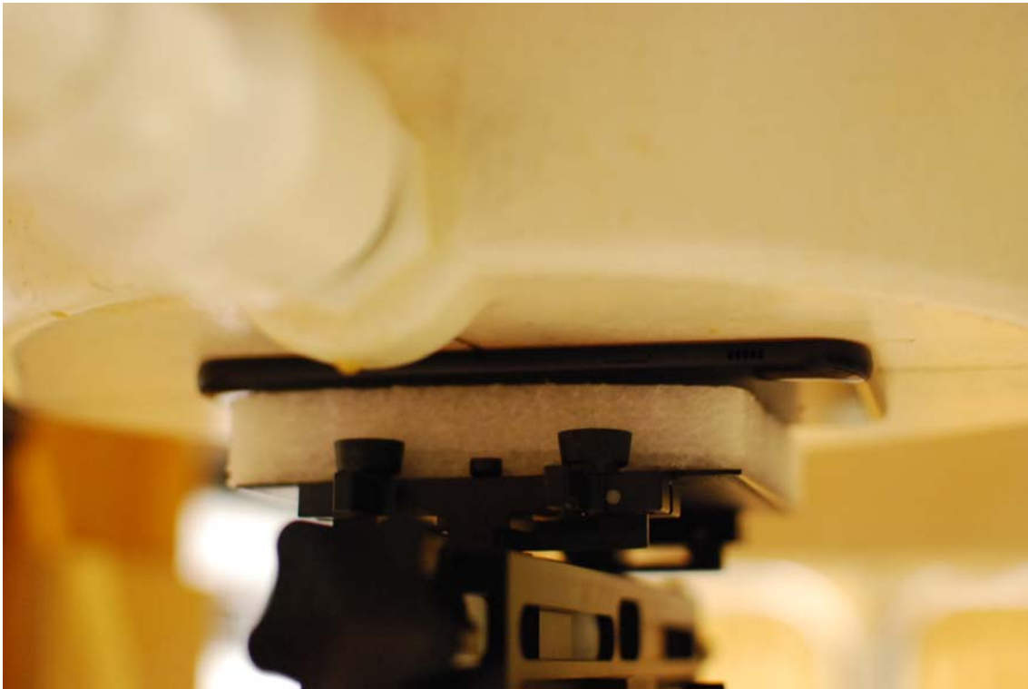
SAR Test Setup Photo 7: Front Side at 0 mm
