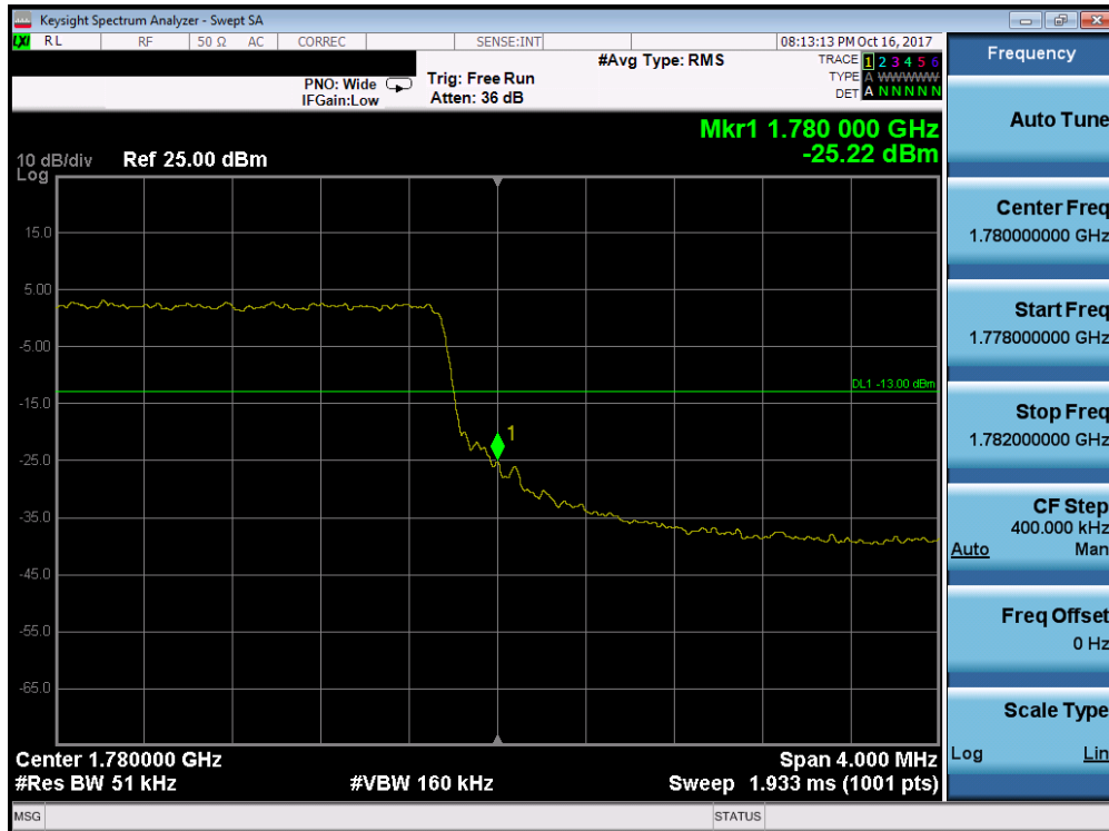
Plot 7-176. Upper Band Edge Plot (Band 66 - 5.0MHz QPSK - Full RB Configuration)
