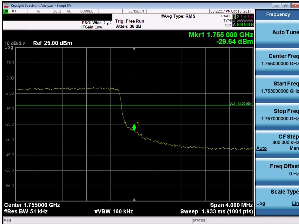
Plot 7-174. Upper Band Edge Plot (Band 4 - 5.0MHz QPSK - Full RB Configuration)
