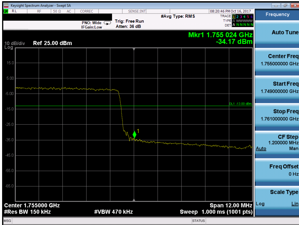
Plot 7-186. Upper Band Edge Plot (Band 4 - 15.0MHz QPSK - Full RB Configuration)
