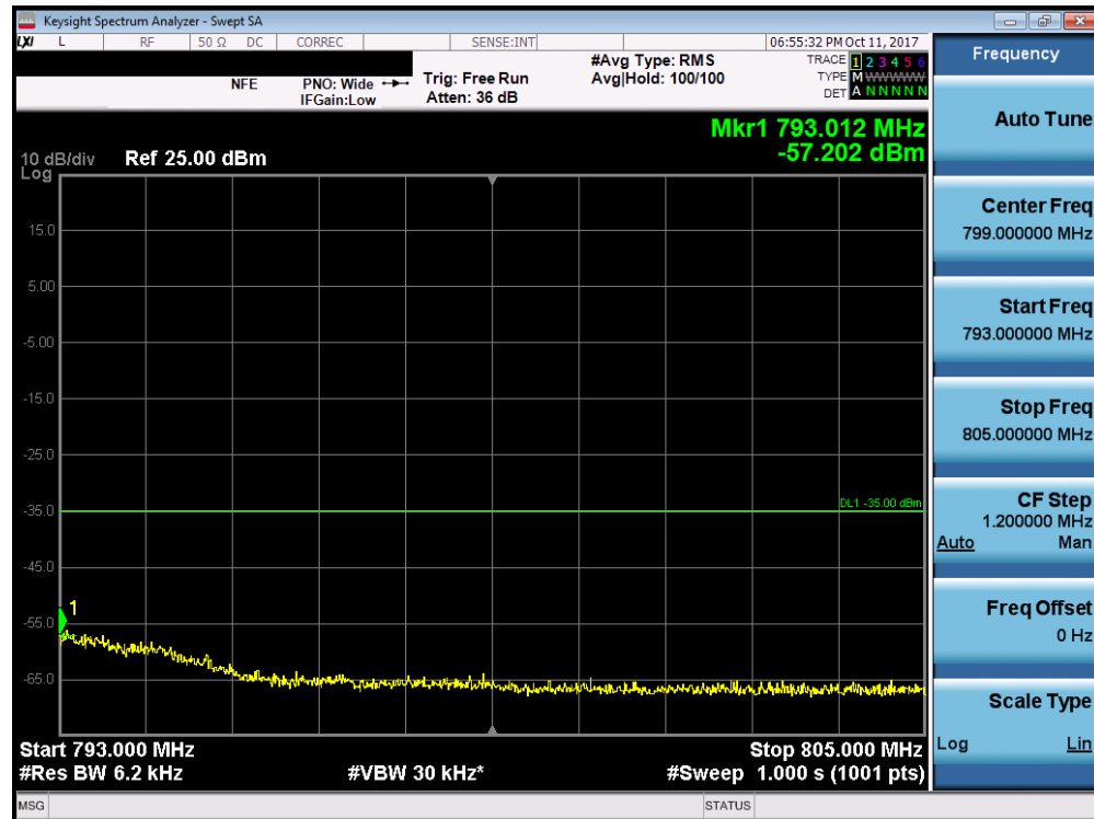
Plot 7-145. Upper Emission Mask Edge Plot (Band 13 - 5.0MHz QPSK - Full RB Configuration)
