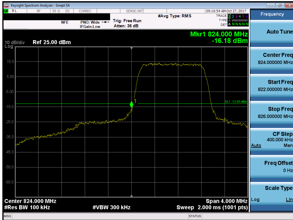
Plot 7-150. Lower Band Edge Plot (Band 5/26 - 1.4MHz QPSK - Full RB Configuration)
