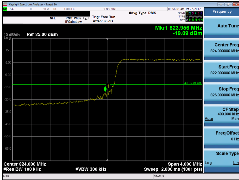
Plot 7-154. Lower Band Edge Plot (Band 5/26 – 5.0MHz QPSK - Full RB Configuration)
