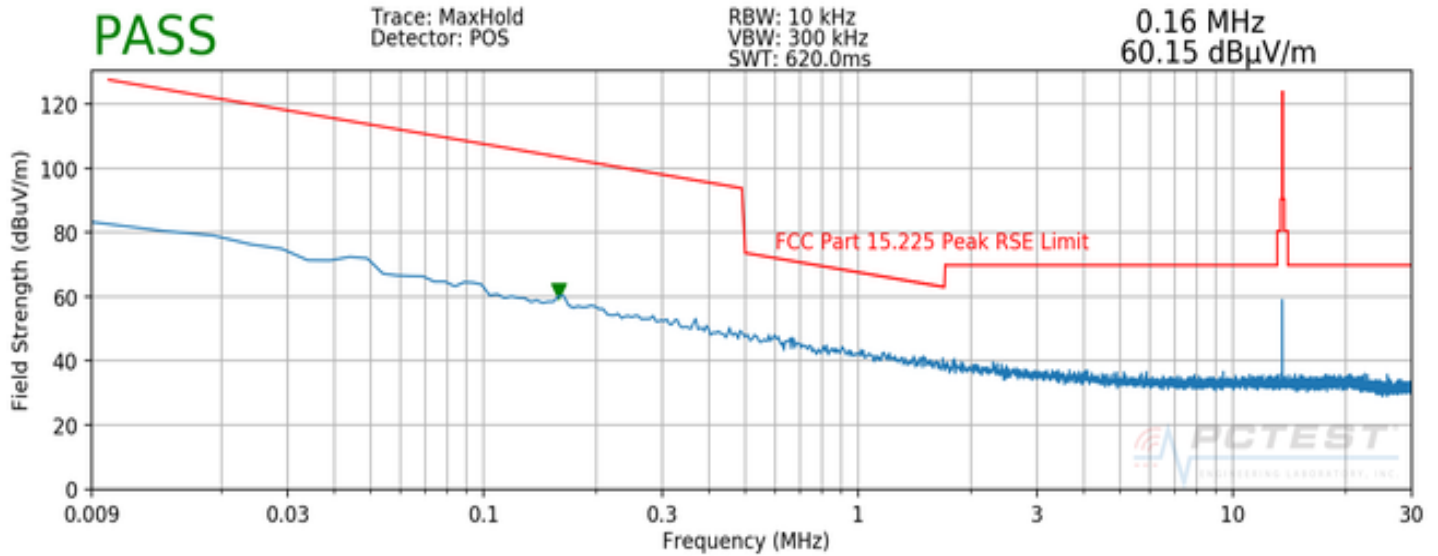
Plot 7-3. Radiated Spurious Plot 9kHz – 30MHz (Pol. Z)
