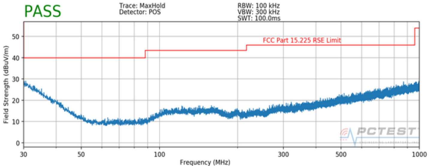
Plot 7-4. Radiated Spurious Plot 30MHz – 1GHz (Pol. H)
