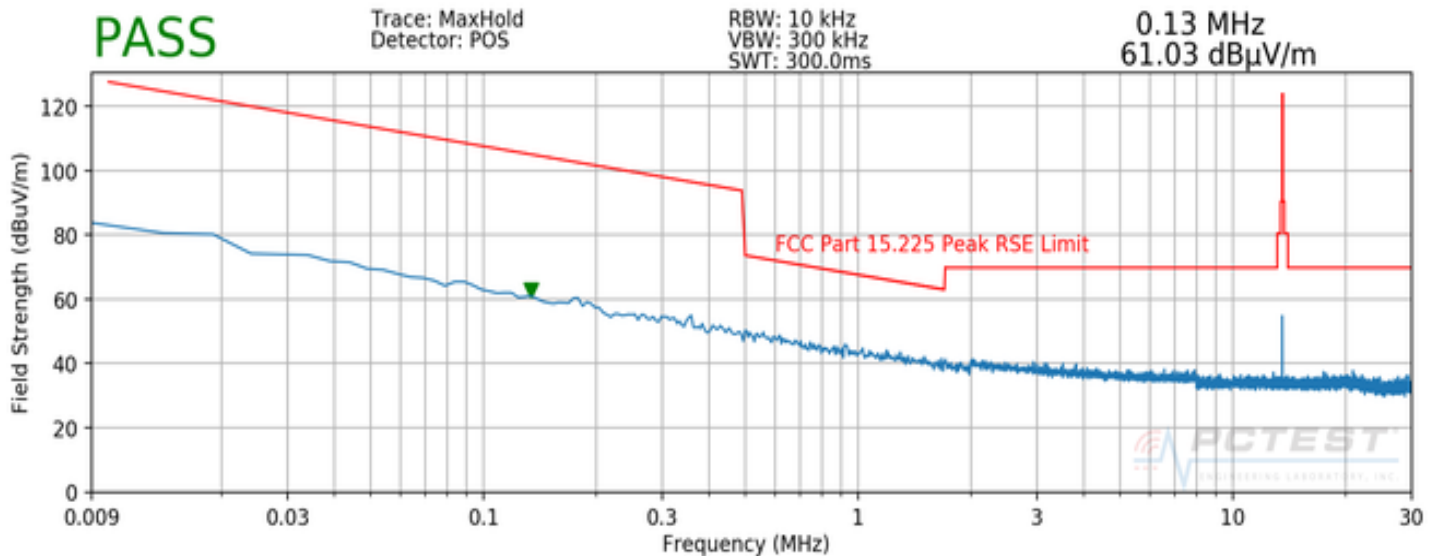
Plot 7-2. Radiated Spurious Plot 9kHz – 30MHz (Pol. Y)
