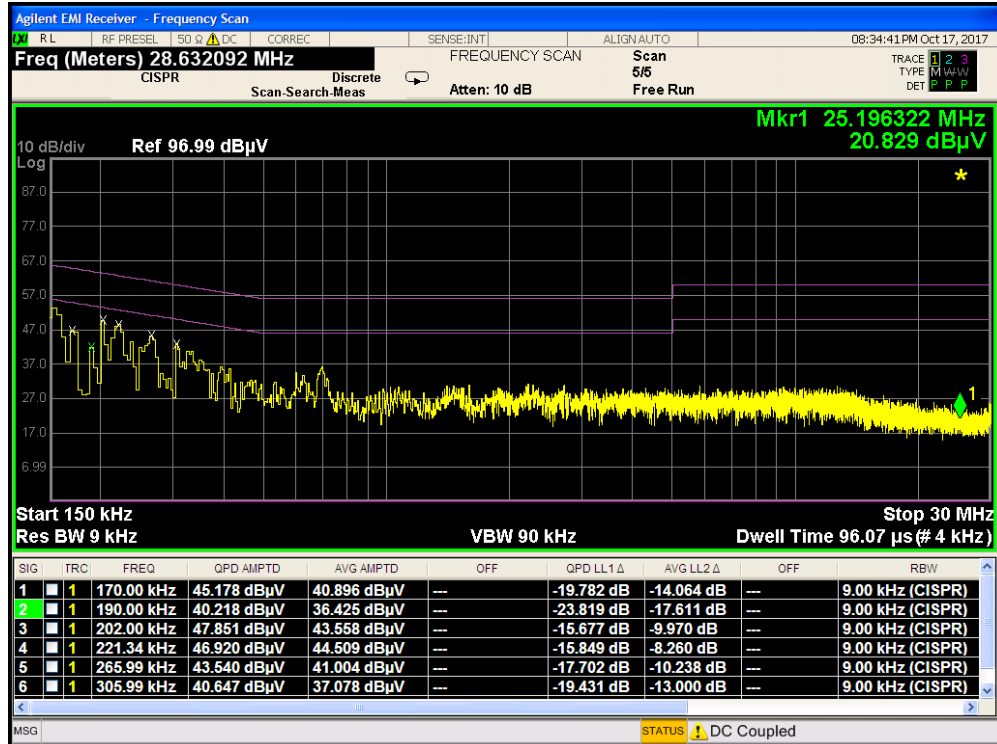
Plot 7-8. Line-Conducted Test Plot (L1) - Terminated in 50Ω
