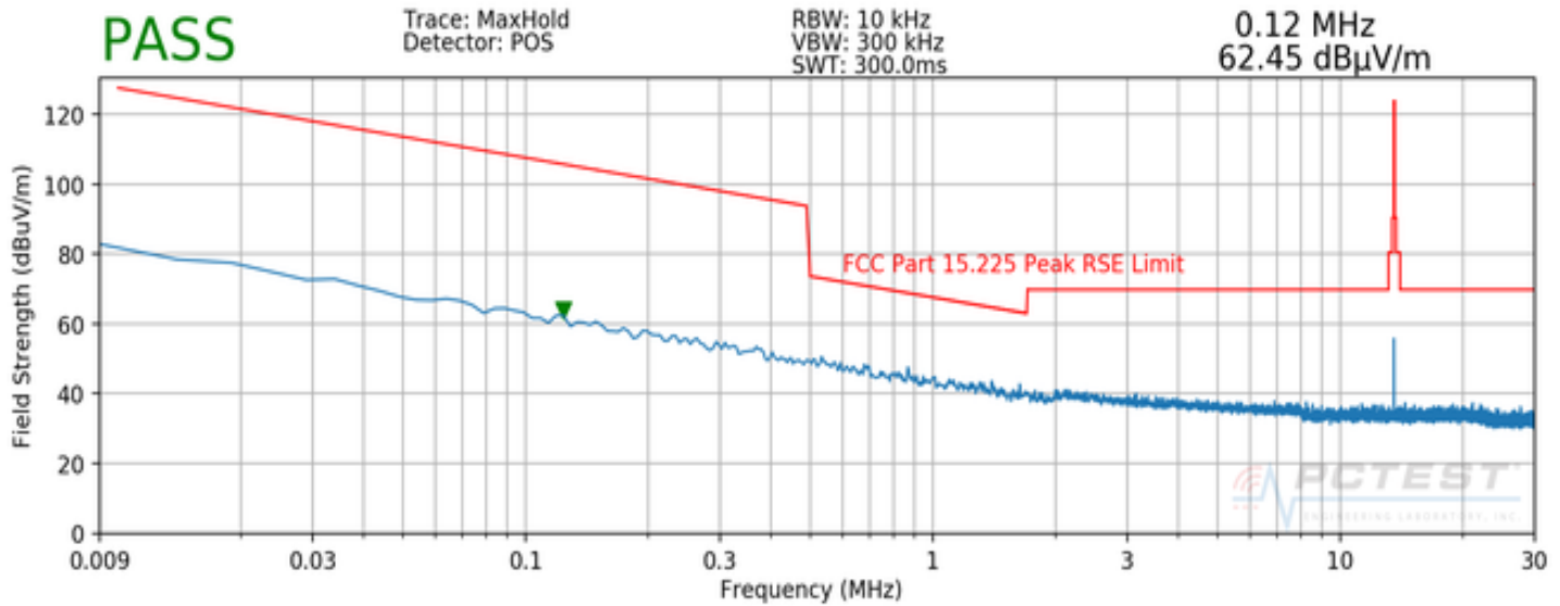
Plot 7-1. Radiated Spurious Plot 9kHz – 30MHz (Pol. X)
