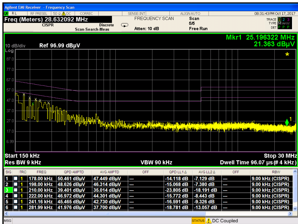
Plot 7-9. Line-Conducted Test Plot (N) - Terminated in 50Ω
