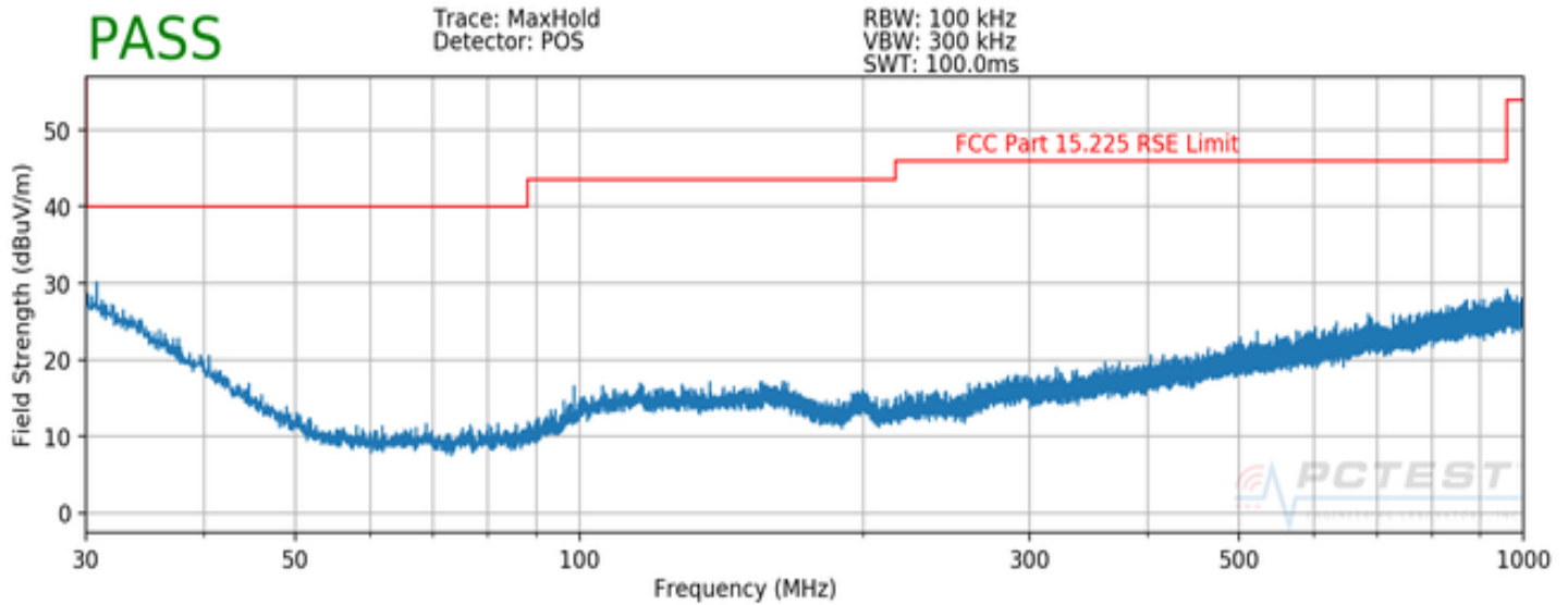
Plot 7-5. Radiated Spurious Plot 30MHz – 1GHz (Pol. V)
