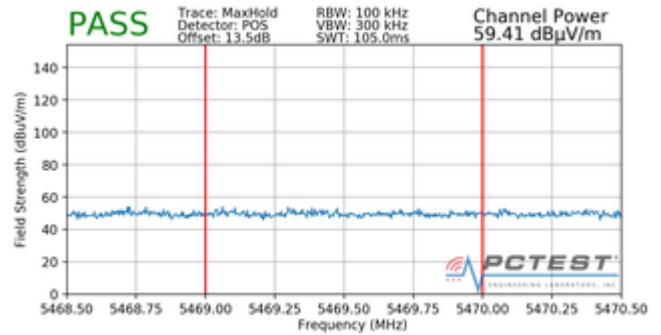
Plot 7-95. Radiated Lower Band Edge Plot (Peak – UNII Band 2C)
