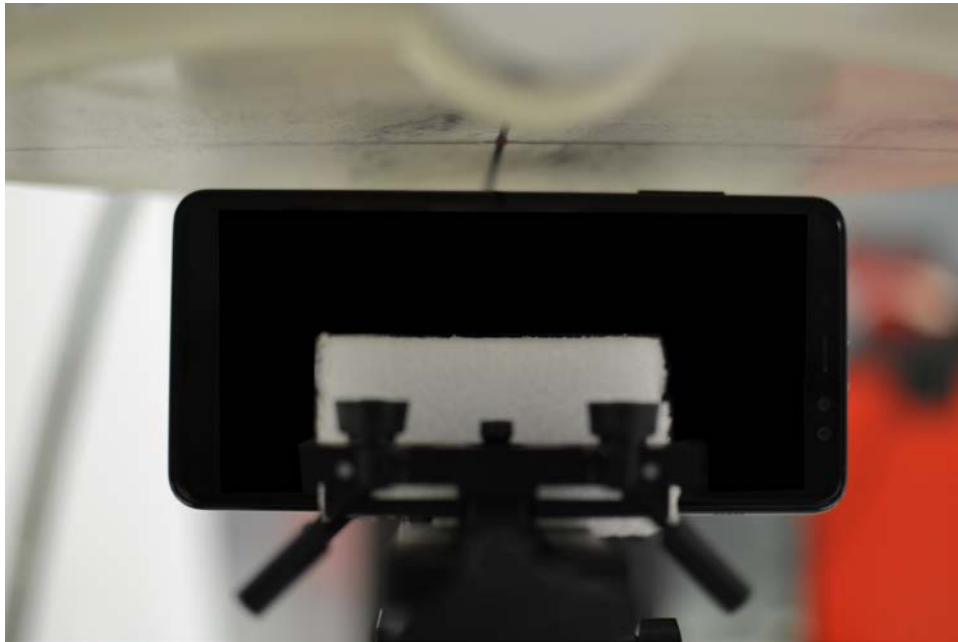
SAR Test Setup Photo 18: Left at 1.0 cm
