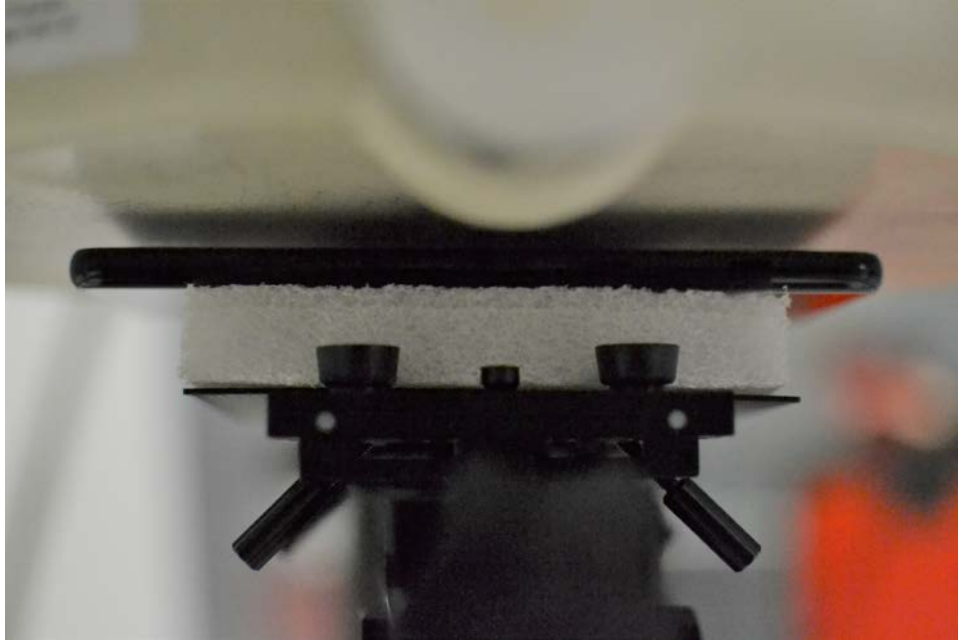
SAR Test Setup Photo 9: Front at 0.6 cm
