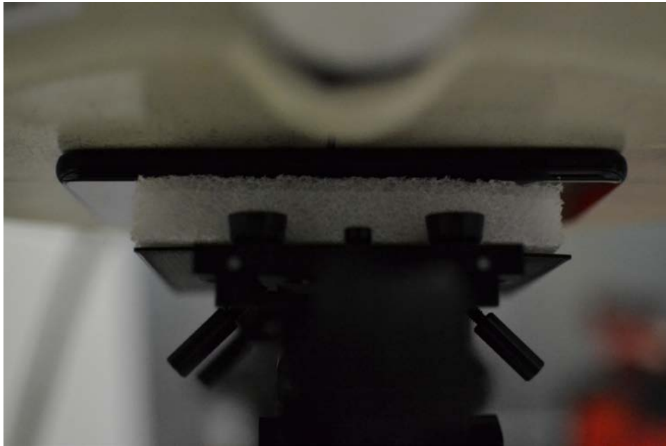
SAR Test Setup Photo 10: Front at 0.0 cm
