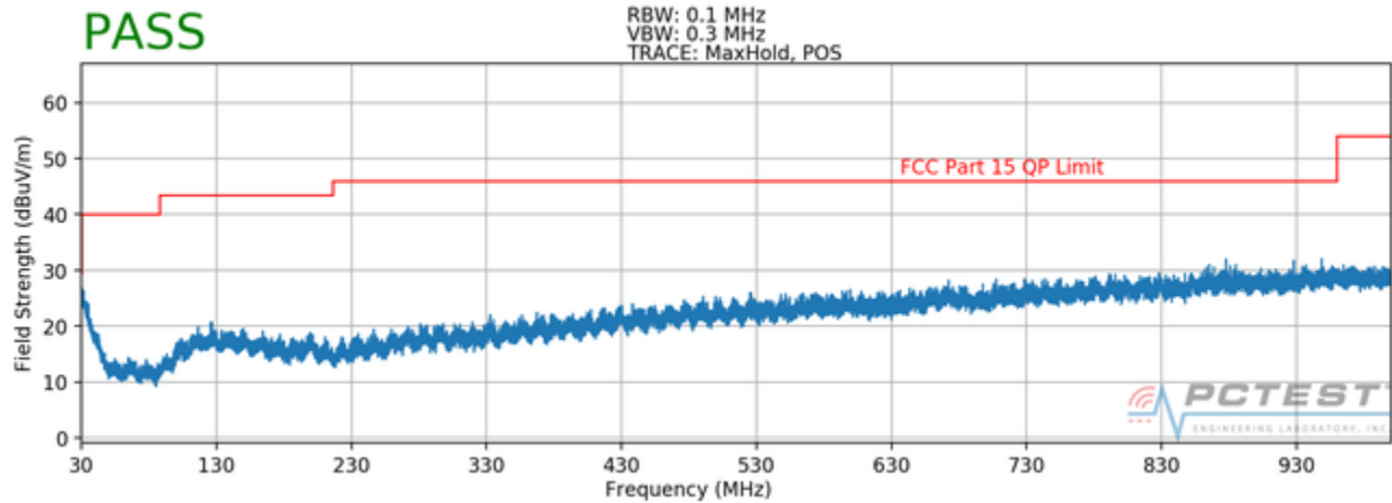
Plot 7-53. Radiated Spurious Plot below 1GHz (Pol. V)
