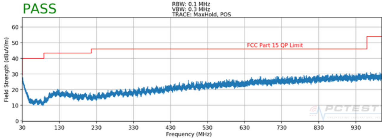
Plot 7-52. Radiated Spurious Plot below 1GHz (Pol. H)
