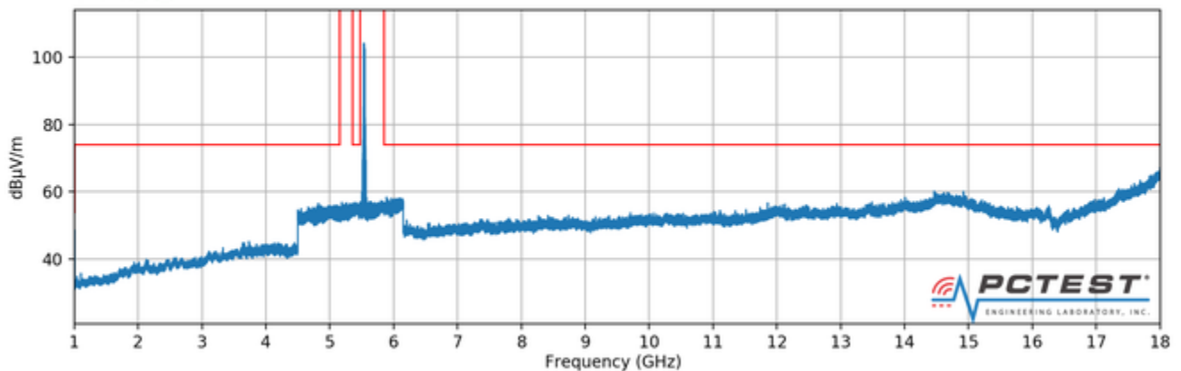
Plot 7-84. Radiated Spurious Plot above 1GHz (802.11a – U2C Ch. 120, Ant. Pol. V)
