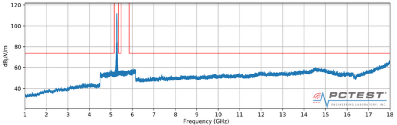
Plot 7-81. Radiated Spurious Plot above 1GHz (802.11a – U2A Ch. 56, Ant. Pol. H)
