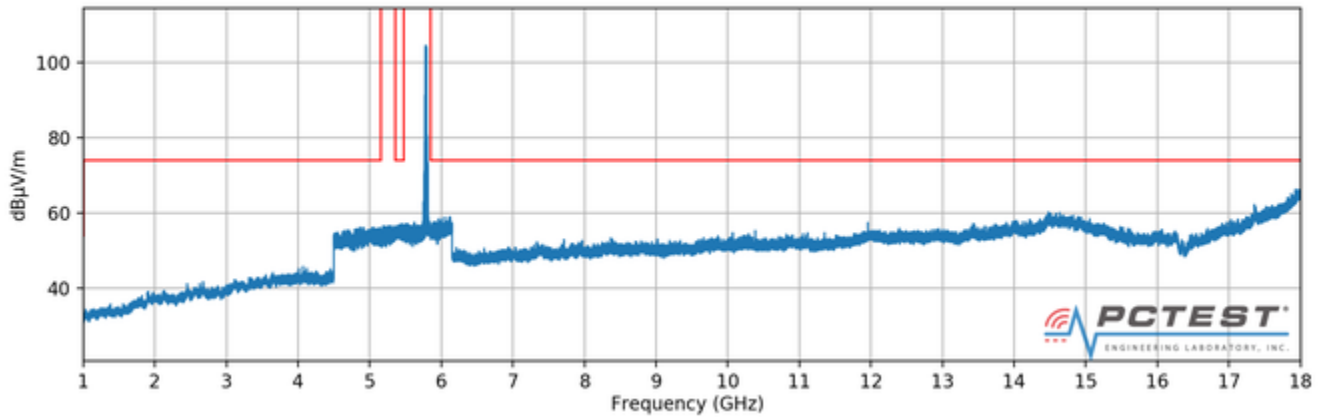
Plot 7-86. Radiated Spurious Plot above 1GHz (802.11a – U3 Ch. 157, Ant. Pol. V)
