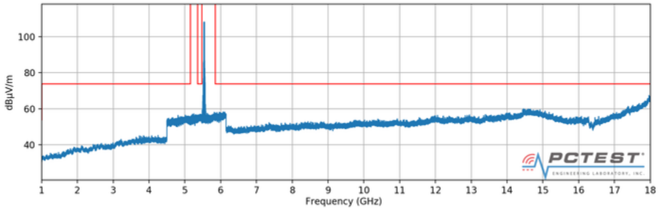
Plot 7-83. Radiated Spurious Plot above 1GHz (802.11a – U2C Ch. 120, Ant. Pol. H)
