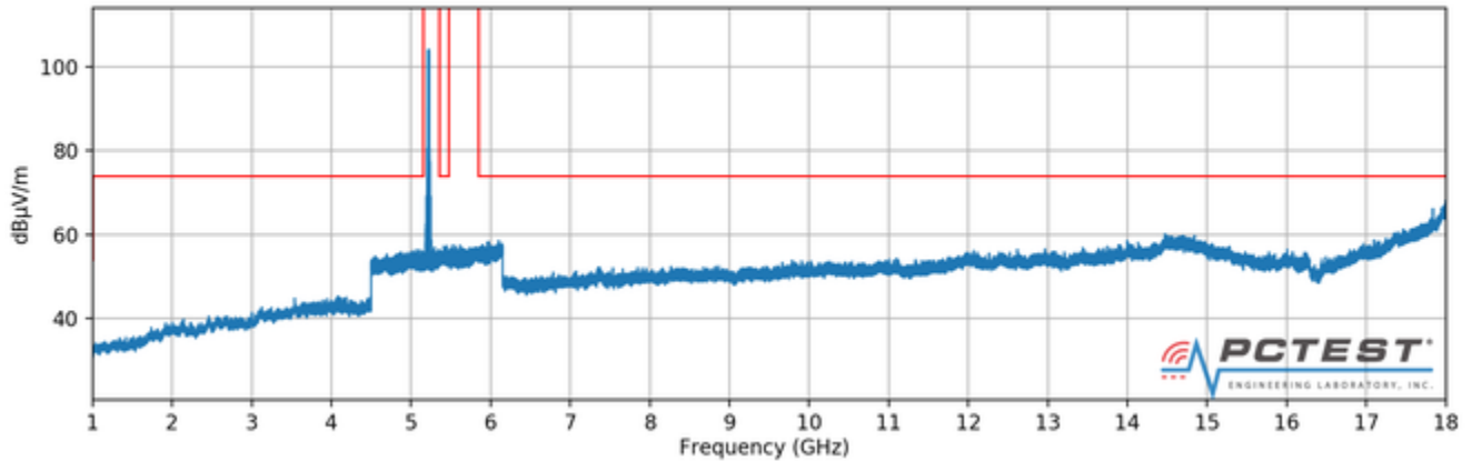
Plot 7-80. Radiated Spurious Plot above 1GHz (802.11a – U1 Ch. 40, Ant. Pol. V)
