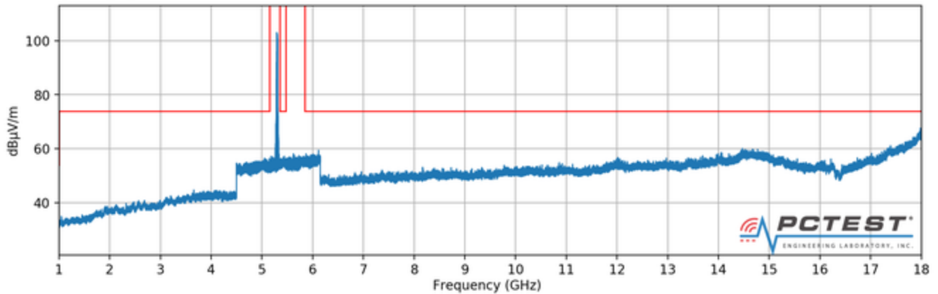
Plot 7-82. Radiated Spurious Plot above 1GHz (802.11a – U2A Ch. 56, Ant. Pol. V)
