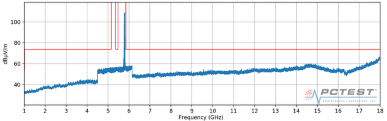
Plot 7-85. Radiated Spurious Plot above 1GHz (802.11a – U3 Ch. 157, Ant. Pol. H)
