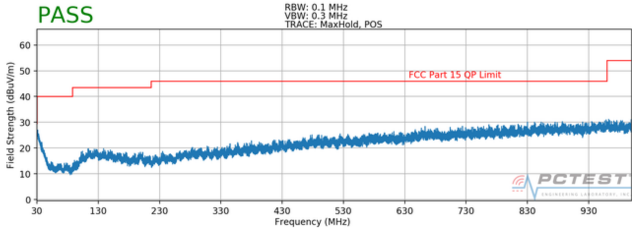
Plot 7-106. Radiated Spurious Plot below 1GHz (802.11a – U3 Ch. 157, Ant. Pol. H)
