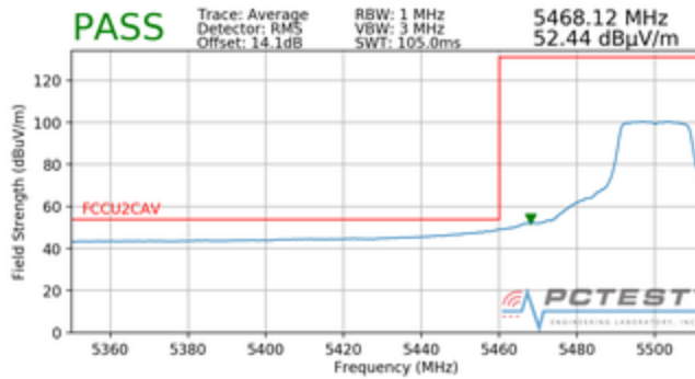
Plot 7-94. Radiated Lower Band Edge Plot (Average – UNII Band 2C)
