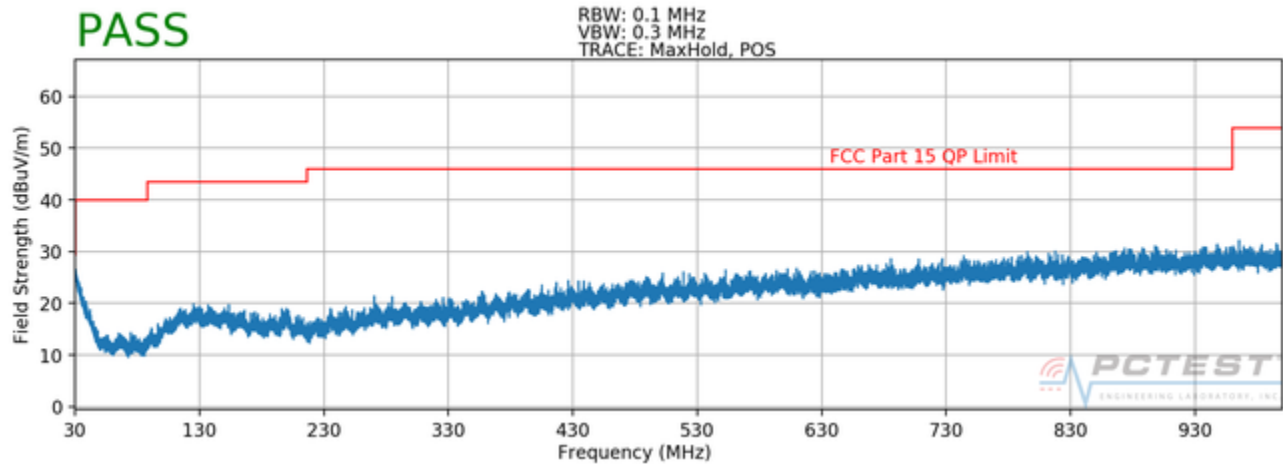
Plot 7-107. Radiated Spurious Plot below 1GHz (802.11a – U3 Ch. 157, Ant. Pol. V)
