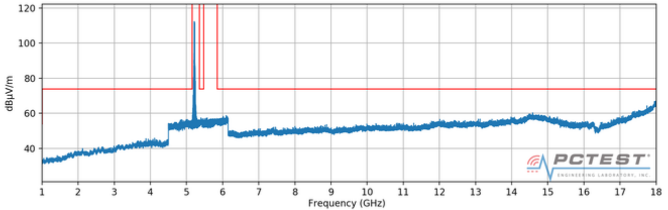
Plot 7-79. Radiated Spurious Plot above 1GHz (802.11a – U1 Ch. 40, Ant. Pol. H)
