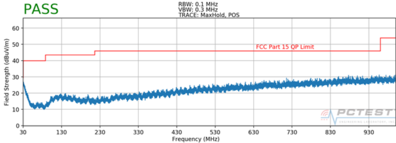
Plot 7-55. Radiated Spurious Plot below 1GHz (Pol. H)
