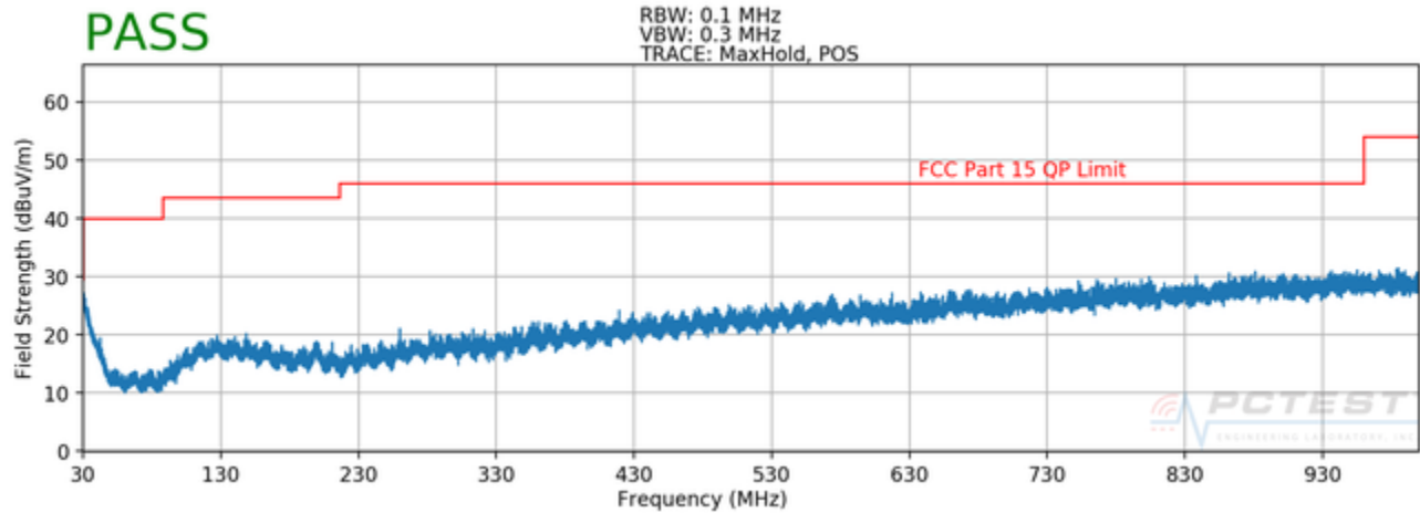
Plot 7-56. Radiated Spurious Plot below 1GHz (Pol. V)
