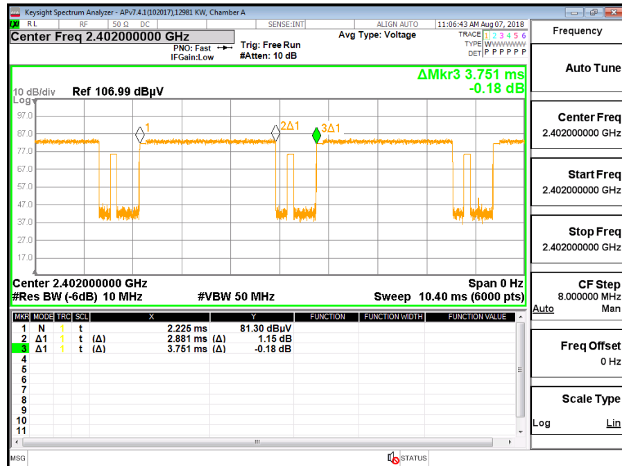
BLUETOOTH 8PSK
