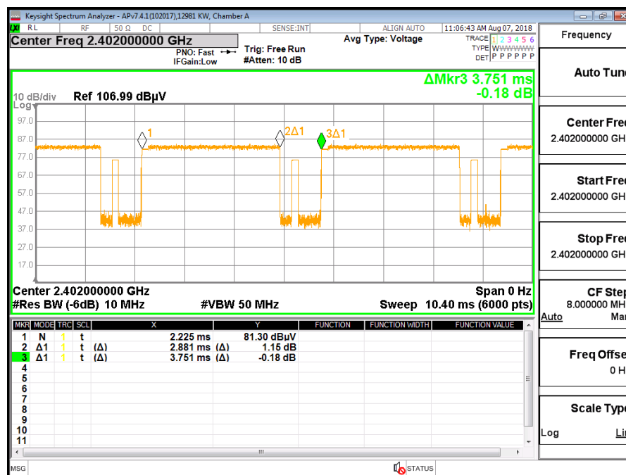
BLUETOOTH 8PSK
