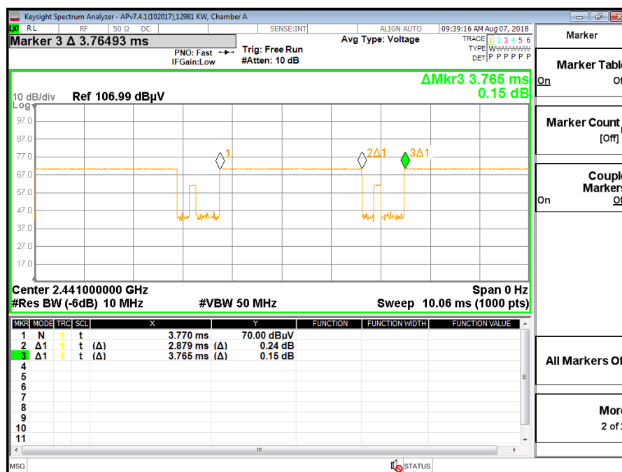
BLUETOOTH GFSK
