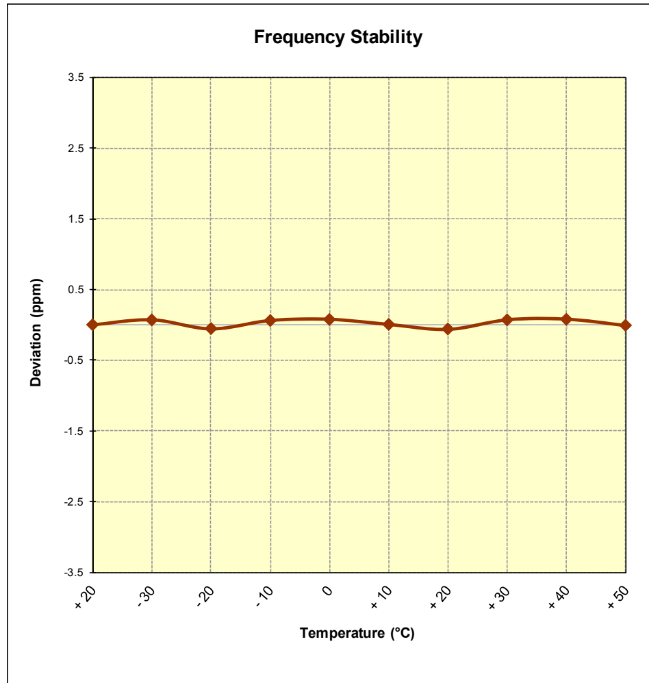
Figure 6-10. Frequency Stability Graph (PCS WCDMA Mode – Ch. 9400)
