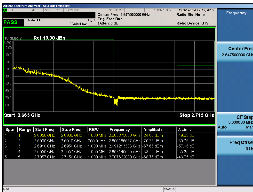
Plot 6-23. Upper ACP Plot (Band 41 – 15.0MHz QPSK – RB Size 75)
