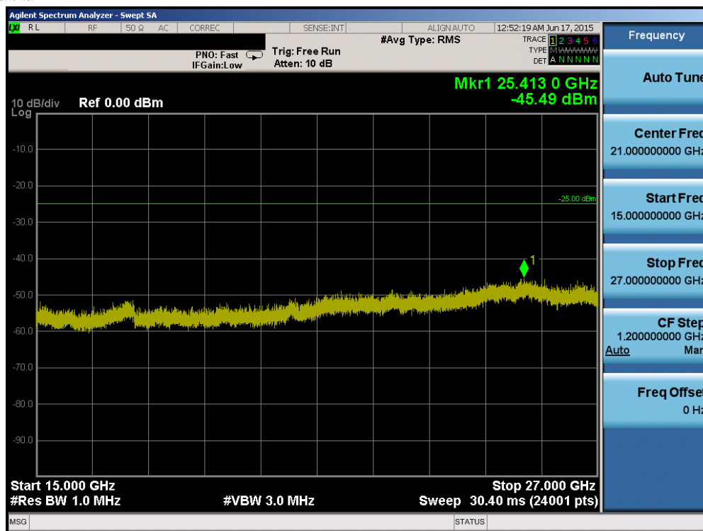
Plot 6-11. Conducted Spurious Plot (Band 41 – 20.0MHz QPSK – RB Size 1, RB Offset 0 – Low Channel)
