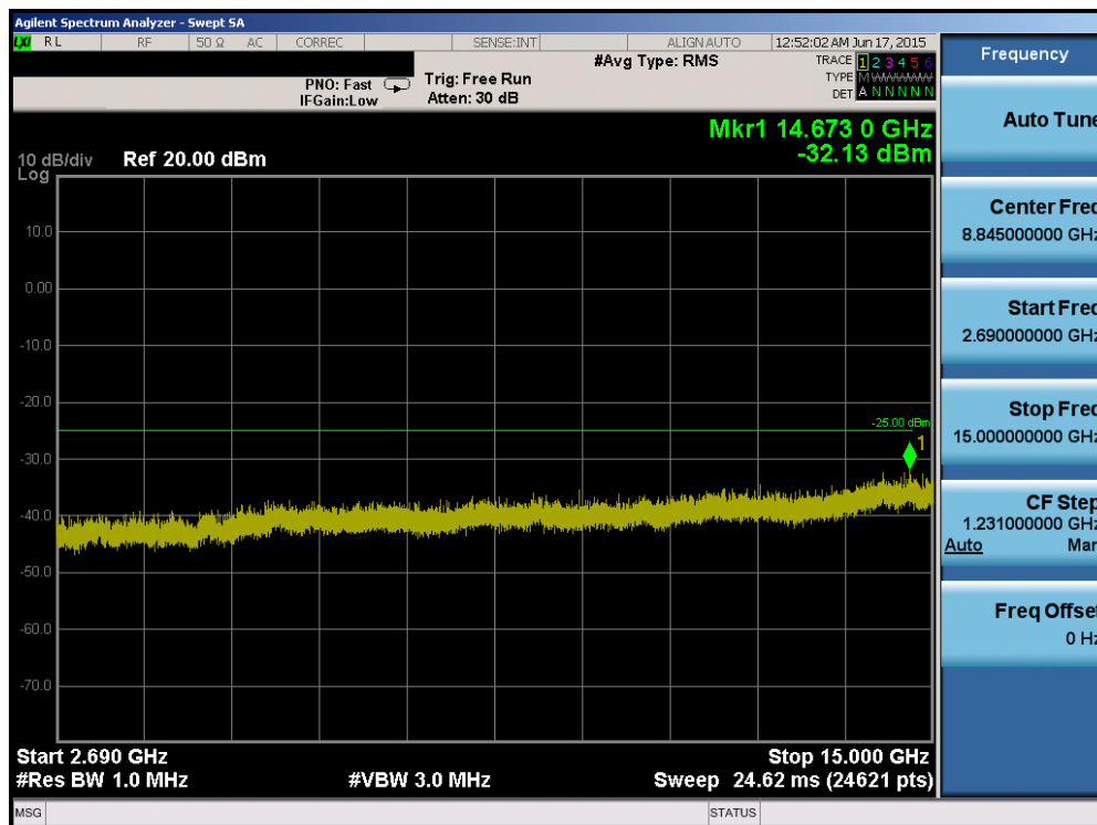
Plot 6-10. Conducted Spurious Plot (Band 41 – 20.0MHz QPSK – RB Size 1, RB Offset 0 – Low Channel)
