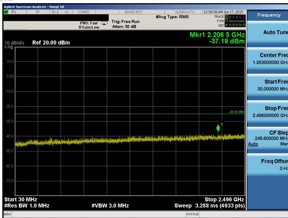
Plot 6-15. Conducted Spurious Plot (Band 41 – 20.0MHz QPSK – RB Size 1, RB Offset 0 – High Channel)
