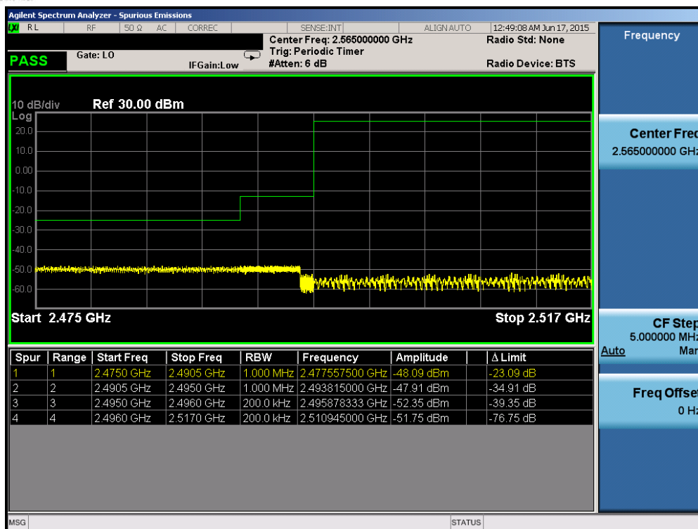
Plot 6-24. Lower ACP Plot (Band 41 – 20.0MHz QPSK – RB Size 100)
