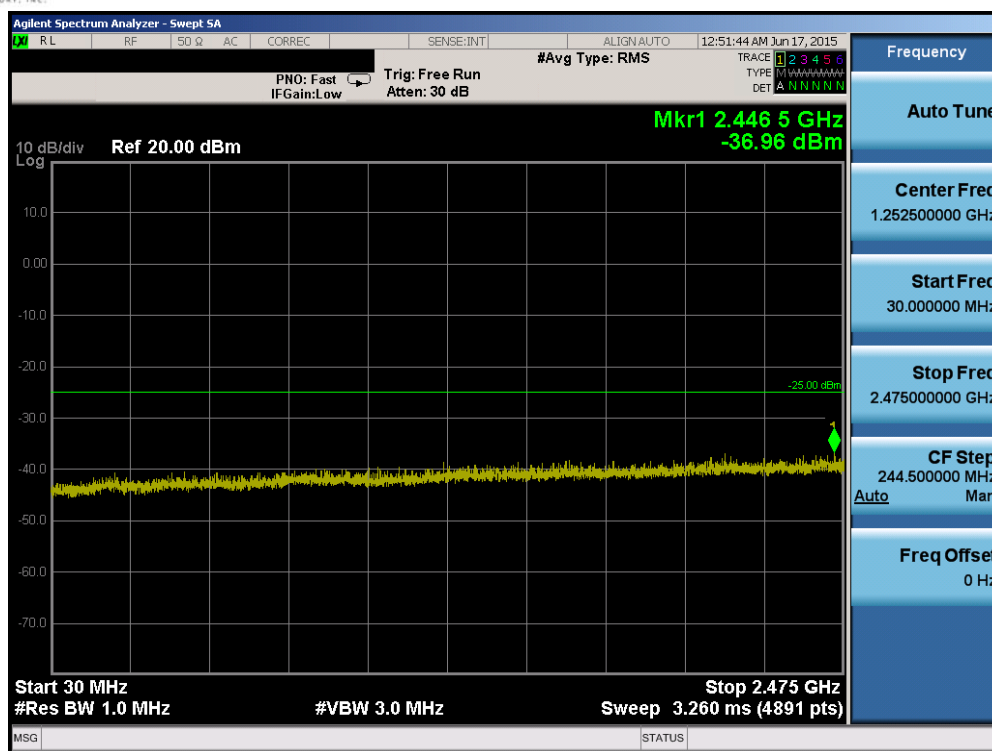
Plot 6-9. Conducted Spurious Plot (Band 41 – 20.0MHz QPSK – RB Size 1, RB Offset 0– Low Channel)
