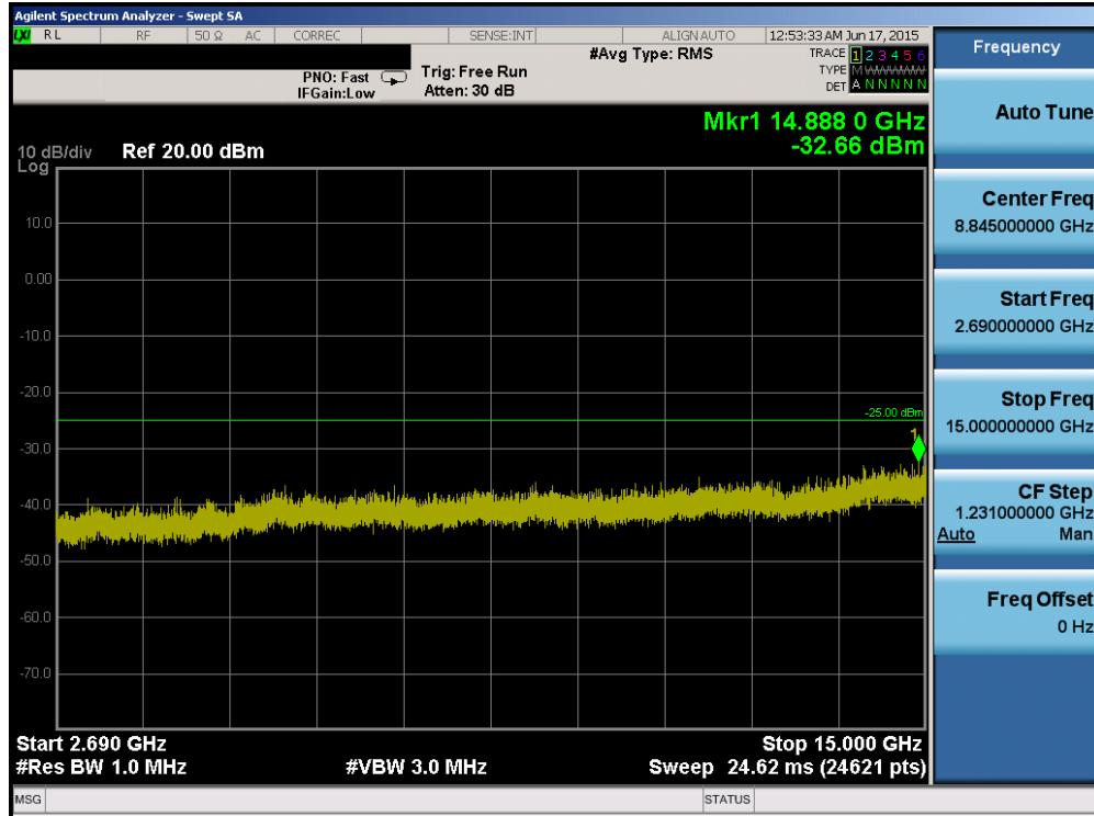
Plot 6-13. Conducted Spurious Plot (Band 41 – 20.0MHz QPSK – RB Size 1, RB Offset 0 – Mid Channel)
