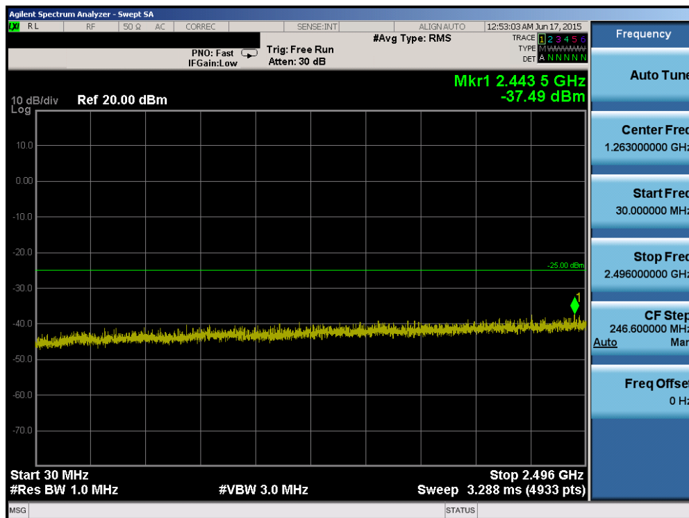
Plot 6-12. Conducted Spurious Plot (Band 41 – 20.0MHz QPSK – RB Size 1, RB Offset 0 – Mid Channel)
