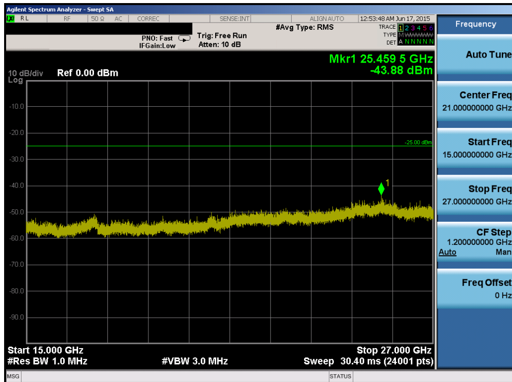
Plot 6-14. Conducted Spurious Plot (Band 41 – 20.0MHz QPSK – RB Size 1, RB Offset 0 – Mid Channel)
