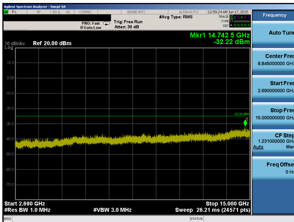
Plot 6-16. Conducted Spurious Plot (Band 41 – 20.0MHz QPSK – RB Size 1, RB Offset 0 – High Channel)
