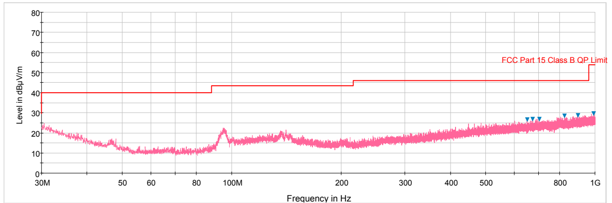
Plot 6-91. Radiated Spurious Plot below 1GHz (802.11a – U3 Ch. 157, Ant. Pol. H)
