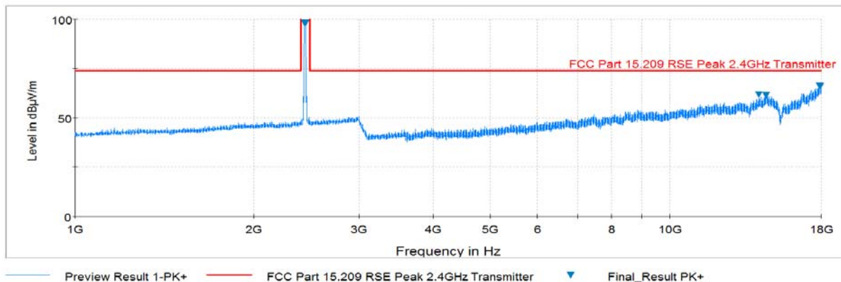
Plot 6-33. Radiated Spurious Plot above 1GHz (802.11b – Ch. 6, Ant. Pol. H)
