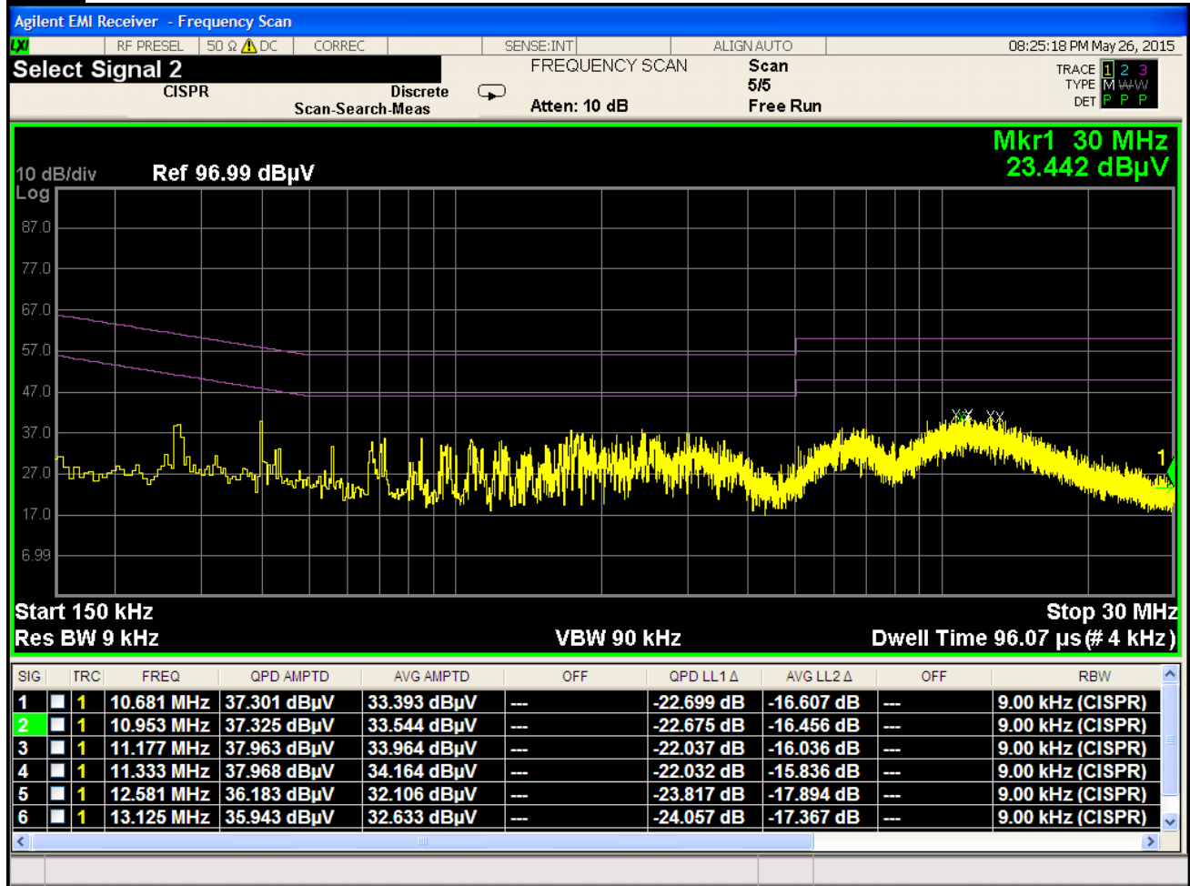
Plot 6-46. Line Conducted Plot with 802.11b (N)
