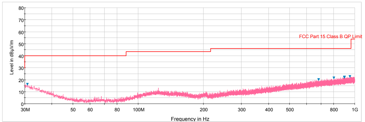
Plot 6-44. Radiated Spurious Plot below 1GHz (Pol. V)
