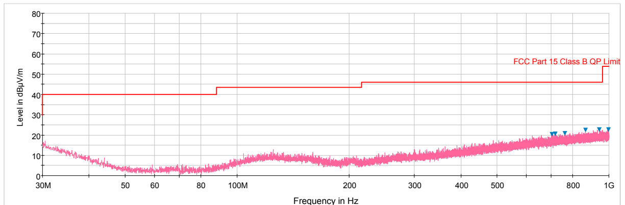
Plot 6-43. Radiated Spurious Plot below 1GHz (Pol. H)
