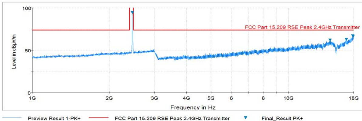
Plot 6-36. Radiated Spurious Plot above 1GHz (802.11b – Ch. 11, Ant. Pol. V)
