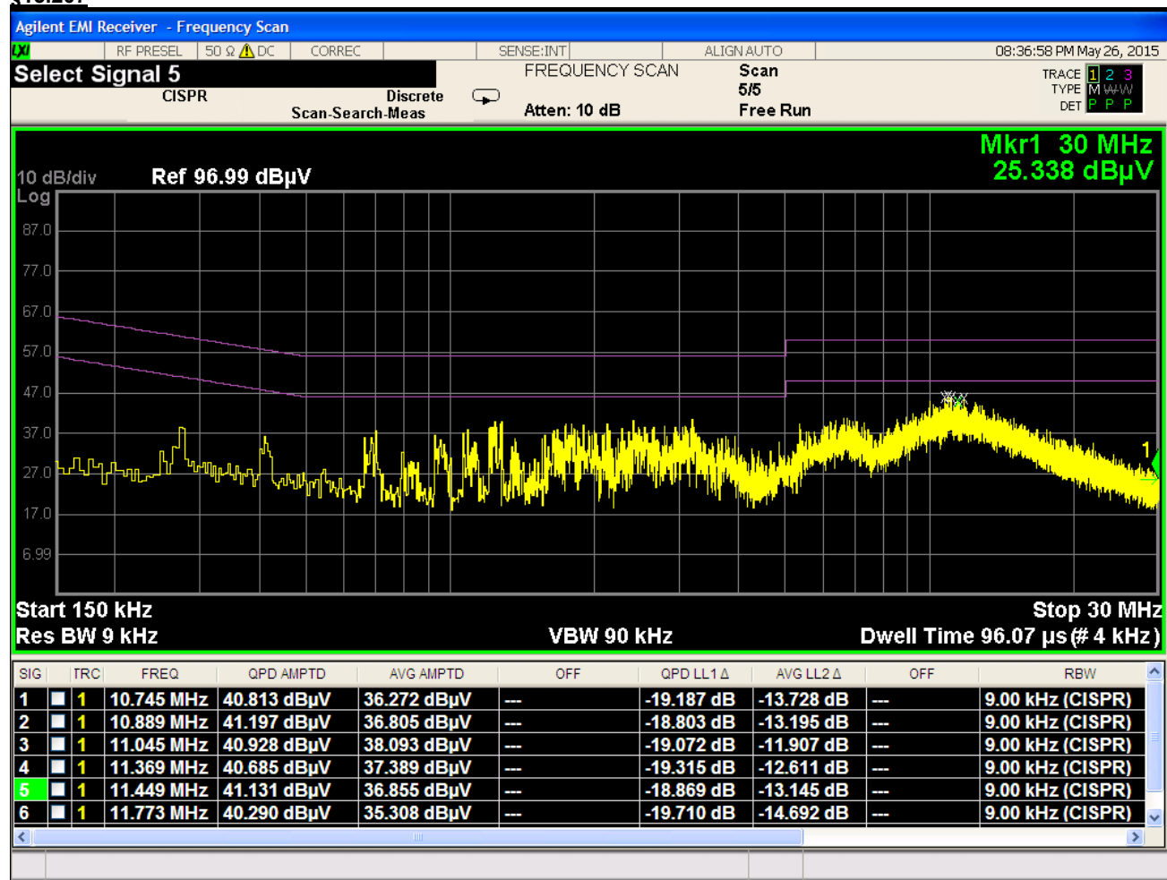
Plot 6-45. Line Conducted Plot with 802.11b (L1)
