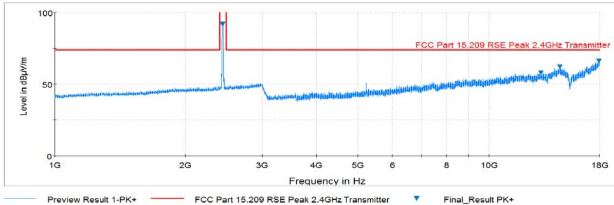
Plot 6-34. Radiated Spurious Plot above 1GHz (802.11b – Ch. 6, Ant. Pol. V)
