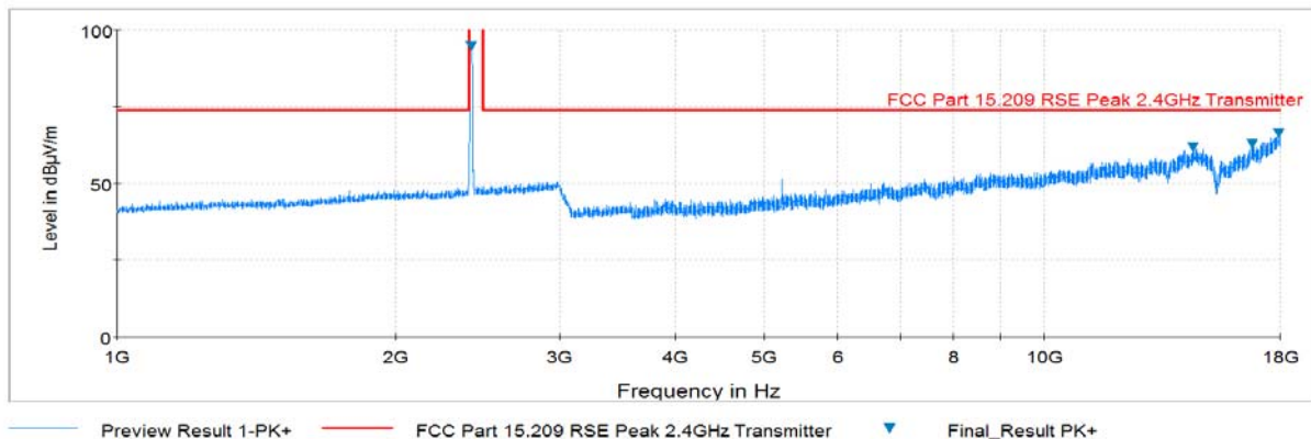
Plot 6-32. Radiated Spurious Plot above 1GHz (802.11b – Ch. 1, Ant. Pol. V)
