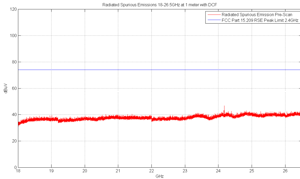
Plot 6-38. Radiated Spurious Plot above 18GHz (Pol. V)
