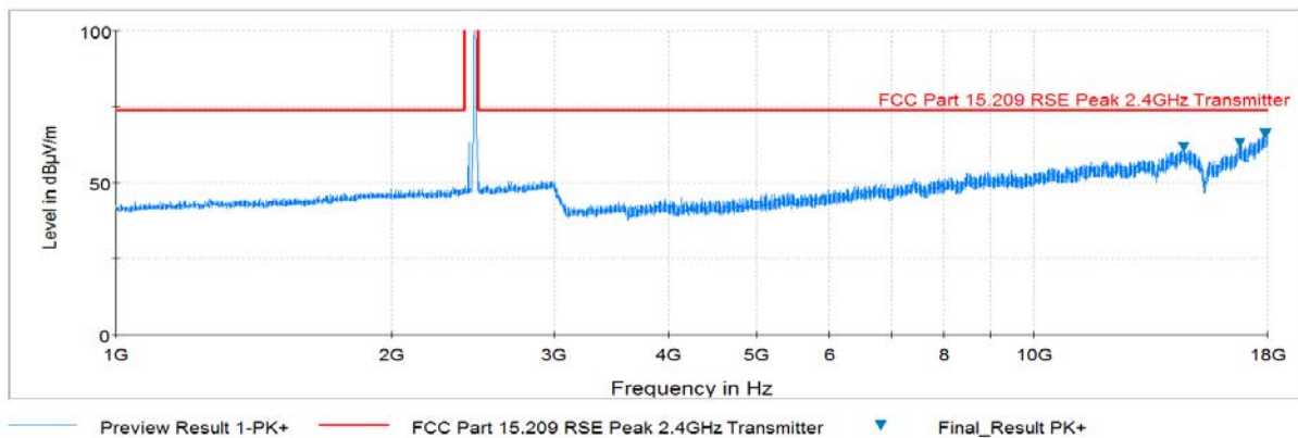
Plot 6-35. Radiated Spurious Plot above 1GHz (802.11b – Ch. 11, Ant. Pol. H)
