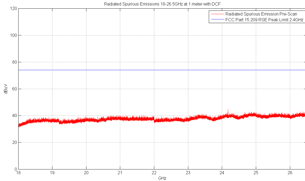
Plot 6-37. Radiated Spurious Plot above 18GHz (Pol. H)
