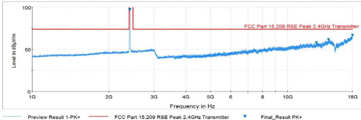
Plot 6-31. Radiated Spurious Plot above 1GHz (802.11b – Ch. 1, Ant. Pol. H)
