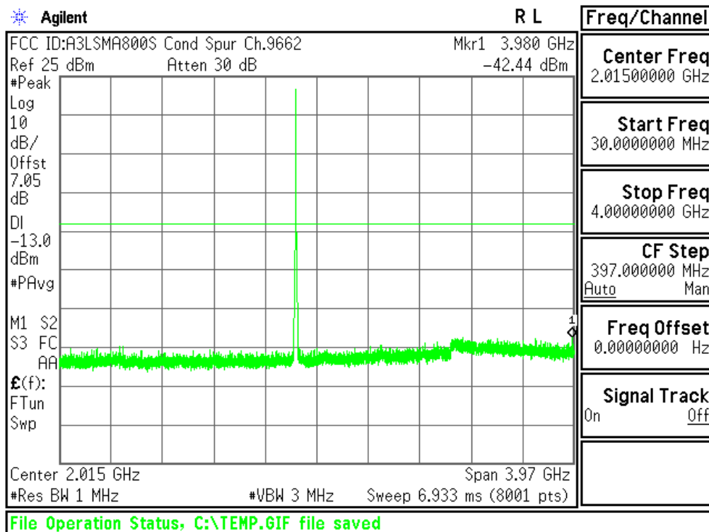
Plot 6-28. Conducted Spurious Plot (PCS WCDMA Mode - Ch.9262(DL9662))
