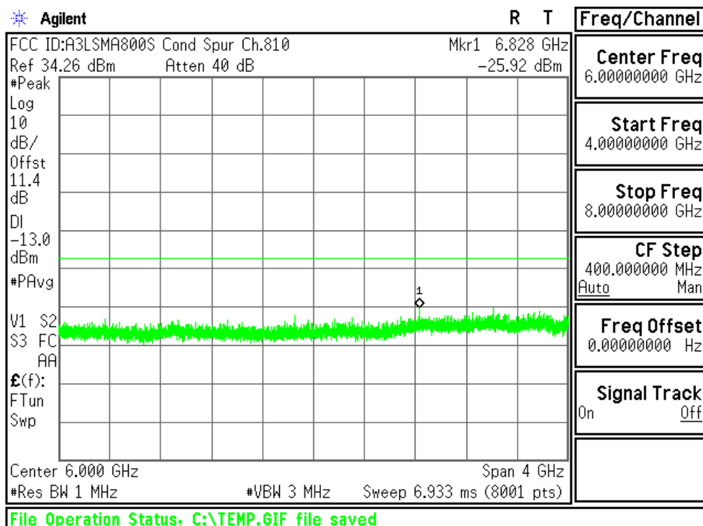
Plot 6-15. Conducted Spurious Plot (PCS GSM Mode - Ch.810)
