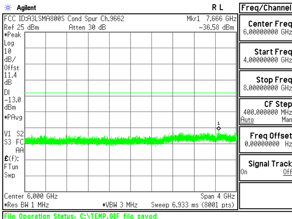
Plot 6-29. Conducted Spurious Plot (PCS WCDMA Mode - Ch.9262(DL9662))
