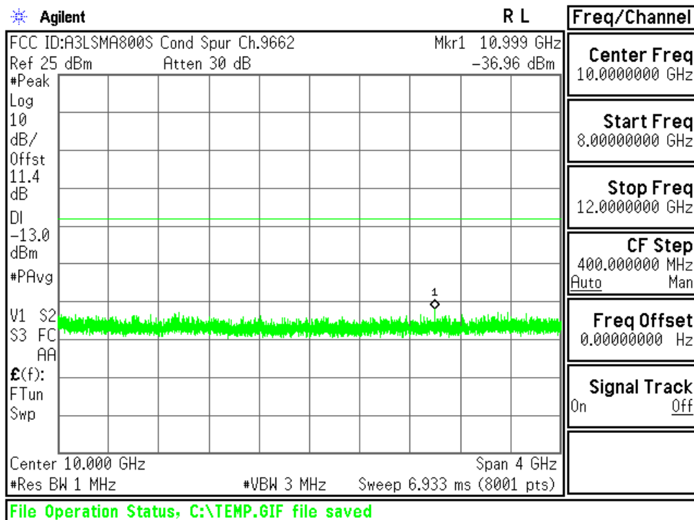
Plot 6-30. Conducted Spurious Plot (PCS WCDMA Mode - Ch.9262(DL9662))
