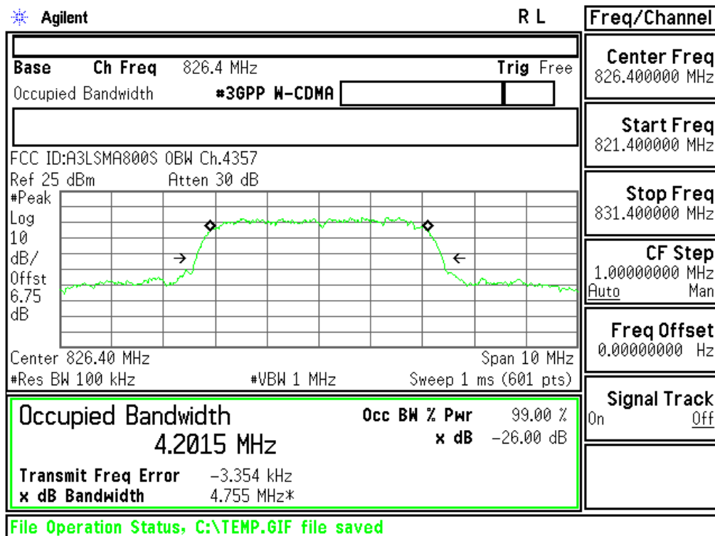
Plot 6-2. Occupied Bandwidth Plot (Cellular WCDMA Mode - Ch.4132(DL4357))
