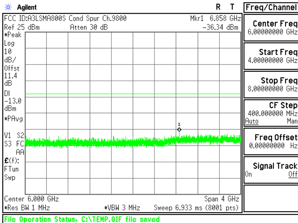
Plot 6-34. Conducted Spurious Plot (PCS WCDMA Mode - Ch.9400(DL9800))
