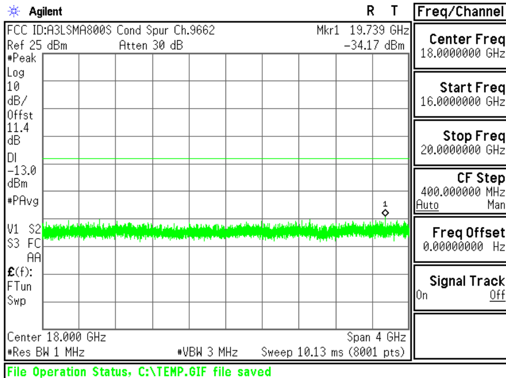
Plot 6-32. Conducted Spurious Plot (PCS WCDMA Mode - Ch.9262(DL9662))
