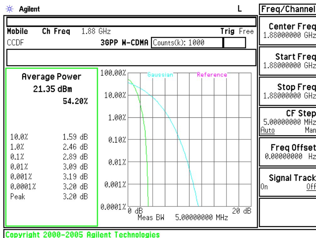
Plot 6-56. Peak-Average Ratio Plot (PCS WCDMA Mode - Ch.9400(DL9800))
