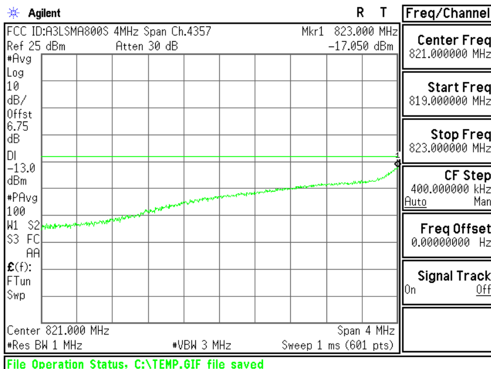
Plot 6-48. Extended Lower Band Edge Plot (Cellular WCDMA Mode - Ch.4132(DL4357))
