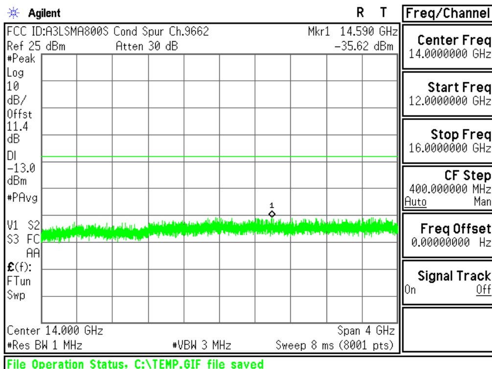
Plot 6-31. Conducted Spurious Plot (PCS WCDMA Mode - Ch.9262(DL9662))
