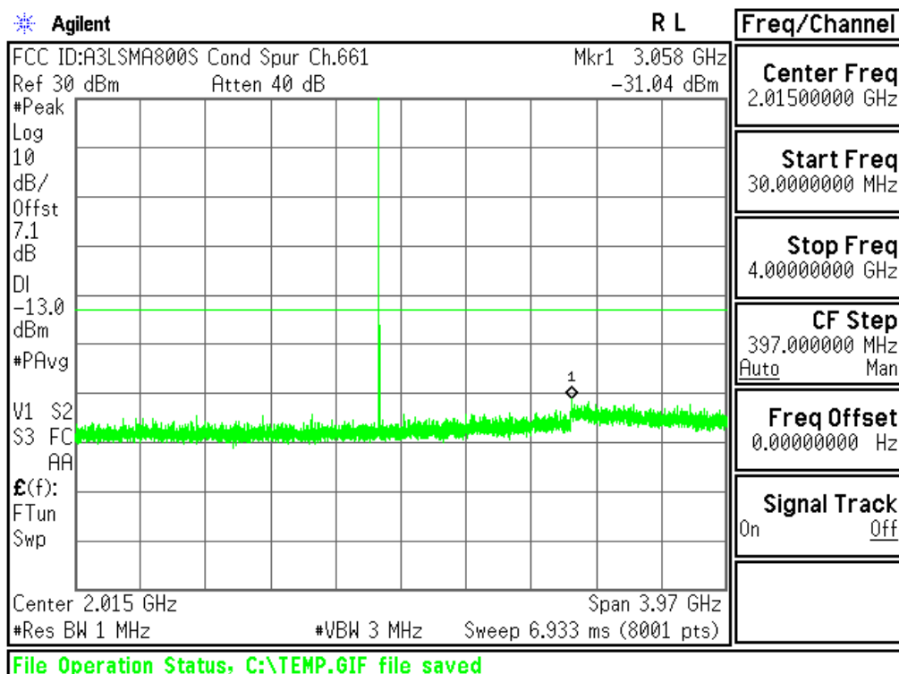
Plot 6-9. Conducted Spurious Plot (PCS GSM Mode - Ch.661)
