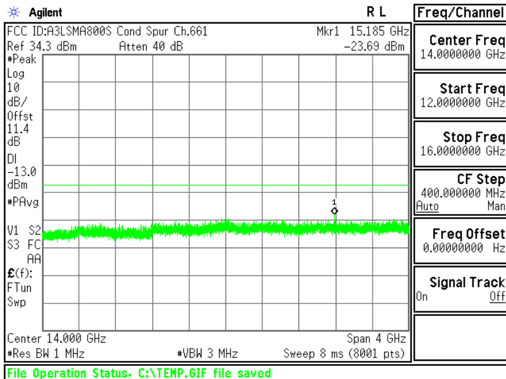
Plot 6-12. Conducted Spurious Plot (PCS GSM Mode - Ch.661)
