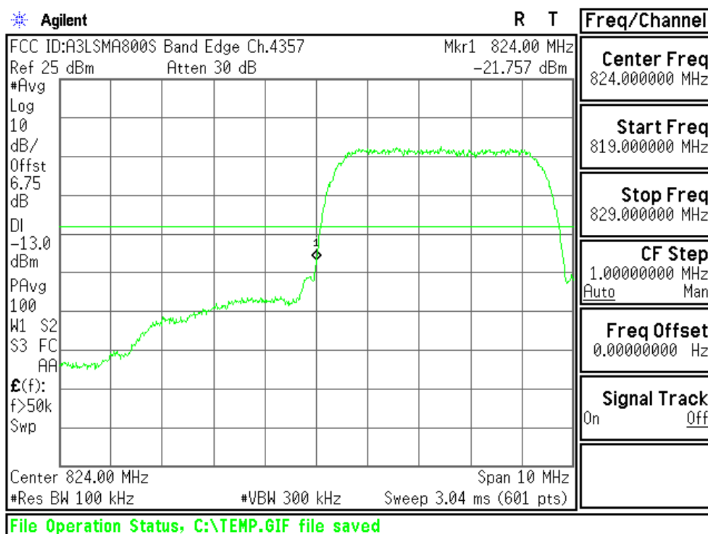
Plot 6-47. Lower Band Edge Plot (Cellular WCDMA Mode - Ch.4132(DL4357))
