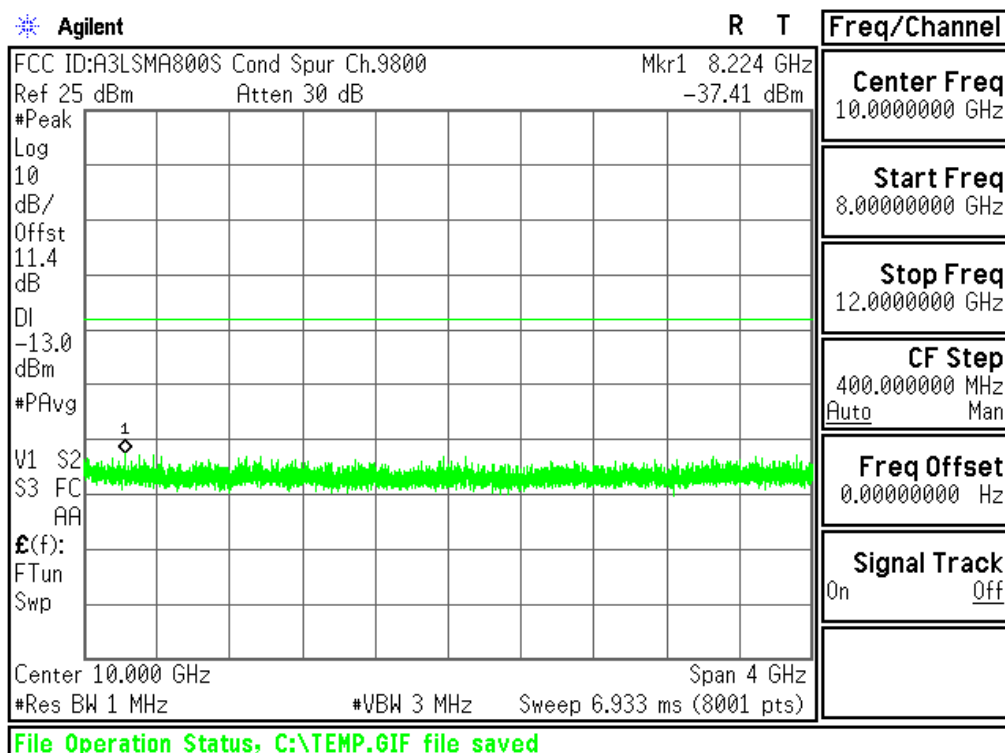
Plot 6-35. Conducted Spurious Plot (PCS WCDMA Mode - Ch.9400(DL9800))
