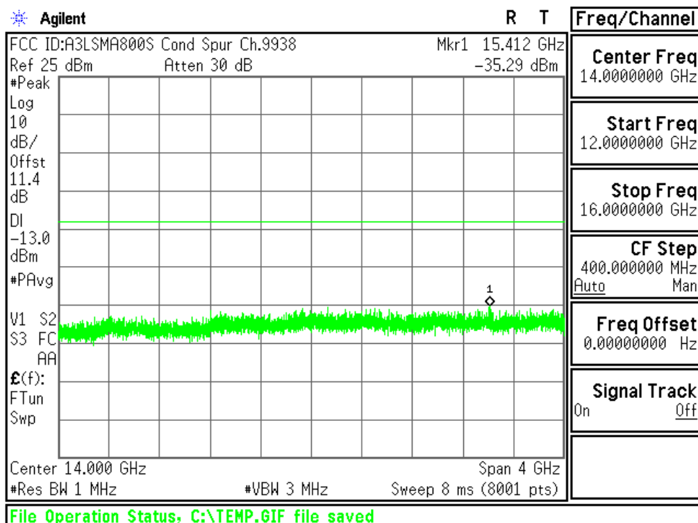
Plot 6-41. Conducted Spurious Plot (PCS WCDMA Mode - Ch.9538(DL9938))
