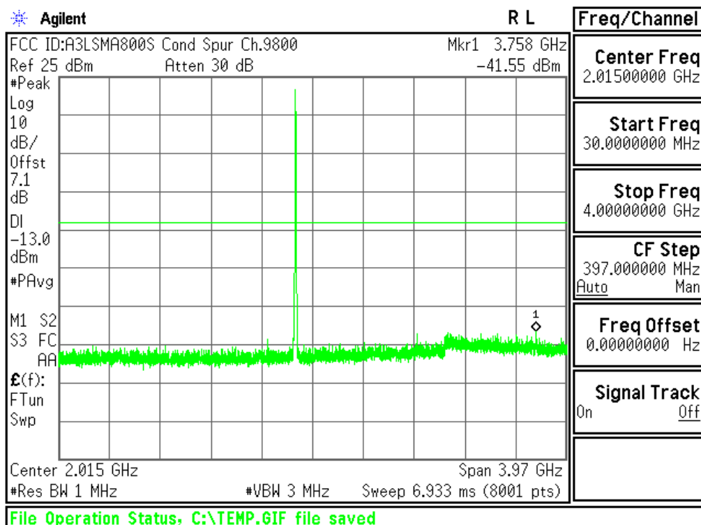
Plot 6-33. Conducted Spurious Plot (PCS WCDMA Mode - Ch.9400(DL9800))
