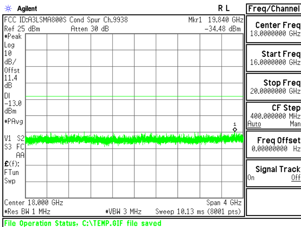
Plot 6-42. Conducted Spurious Plot (PCS WCDMA Mode - Ch.9538(DL9938))
