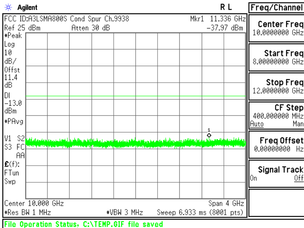
Plot 6-40. Conducted Spurious Plot (PCS WCDMA Mode - Ch.9538(DL9938))
