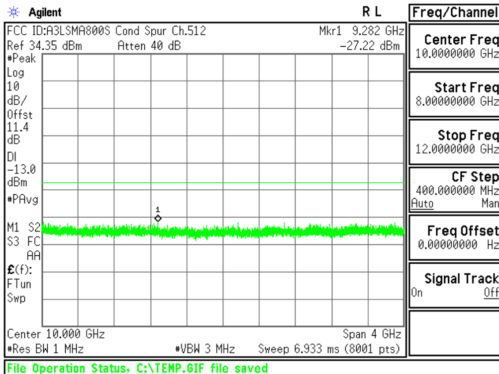
Plot 6-6. Conducted Spurious Plot (PCS GSM Mode - Ch.512)
