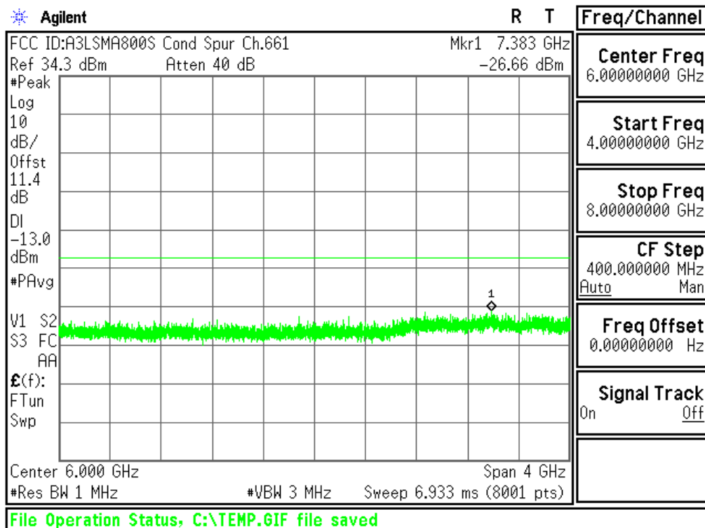
Plot 6-10. Conducted Spurious Plot (PCS GSM Mode - Ch.661)
