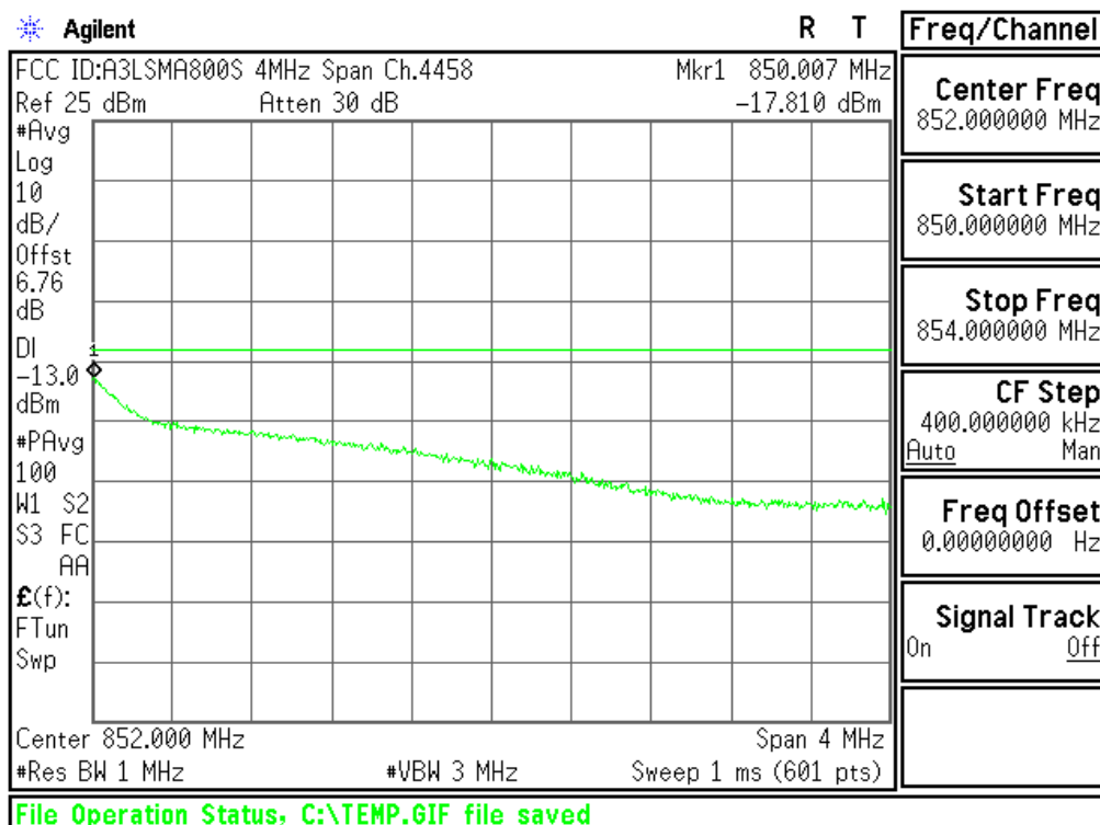
Plot 6-50. Extended Upper Band Edge Plot (Cellular WCDMA Mode - Ch.4233(DL4458))
