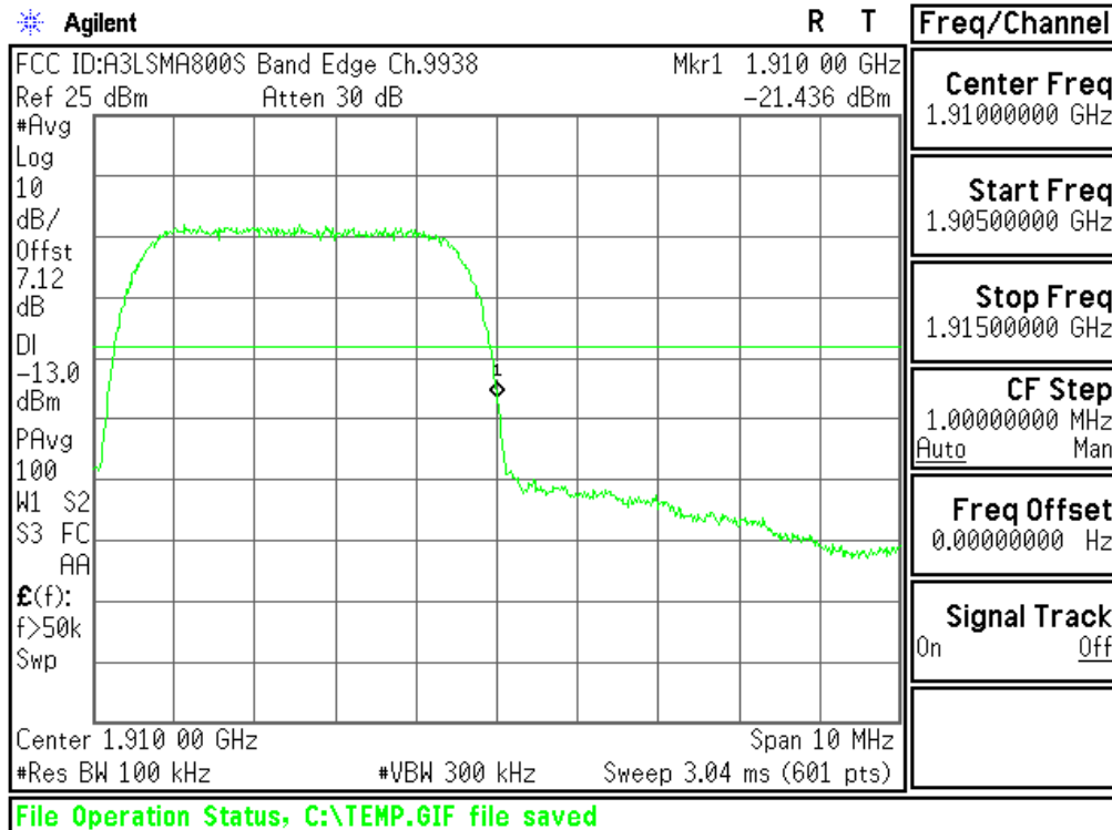
Plot 6-53. Upper Band Edge Plot (PCS WCDMA Mode - Ch.9538(DL9938))
