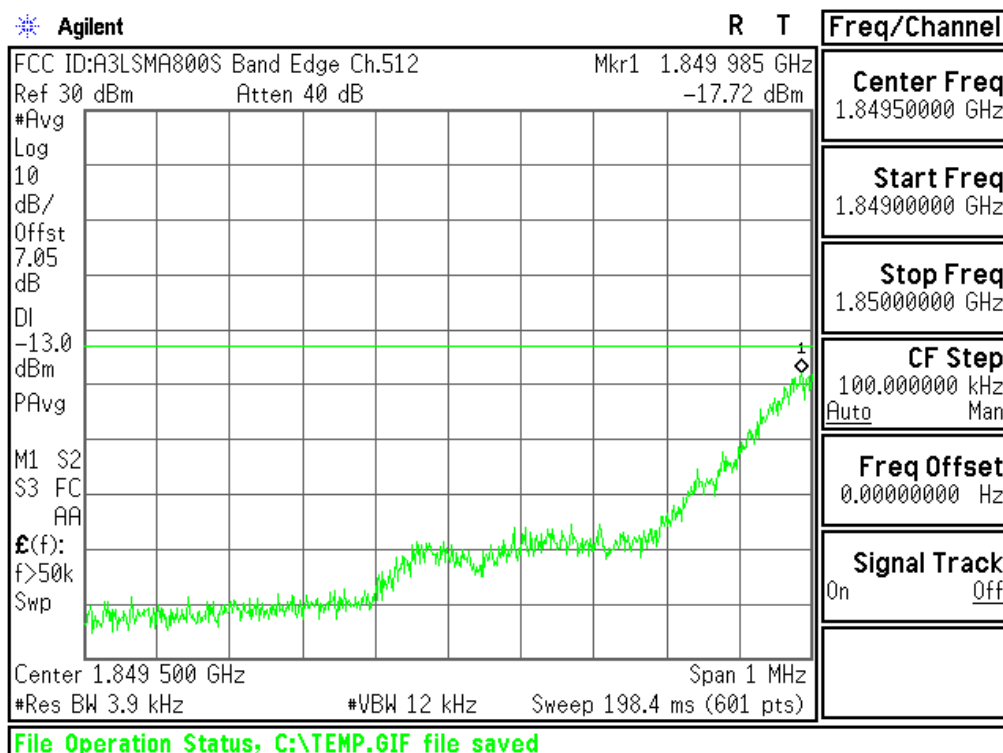
Plot 6-44. Lower Band Edge Plot (PCS GSM Mode – Ch.512)
