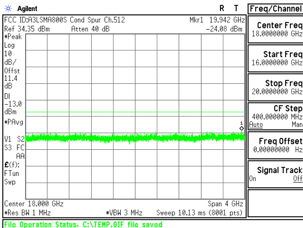
Plot 6-8. Conducted Spurious Plot (PCS GSM Mode - Ch.512)
