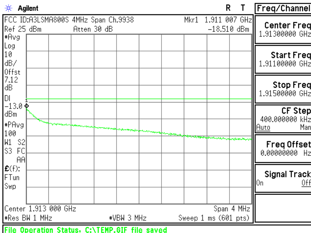
Plot 6-54. Extended Upper Band Edge Plot (PCS WCDMA Mode - Ch.9538(DL9938))
