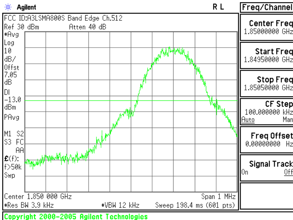
Plot 6-43. Lower Band Edge Plot (PCS GSM Mode – Ch.512)
