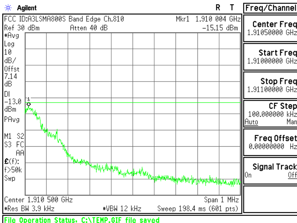
Plot 6-46. Upper Band Edge Plot (PCS GSM Mode – Ch.810)
