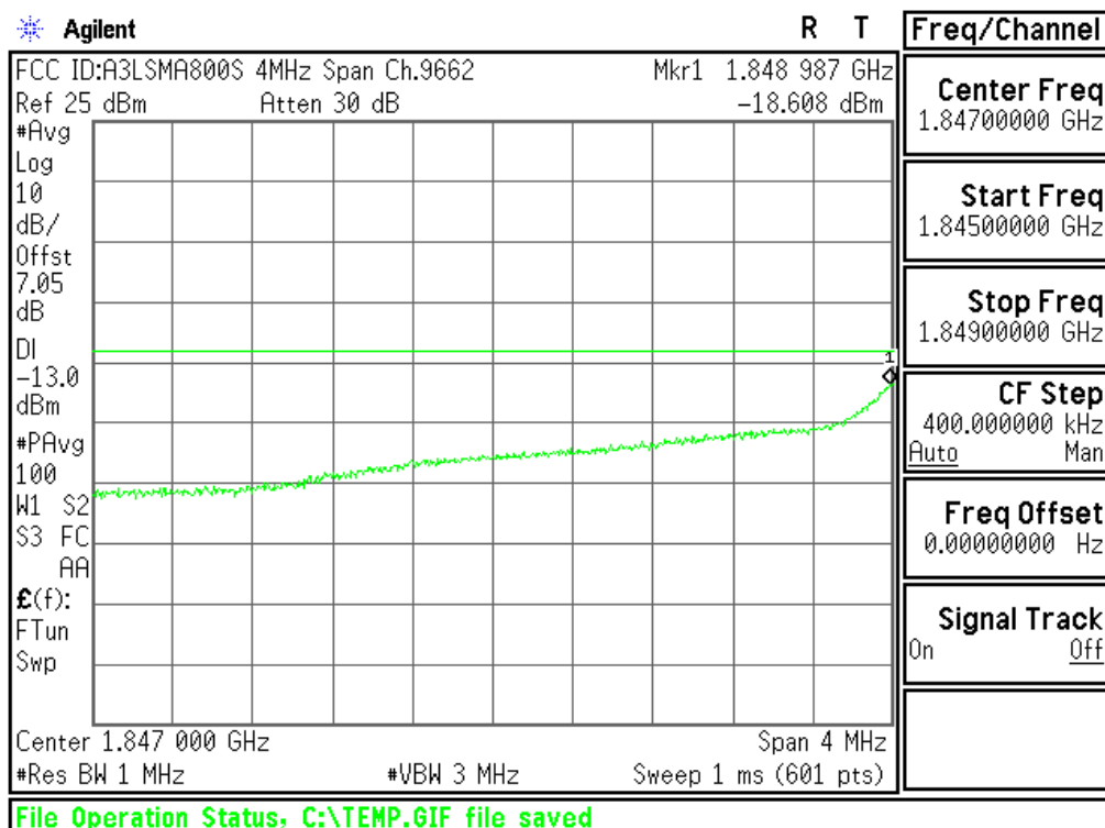
Plot 6-52. Extended Lower Band Edge Plot (PCS WCDMA Mode - Ch.9262(DL9662))
