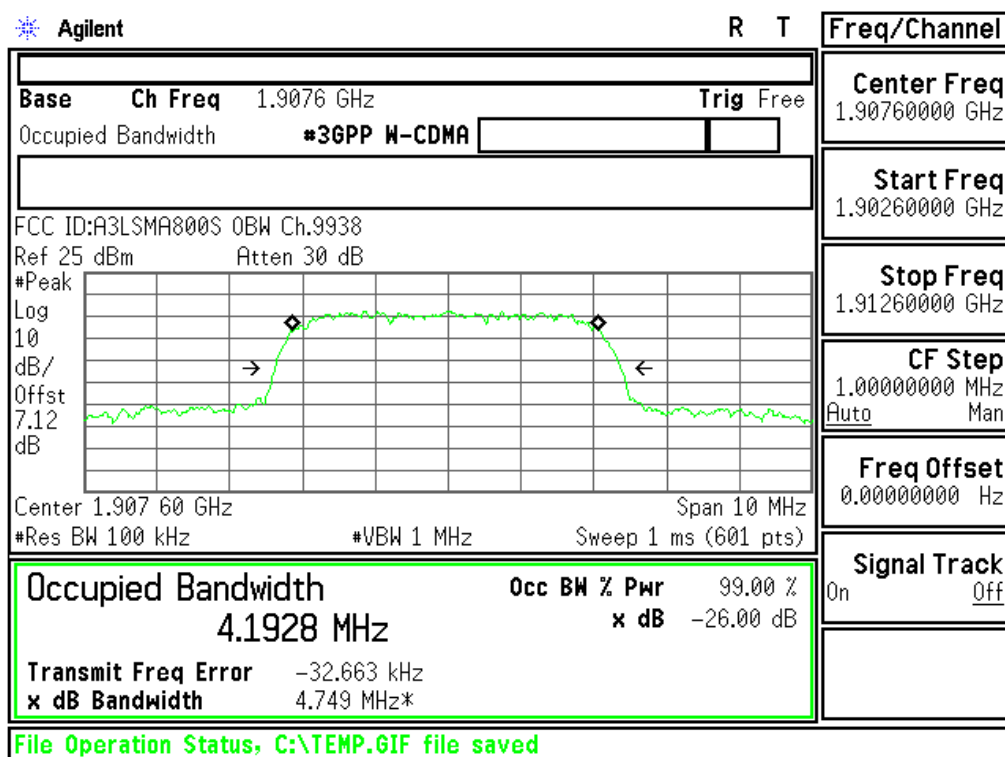
Plot 6-3. Occupied Bandwidth Plot (PCS WCDMA Mode - Ch.9538(DL9938))
