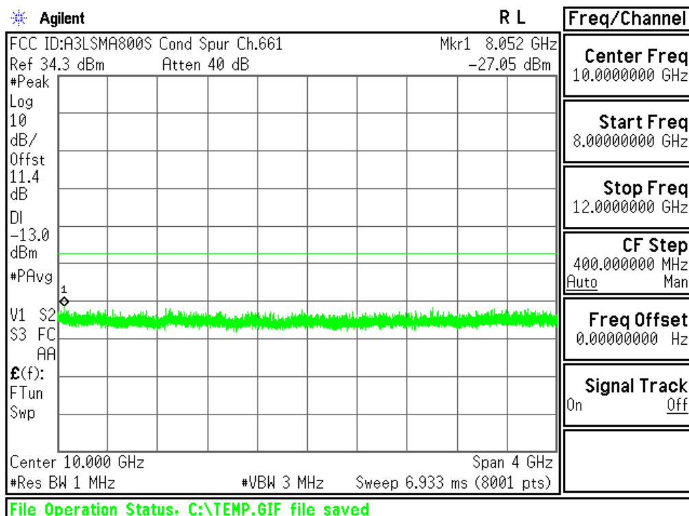
Plot 6-11. Conducted Spurious Plot (PCS GSM Mode - Ch.661)
