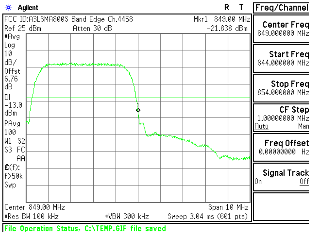
Plot 6-49. Upper Band Edge Plot (Cellular WCDMA Mode - Ch.4233(DL4458))
