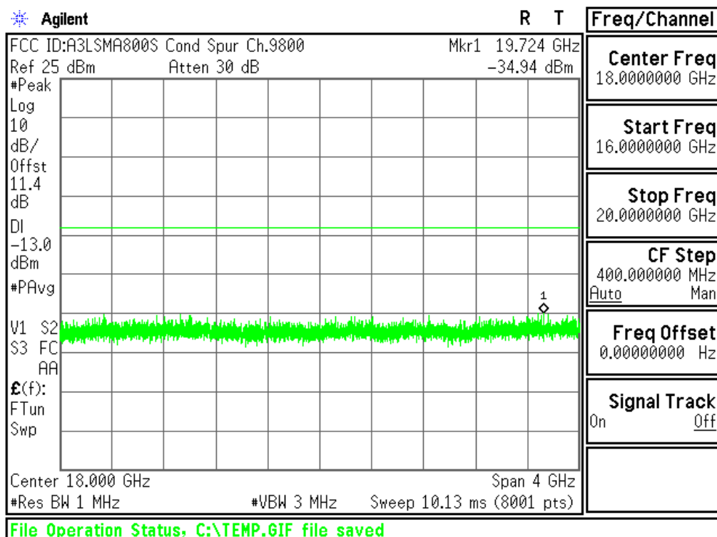
Plot 6-37. Conducted Spurious Plot (PCS WCDMA Mode - Ch.9400(DL9800))
