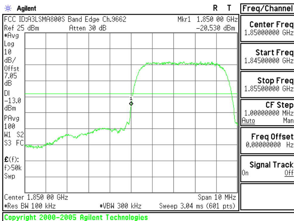
Plot 6-51. Lower Band Edge Plot (PCS WCDMA Mode - Ch.9262(DL9662))
