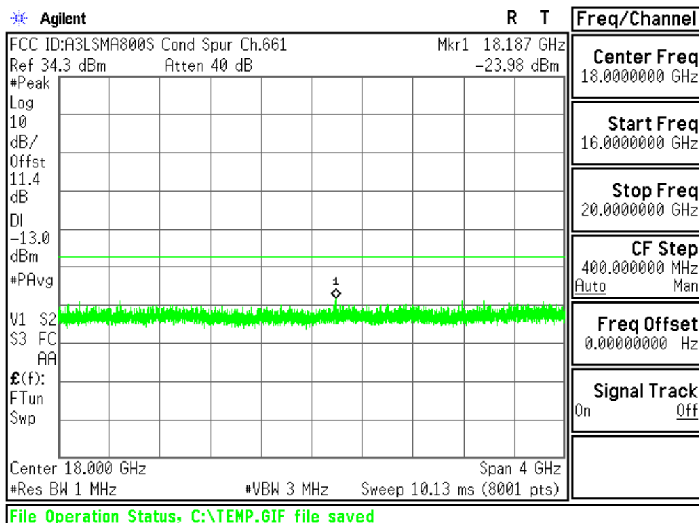
Plot 6-13. Conducted Spurious Plot (PCS GSM Mode - Ch.661)
