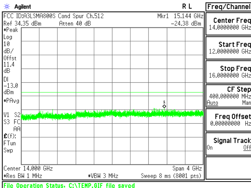
Plot 6-7. Conducted Spurious Plot (PCS GSM Mode - Ch.512)
