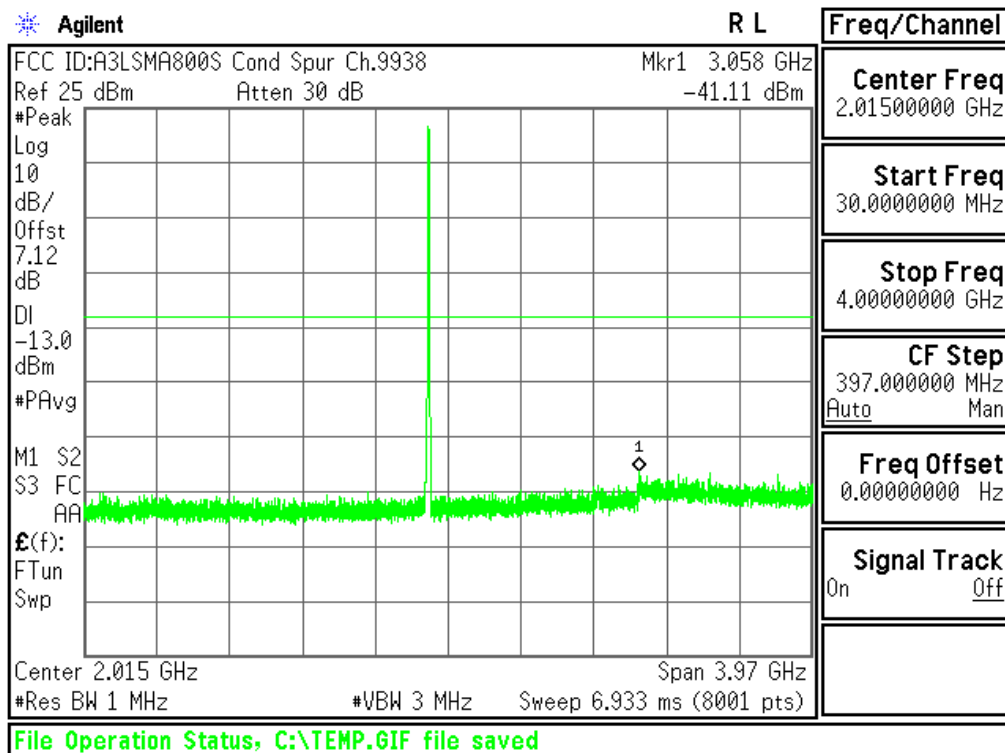
Plot 6-38. Conducted Spurious Plot (PCS WCDMA Mode - Ch.9538(DL9938))
