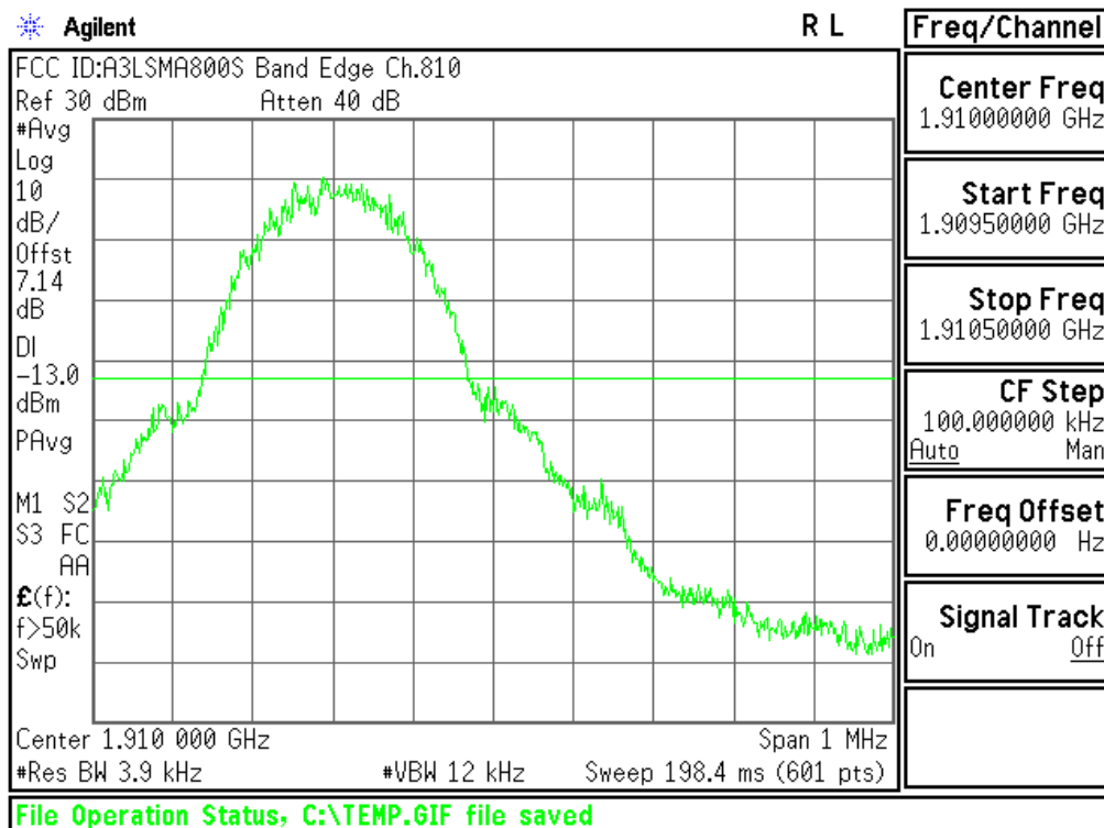
Plot 6-45. Upper Band Edge Plot (PCS GSM Mode – Ch.810)
