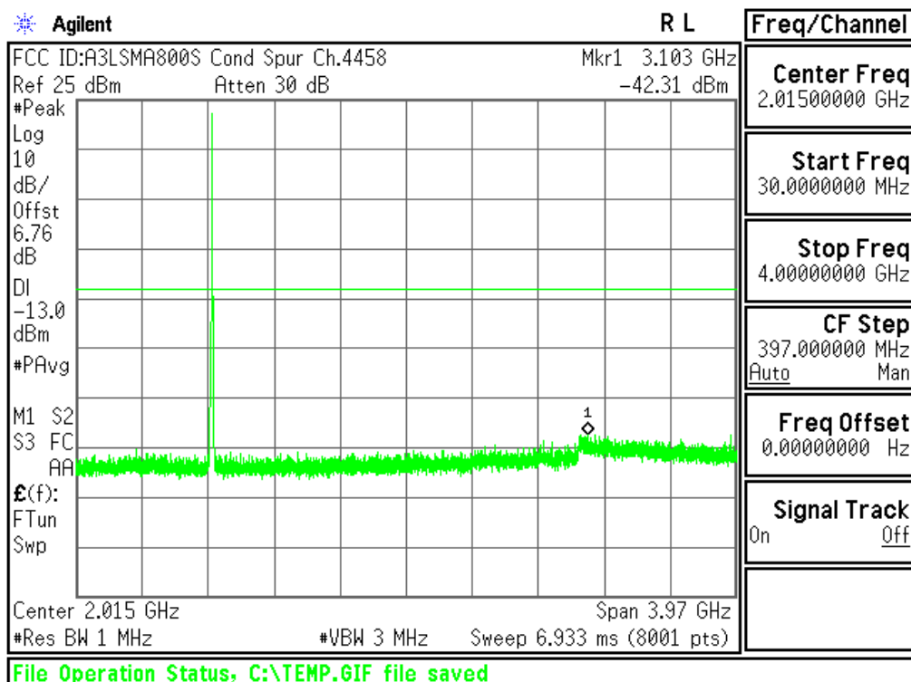
Plot 6-25. Conducted Spurious Plot (Cellular WCDMA Mode - Ch.4233(DL4458))
