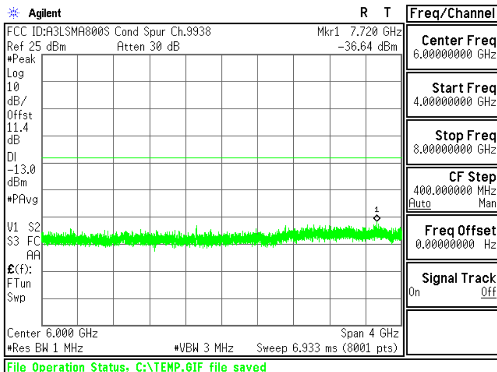
Plot 6-39. Conducted Spurious Plot (PCS WCDMA Mode - Ch.9538(DL9938))
