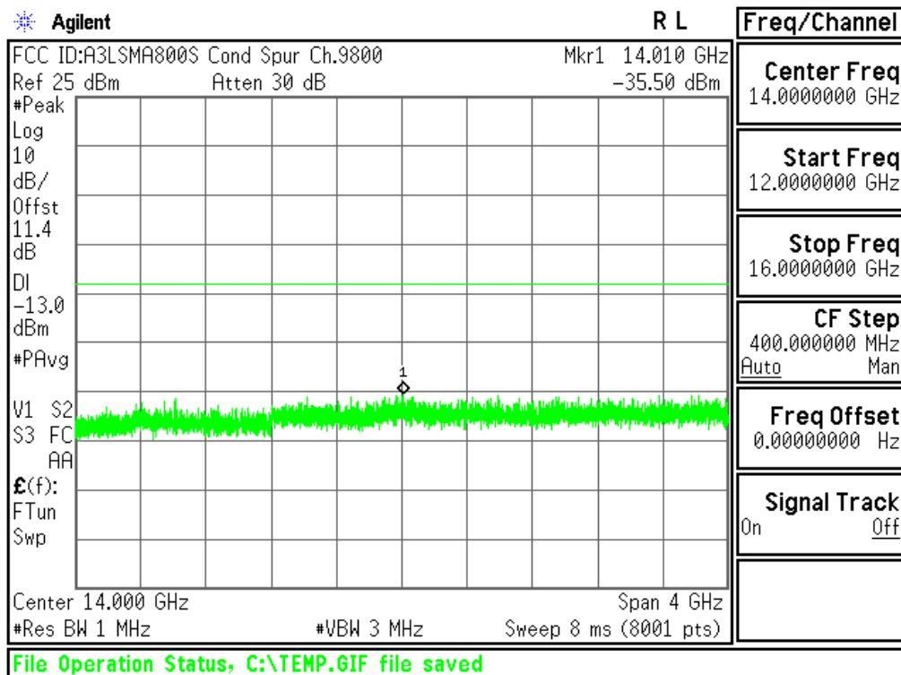
Plot 6-36. Conducted Spurious Plot (PCS WCDMA Mode - Ch.9400(DL9800))
