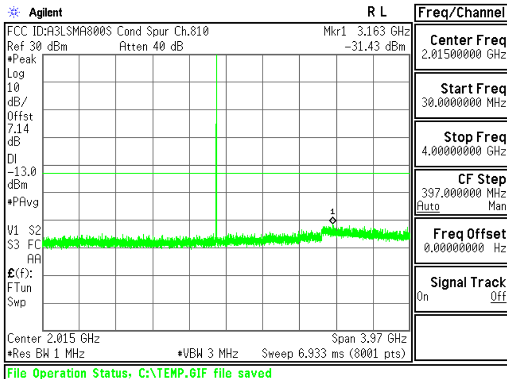
Plot 6-14. Conducted Spurious Plot (PCS GSM Mode - Ch.810)
